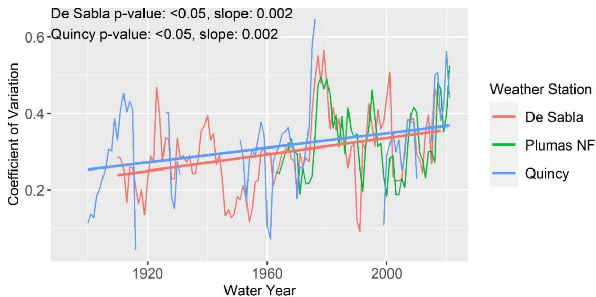
Figure 4. Coefficient of variation in precipitation for local Plumas National Forest weather stations (identified in different colors).
