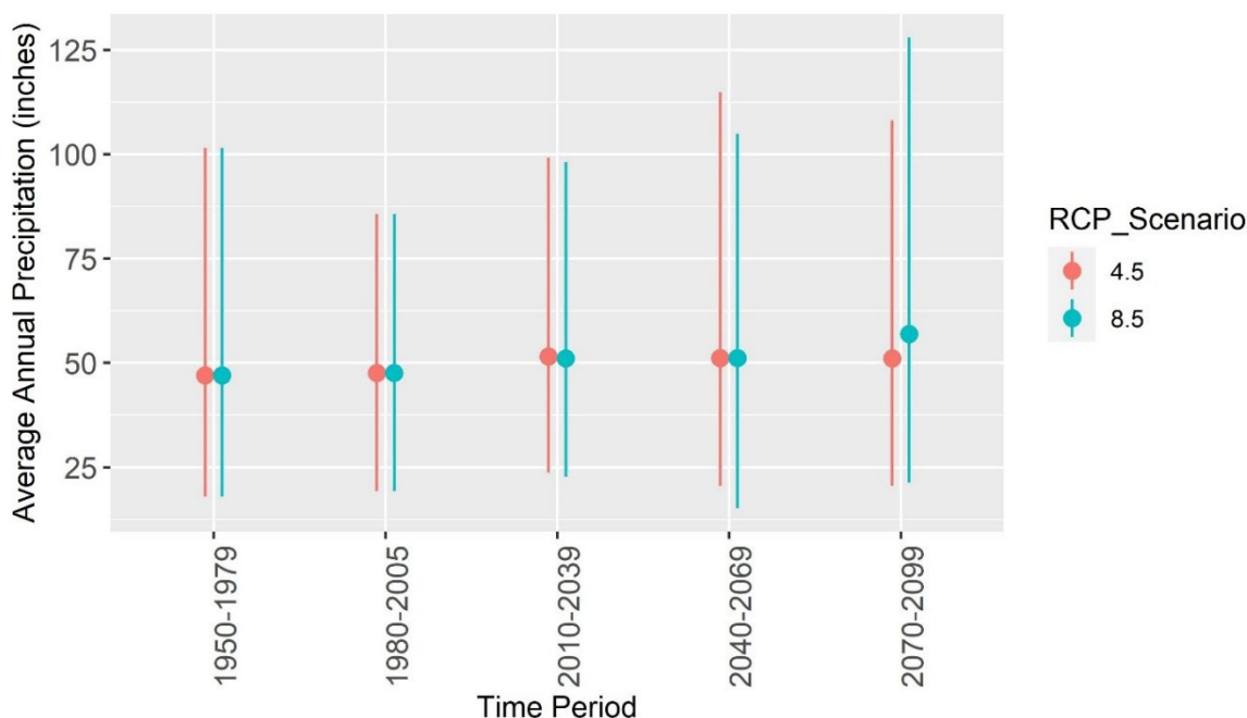
Figure 16. Modeled historic and future average annual precipitation on the Plumas National Forest summarized for 30-year periods. Points represent average while lines indicate range of data (minimum and maximum). Data source CalAdapt: See Table 4 footnote.
