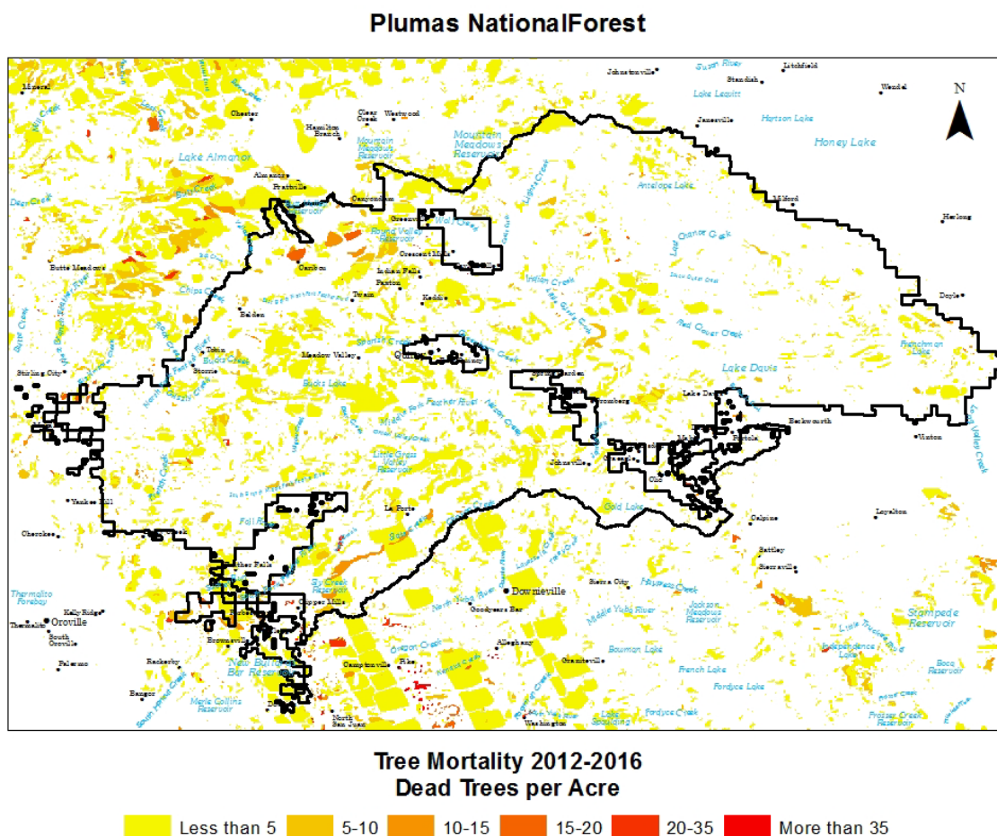
Figure 10. Recent (2012-2016) cumulative drought and insect-related mortality in the Plumas National Forest based on aerial detection surveys by the drought. Forest Service Forest Health Protection.
