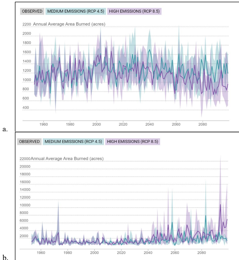
Figure 23. Wildfire simulations for Little Last Chance (a) and Lower North Fork Feather River (b) watersheds on the Plumas National Forest. Data source CalAdapt using wildfire scenario projections produced by Westerling (2018).
