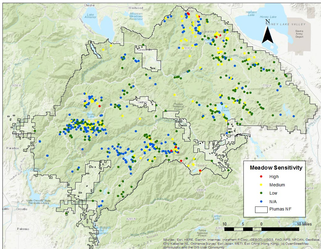
Figure 11. Meadow sensitivity on the Plumas National Forest based on the slope of the relationship between April 1 st snowpack and late season greenness (Normalized Difference Vegetation Index-NDVI) between 1984 to 2016.
