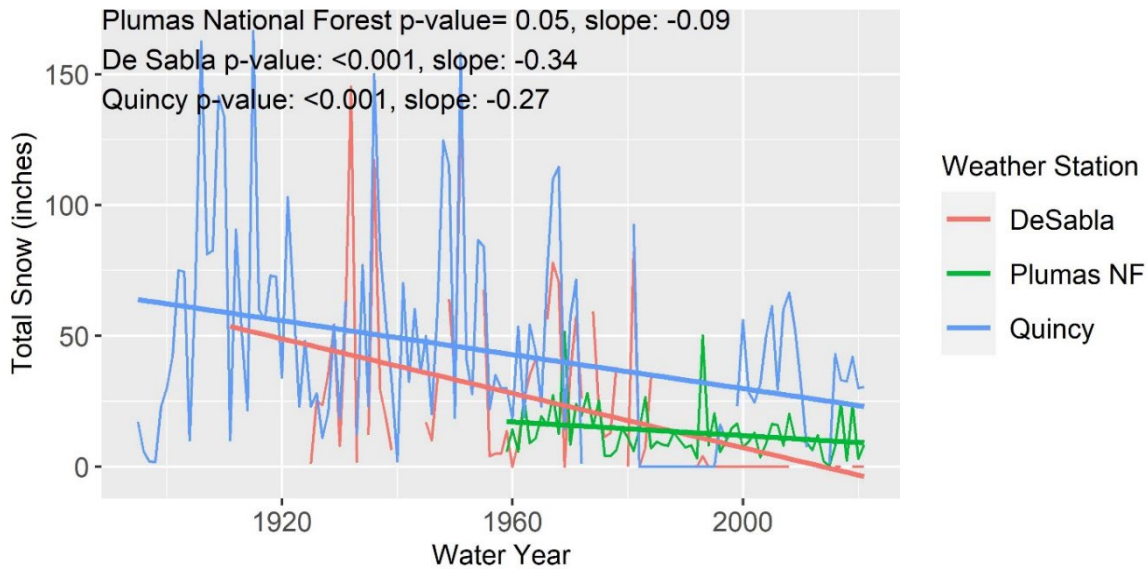
Figure 5. Total snowfall for local Plumas National Forest weather stations (identified in different colors). Linear lines indicate a significant trend. For all significant trends the level of significance (p-value) and magnitude and direction of trend (slope) are presented. *Note that data for the Plumas National Forest (Terra Climate) are Snow Water Equivalent (in inches), while data for the individual weather stations are Total Snow (in inches).
