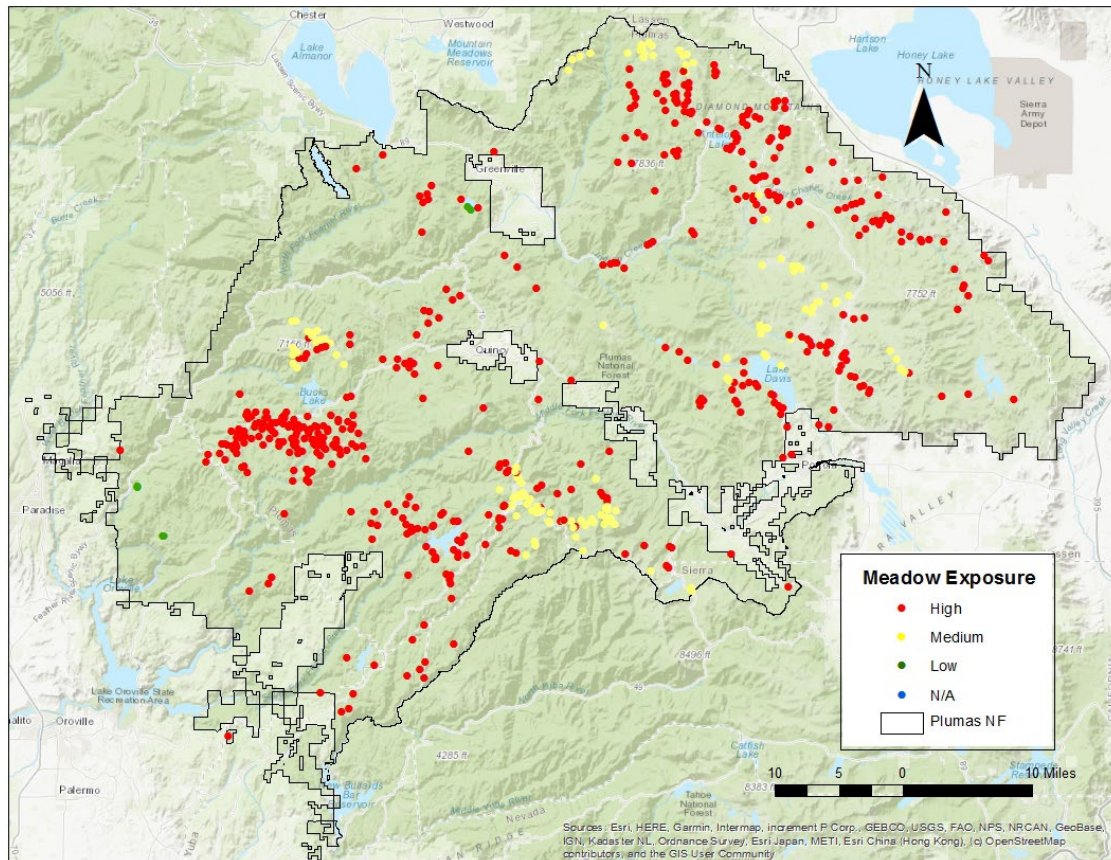
Figure 25. Future exposure of meadows on the Plumas National Forest based on the relative change in April 1 st snowpack between 1981-2010 and 2040-2069 using the climate model MIROC-RCP8.5.
