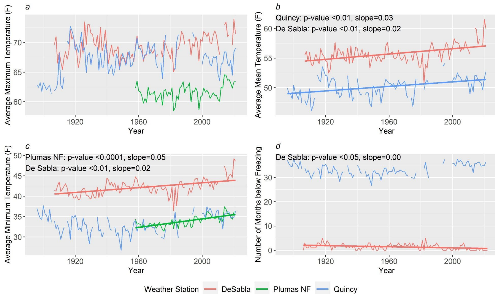
Figure 2. Historic temperature trends for Plumas National Forest weather stations (identified in different colors): a) Average Maximum Temperature, b) Average Mean Temperature, c) Average Minimum Temperature, and d) Number of Months below Freezing (months where the average minimum temperature was <32^{\circ}\text{F} ). Linear lines indicate a significant trend. For all significant trends the level of significance (p-value) and magnitude and direction of trend (slope) are presented.
