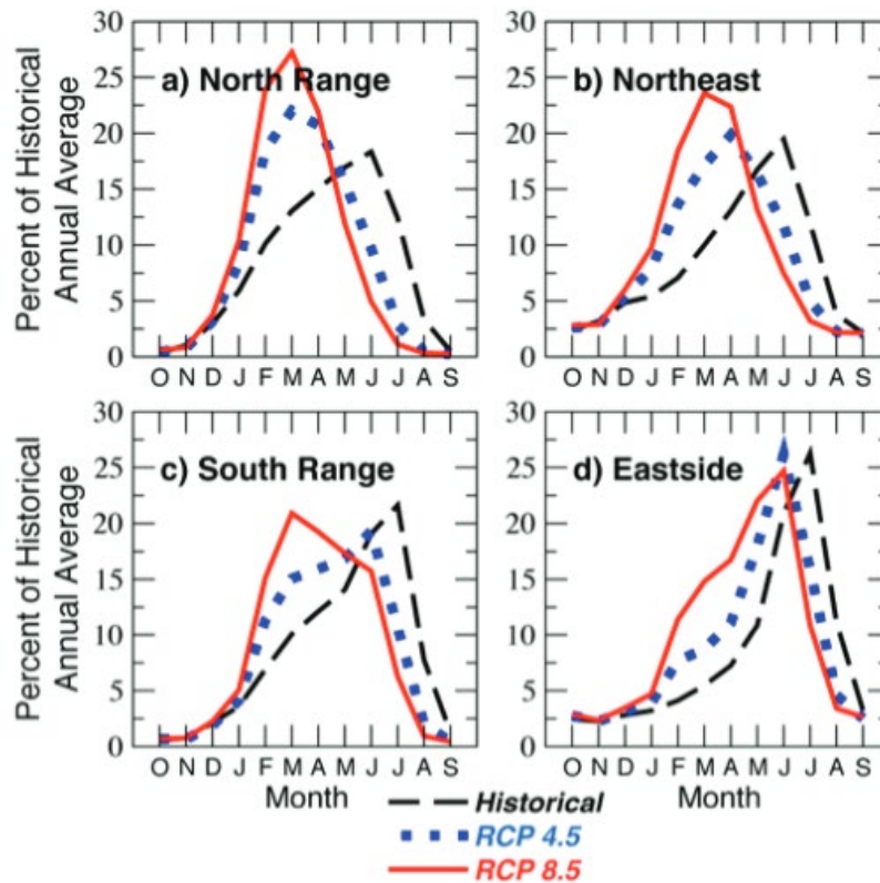
Figure 20. Ensemble averages of 2070-2099 runoff hydrographs for the Sierra Nevada subregions with each month's runoff shown as a percentage of the historical (1961-1990) annual-total norms--from ten climate models responding to two greenhouse-gas futures, where “runoff” is the water that avoids evaporation and use by plants to flow off or into land surfaces (essentially, surface water flows and groundwater recharge generated by a given area). Notably (d) Eastside responses shown mostly reflect snowmelt and runoff from the eastern slopes of the Sierra Nevada. Adapted from (Dettinger et al. 2018).
