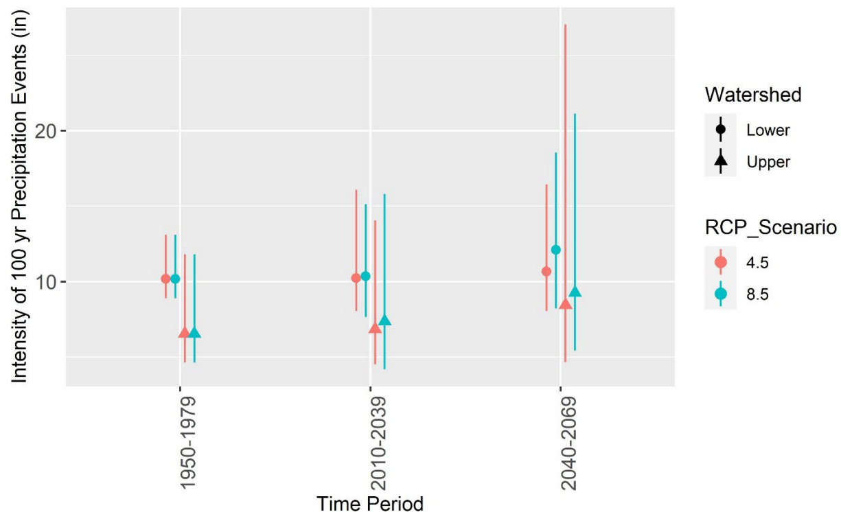
Figure 18. Modeled intensity of extreme precipitation events that on average occur every 100 years for the upper watershed (Little Last Chance Watershed – 2.53 inches) and the lower watershed (Lower North Fork Feather River Watershed – 0.75 inches) on the Plumas National Forest summarized for 30-year periods. Points represent average, while lines indicate the maximum upper and maximum lower 95% confidence interval. Data source CalAdapt: See Table 4 footnote.
