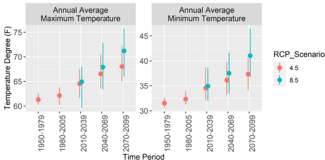
Figure 13. Modeled historic and future average minimum and maximum temperature on the Plumas National Forest summarized for 30-year periods. Points represent average while lines indicate range of data (minimum and maximum). Data source CalAdapt: See Table 4 footnote.
