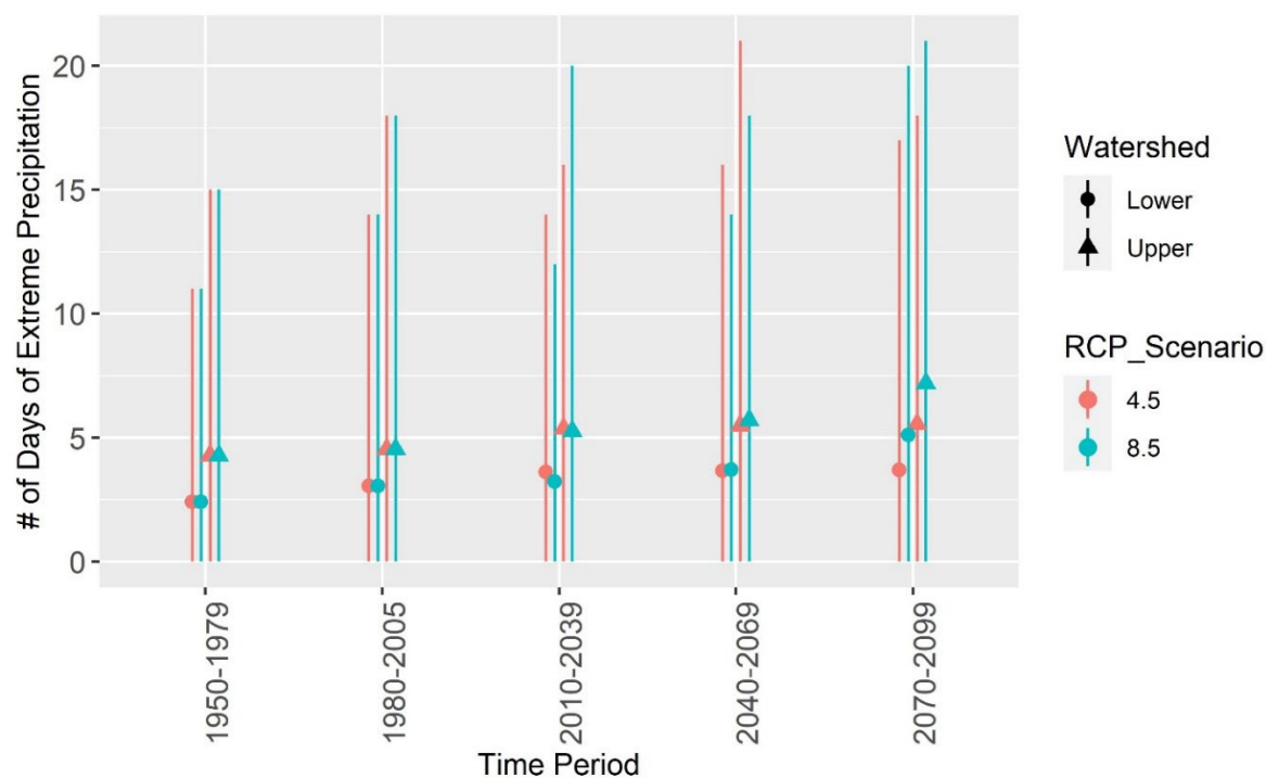
Figure 17. Modeled number of days of extreme precipitation in a water year with 2-day rainfall totals above the extreme threshold for the upper watershed, (Little Last Chance Watershed - 0.75 inches) and the lower watershed (Lower North Fork Feather River Watershed - 2.53 inches) on the Plumas National Forest summarized for 30-year periods. Points represent average, while lines indicate the minimum and maximum. Data source CalAdapt: See Table 4 footnote.
