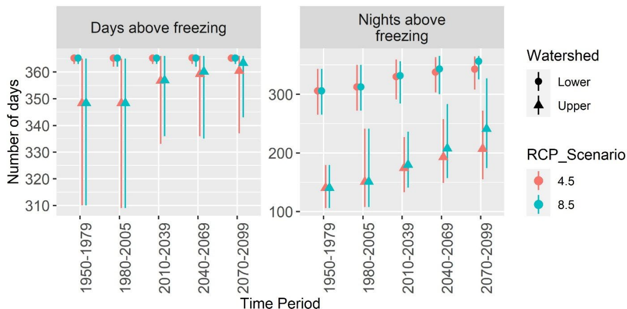
Figure 14. Modeled number of days above freezing (32°F) for the Little Last Chance Watershed (upper) and North Fork Feather River (lower) watersheds on the Plumas National Forest summarized for 30-year periods. Points represent the average while lines indicate range of data. Data source CalAdapt: See Table 4 footnote. Days above freezing and nights above freezing are based on when the daily maximum/minimum exceeds 32°F.
