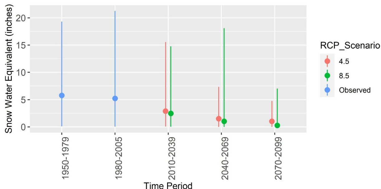
Figure 19: Historic observed and future predicted April 1 st Snow Water Equivalent (SWE) on the Plumas National Forest summarized for 30-year periods under two emission scenarios (RCP 4.5 and RCP 8.5). Points represent average while lines indicate range of data (minimum and maximum). Data source CalAdapt: See Table 4 footnote.
