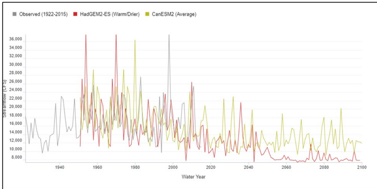
Figure 21.. This chart shows total annual unimpaired flows in a water year (October – September) for June, July, and August. Data are shown for the Sacramento River at Red Bluff under the RCP 8.5 scenario in which emissions continue to rise strongly through 2050 and plateau around 2100. Values represent observed streamflow (1922-2015) and global climate models of CanESM2 (an average simulation) and HadGEM2-ES (a warm/drier simulation).
