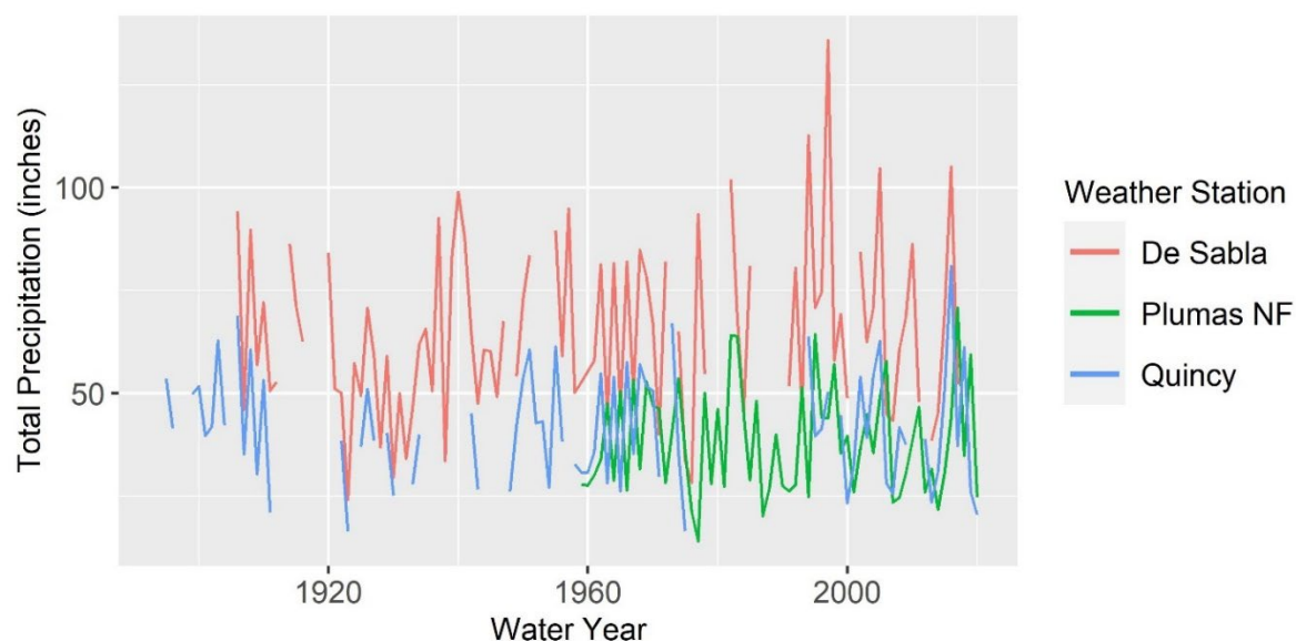
Figure 3. Total precipitation for local Plumas National Forest weather stations (identified in different colors).
