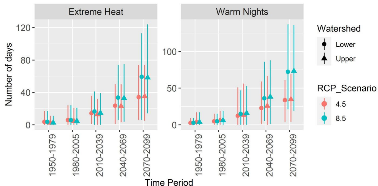
Figure 15. Modeled extreme heat days and warm nights for the Little Last Chance (upper) and the Lower North Fork Feather River (lower) watersheds on the Plumas National Forest summarized for 30-year periods. Points represent the average while lines indicate range of data. Data is based on the 98 th percentile for what is currently considered extremely hot for the specific area between April through October. The 98 th percentile for extreme heat (maximum temperature) is 91.1°F and 97.7°F and for warm nights (minimum temperature) is 50.1°F and 63.8°F for the Little Last Chance Watershed and the Lower North Fork Feather River Watershed, respectively. Data source CalAdapt: See Table 4 footnote.
