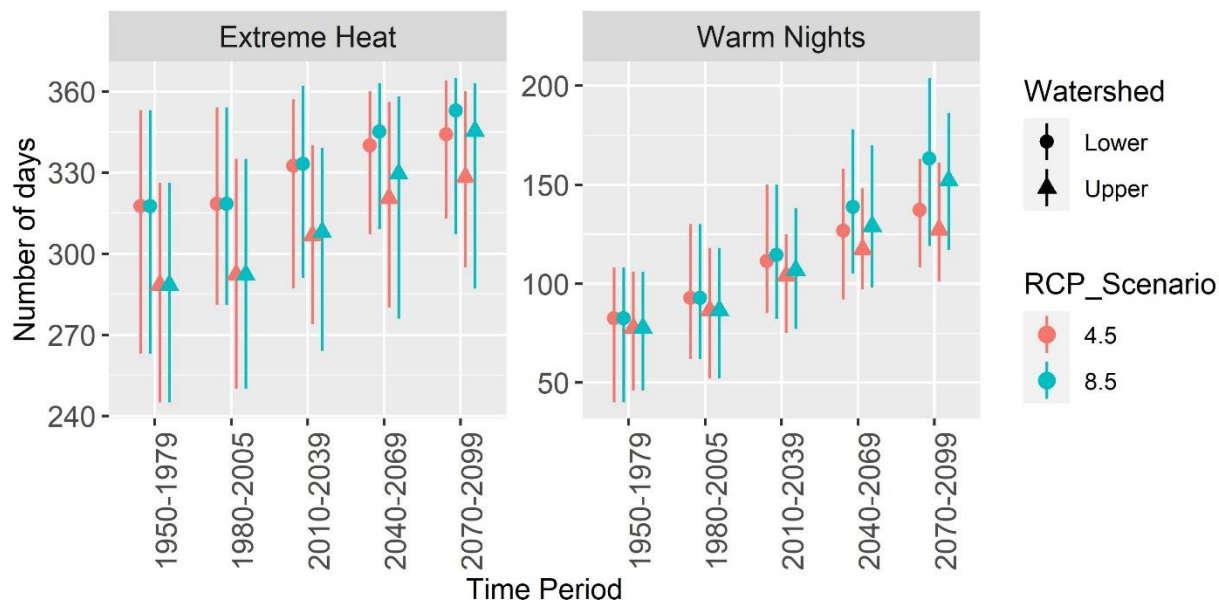
Figure 15. Modeled extreme heat days and warm nights for the Kaiser Creek/ Upper San Joaquin and the Willow Creek Watershed on the Sierra National Forest summarized for 30-year periods. Points represent the average while lines indicate range of data. Data is based on the 98 th percentile for what is currently considered extremely hot for the specific area between April through October. The 98 th percentile for extreme heat (maximum temperature) is 83.7°F and 91.6°F and for warm nights (minimum temperature) is 53.5°F and 58.4°F for the Kaiser Creek- Upper San Joaquin River Watershed and the Willow Creek Watershed, respectively. Data source CalAdapt: See Table 3 footnote.
