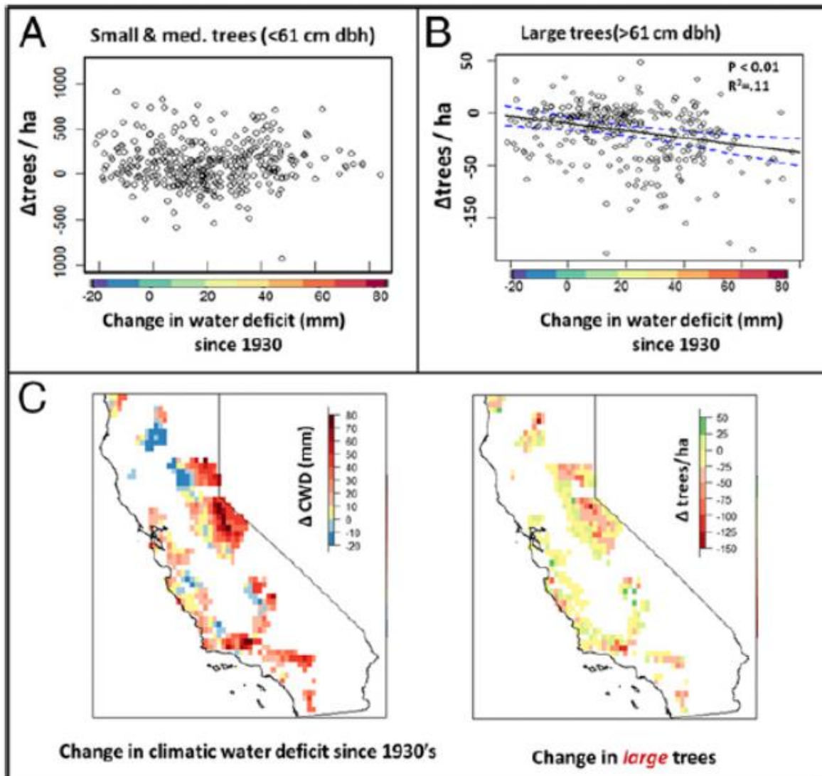
Figure 9. Changes in tree density and climatic water deficit between Wieslander and existing conditions for small & medium trees (A&C) and large trees (B&C) (McIntyre et al. 2015).
