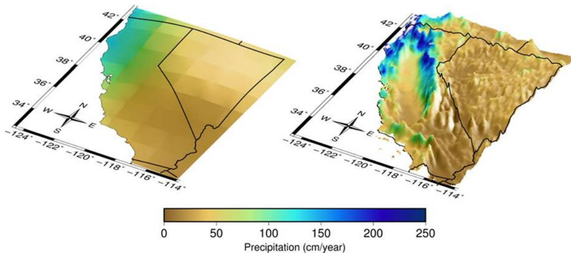
Figure 12. Annual precipitation in California and Nevada (250 cm = ~100 inches). On the left is a global climate model with a resolution of 100 miles. On the right, downscaled model with a resolution of about 3.7 miles. Note how the downscaled model is better able to better capture the wet conditions on the west slope and drier conditions on the east slope of the Sierra Nevada. Image was taken from (Pierce et al. 2018) where the vertical scale has been equally exaggerated in both images for clarity.
