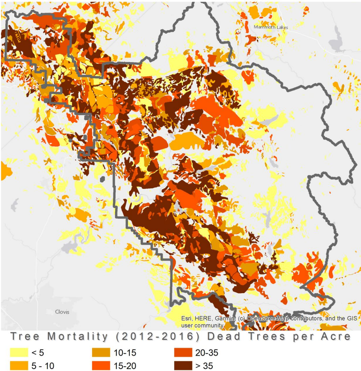
Figure 10. Recent (2012-2016) cumulative drought and insect-related mortality in the Sierra National Forest based on aerial detection surveys by the drought. Forest Service Forest Health Protection.
