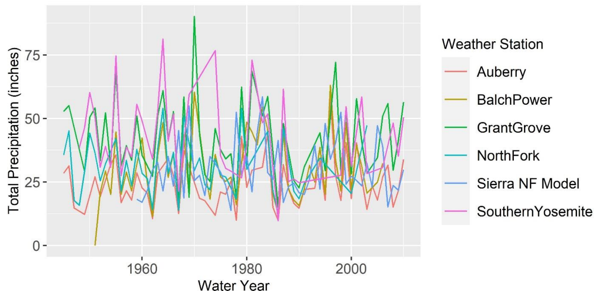
Figure 3. Total precipitation for local Sierra National Forest weather stations (identified in different colors).
