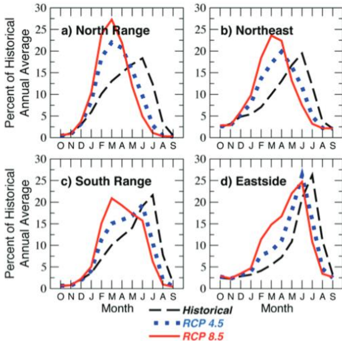
Figure 20. Ensemble averages of 2070-2099 runoff hydrographs for the Sierra Nevada subregions shown in Fig. 1.1a—with each month’s runoff shown as a percentage of the historical (1961-1990) annual-total norms—from ten climate models responding to two greenhouse-gas futures, where “runoff” is the water that avoids evaporation and use by plants to flow off or into land surfaces (essentially, surface water flows and groundwater recharge generated by a given area). Notably (d) Eastside responses shown mostly reflect snowmelt and runoff from the eastern slopes of the Sierra Nevada. Adapted from (Dettinger et al. 2018).
