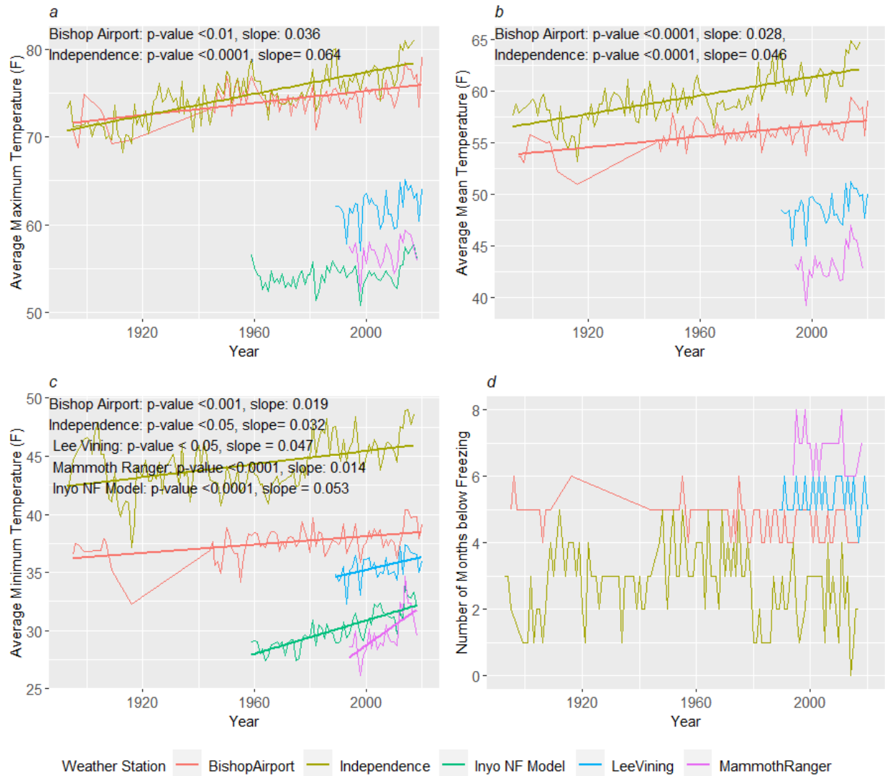
Figure 2. Historic temperature trends for Inyo National Forest weather stations (identified in different colors): a) Average Maximum Temperature, b) Average Mean Temperature, c) Average Minimum Temperature, and D) Number of Months below Freezing (months where the average minimum temperature was <32°F). Linear lines indicate a significant trend. For all significant trends the level of significance (p-value) and magnitude and direction of trend (slope) are presented.
