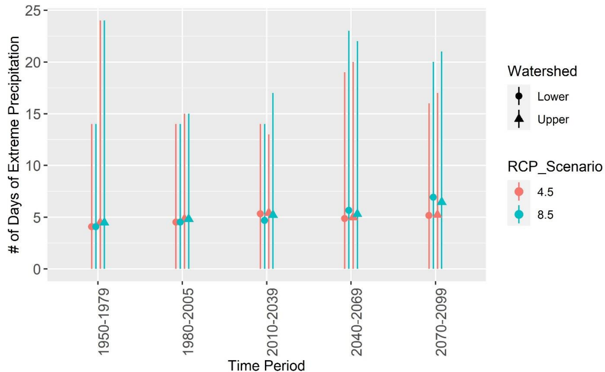
Figure 16. Modeled number of days of extreme precipitation in a water year with 2-day rainfall totals above the extreme threshold for the Bishop Creek (1.84 inches) and the Lee Vining Creek – Frontal Mono Lake Watershed (1.84 inches) on the Inyo National Forest summarized for 30-year periods. Points represent average, while lines indicate the minimum and maximum. Data source CalAdapt: See Table 3 footnote.
