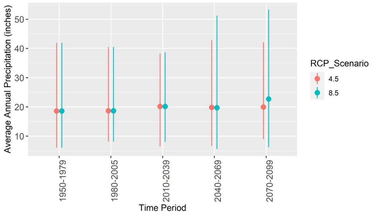
Figure 15. Modeled historic and future average annual precipitation on the Inyo National Forest summarized for 30-year periods. Points represent average while lines indicate range of data (minimum and maximum). Data source CalAdapt: See Table 3 footnote.
