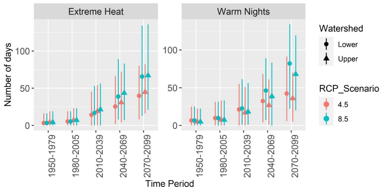
Figure 14. Modeled extreme heat days and warm nights for the Bishop Creek Watershed and the Lee Vining Creek Frontal Watershed on the Inyo National Forest summarized for 30-year periods. Points represent the average while lines indicate range of data. Data is based on the 98 th percentile for what is currently considered extremely hot for the specific area between April through October. The 98 th percentile for extreme heat (maximum temperature) is 79.3°F and 82.9°F and for warm nights (minimum temperature) is 44.8°F and 46.4°F for the Bishop Creek Watershed and the Lee Vining Creek – Mono Lake Frontal Watershed, respectively. Data source CalAdapt: See Table 3 footnote.
