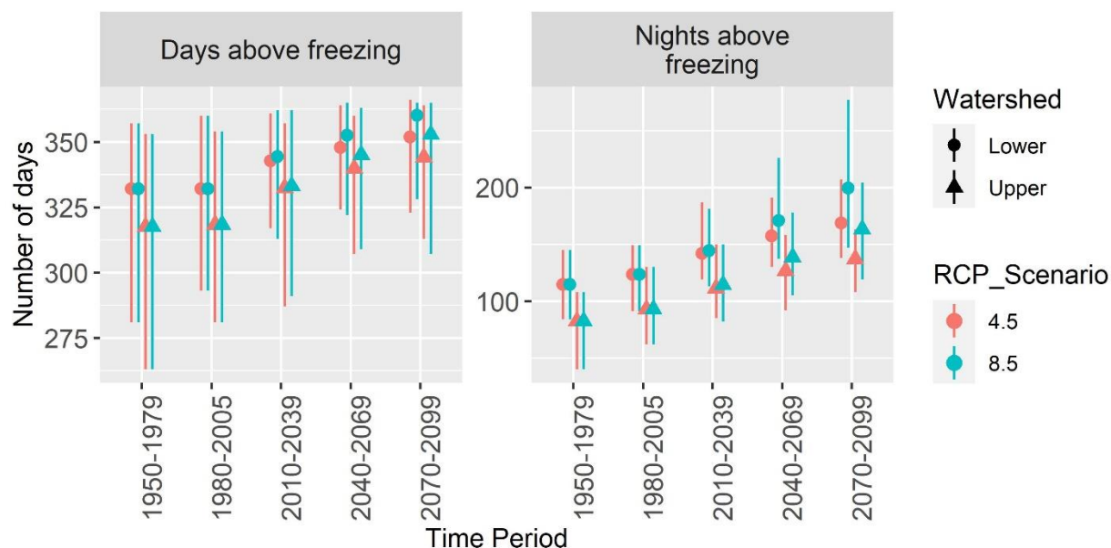
Figure 13. Modeled number of days above freezing (32°F) for the Lee Vining Creek Frontal Bishop Creek Watershed and Lee Vining Creek – Mono Lake Frontal Watershed Creek Watershed on the Inyo National Forest summarized for 30-year periods. Points represent the average while lines indicate range of data. Data source CalAdapt: See Table 3 footnote. Days above freezing and nights above freezing are based on when the daily maximum/minimum exceeds 32°F.
