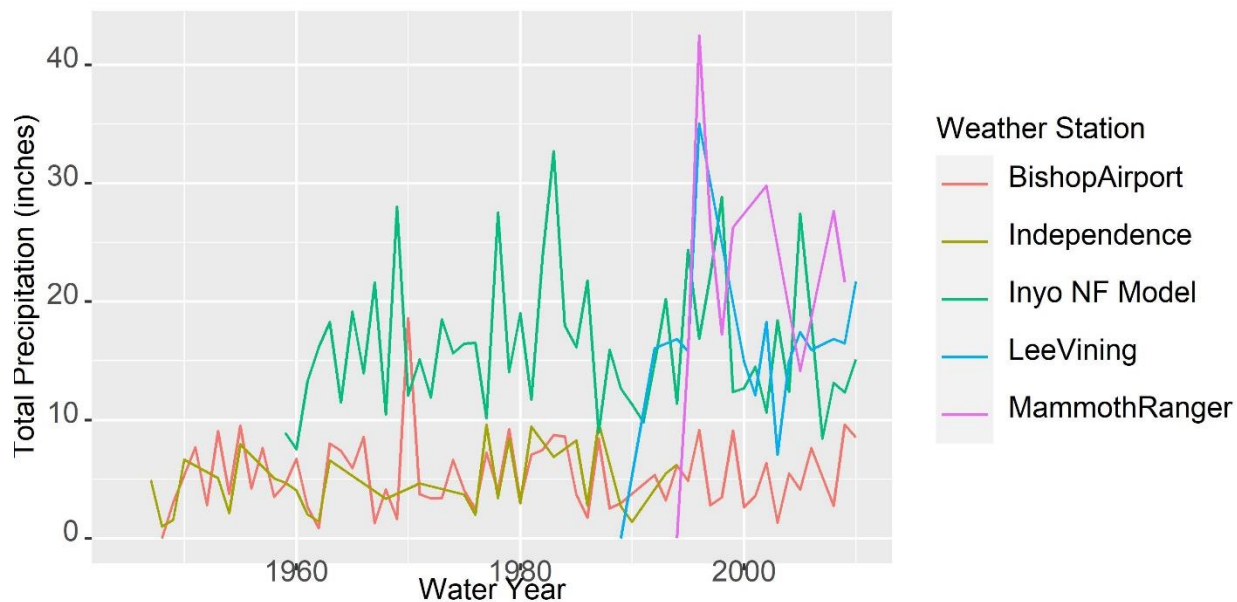
Figure 3. Total precipitation for local Inyo National Forest weather stations (identified in different colors).
