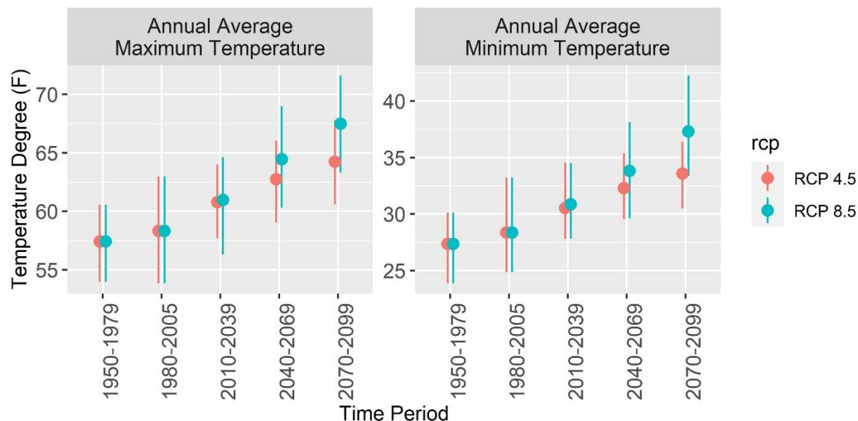
Figure 12. Modeled historic and future average minimum and maximum temperature on the Inyo National Forest summarized for 30-year periods. Points represent average while lines indicate range of data (minimum and maximum). Data source CalAdapt: See Table 3 footnote.
