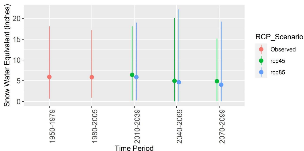
Figure 18: Historic observed and future predicted April 1 st Snow Water Equivalent (SWE) on the Inyo National Forest summarized for 30-year periods under two emission scenarios (RCP 4.5 and RCP 8.5). Points represent average while lines indicate range of data (minimum and maximum). Data source CalAdapt: See Table 3 footnote.
