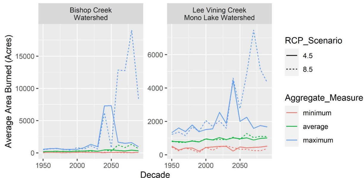
Figure 21. Wildfire simulations for two watersheds on the Inyo National Forest smoothed by decade. Data source CalAdapt using wildfire scenario projections produced by Westerling (2018).
