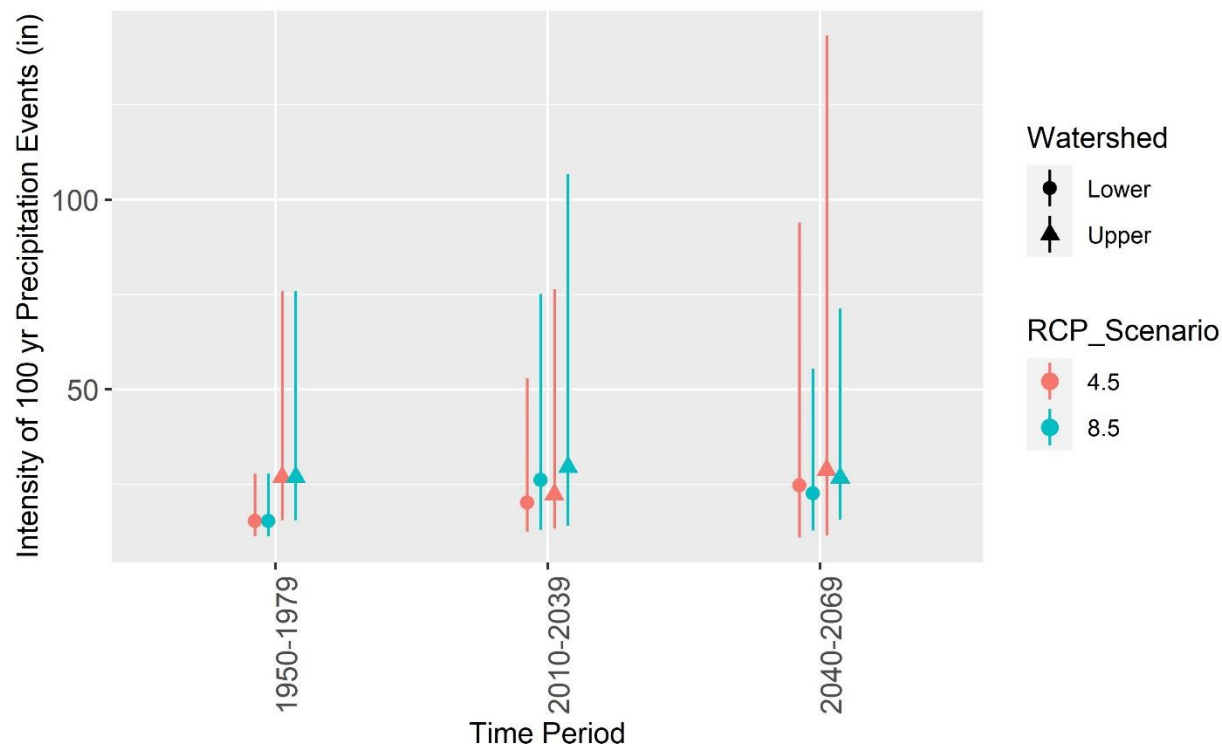
Figure 17. Modeled intensity of extreme precipitation events that on average occur every 100 years for the Upper Watershed (Bishop Creek- 27 inches) and the Lower Watershed (Lee Vining –Frontal Mono Lake Lee Vining Creek – Mono Lake Frontal Watershed – 15.2 inches) on the Inyo National Forest summarized for 30-year periods. Points represent average, while lines indicate the maximum upper and maximum lower 95% confidence interval. Data source CalAdapt: See Table 3 footnote.
