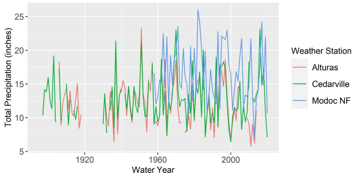
Figure 3. Total precipitation for local Modoc National Forest weather stations (identified in different colors).
