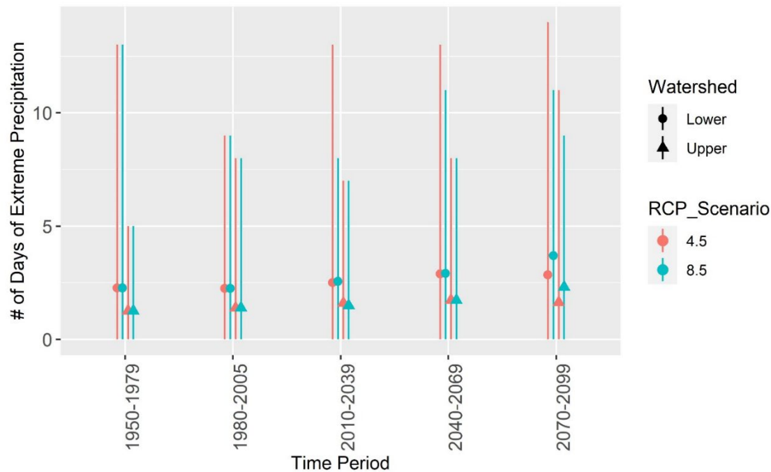
Figure 16. Modeled number of days of extreme precipitation in a water year with 2-day rainfall totals above the extreme threshold for the lower elevation Taylor Reservoir Watershed (threshold = 2.33 inches) and the upper elevation Jess Valley-South Fork Pit River Watershed (threshold = 1.45 inches) on the Modoc National Forest summarized for 30-year periods. Points represent average, while lines indicate the minimum and maximum. Data source CalAdapt: See Table 4 footnote.
