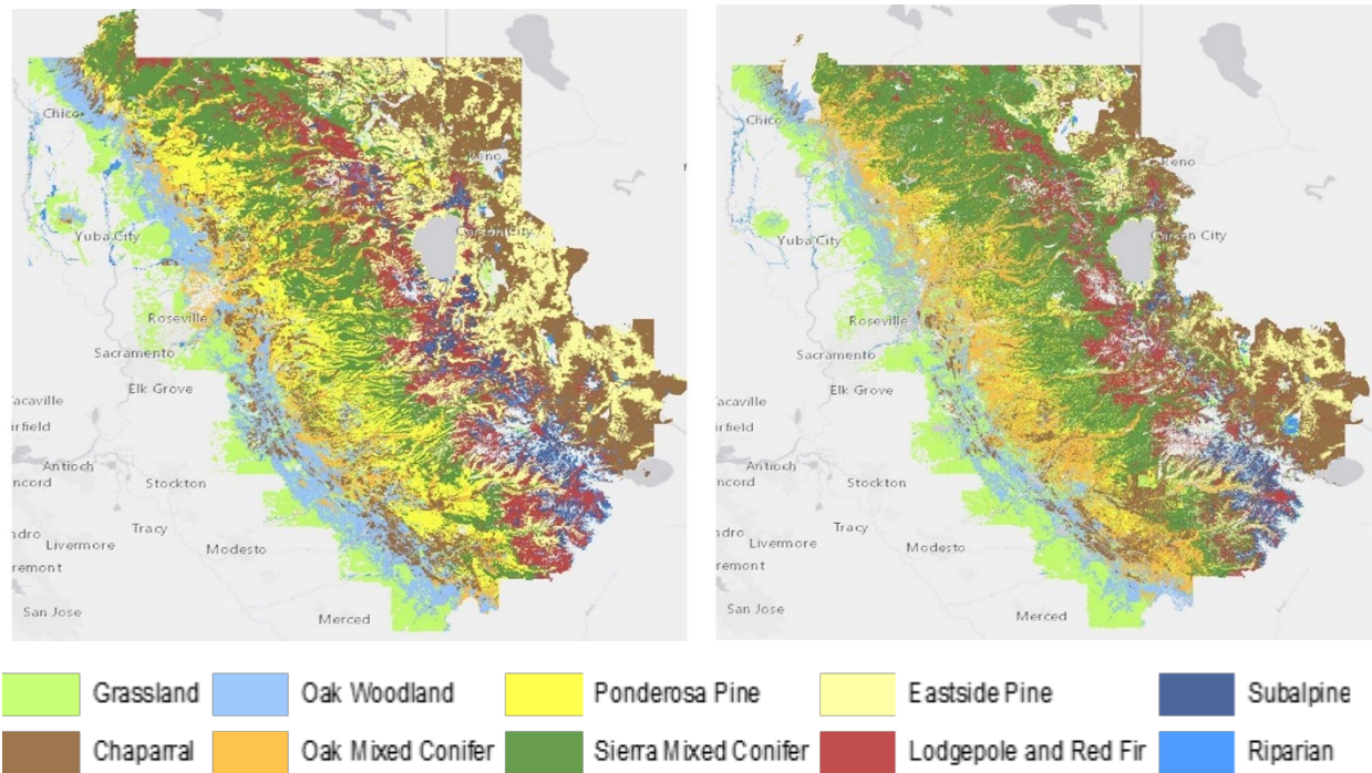
Figure 6. The distribution of major vegetation types in the Sierra Nevada in the period from 1932-1936 as mapped by Wieslander (left panel) compared to current conditions (right panel).
