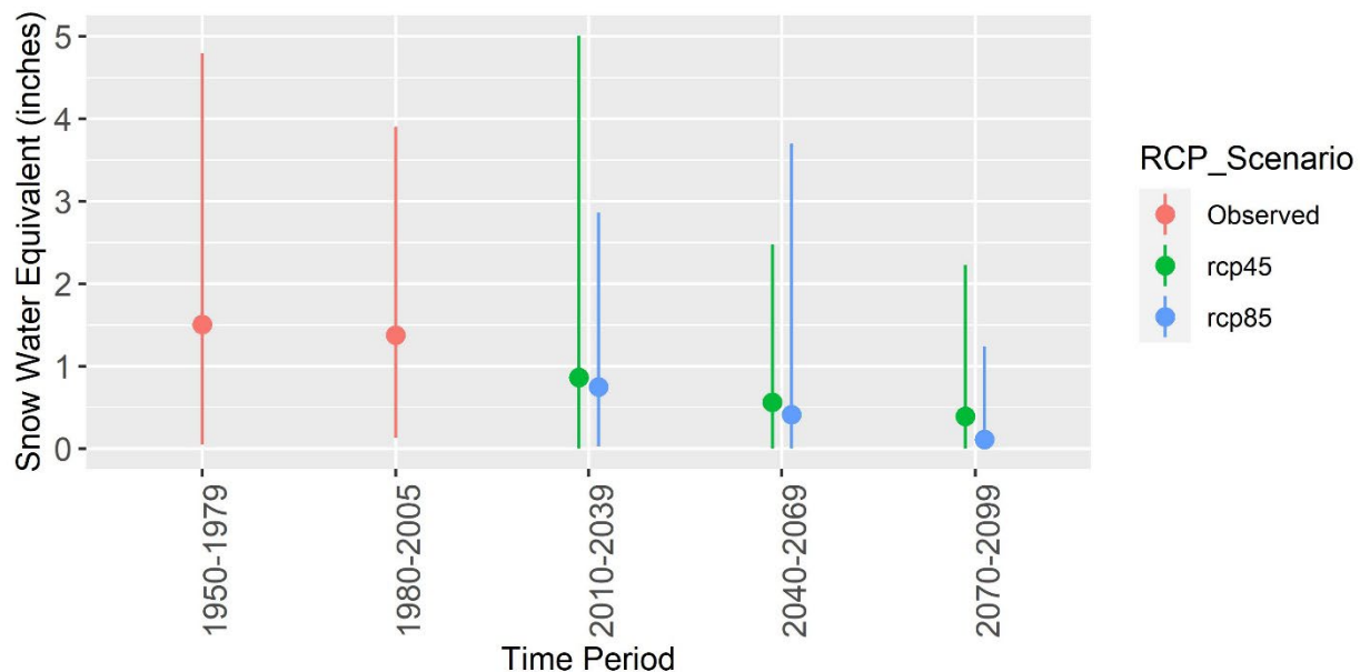
Figure 18. Historic observed and future predicted April 1 st Snow Water Equivalent (SWE) on the Modoc National Forest summarized for 30-year periods under two emission scenarios (RCP 4.5 and RCP 8.5). Points represent average while lines indicate range of data (minimum and maximum). Data source CalAdapt: See Table 4 footnote.
