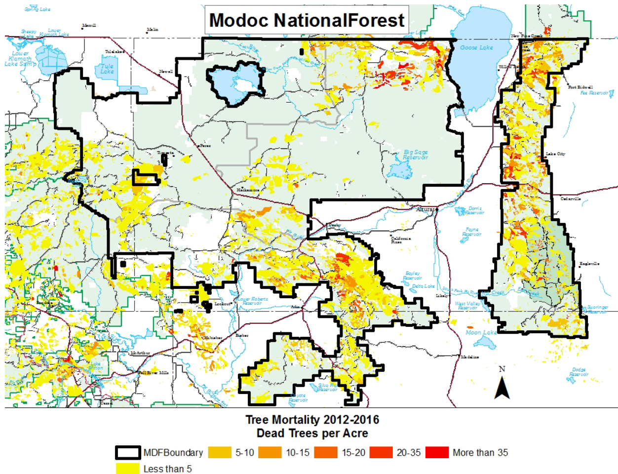
Figure 9. Recent (2012-2016) cumulative drought and insect-related mortality on the Modoc National Forest based on aerial detection surveys by the Forest Health Protection Program.
