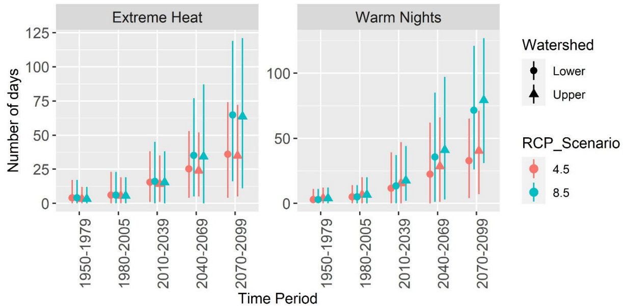
Figure 14. Modeled extreme heat days and warm nights for the Jess Valley-Pitt River and the Taylor Reservoir watersheds on the Modoc National Forest summarized for 30-year periods. Points represent the average while lines indicate range of data. Data is based on the 98 th percentile for what is currently considered extremely hot for the specific area between April through October. The 98 th percentile for extreme heat (maximum temperature) is 87.6°F and 93.1°F and for warm nights (minimum temperature) is 49.4°F and 53.7°F for the Jess Valley-Pitt River and the Taylor Reservoir watersheds, respectively. Data source CalAdapt: See Table 4 footnote.
