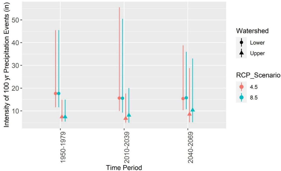
Figure 17. Modeled intensity of extreme precipitation events that on average occur every 100 years for the Upper Watershed (Jess Valley-South Fork Pit River Watershed – 1.45 inches) and the Lower Watershed (Taylor Reservoir Watershed - 2.33 inches) on the Modoc National Forest summarized for 30-year periods. Points represent average, while lines indicate the maximum upper and maximum lower 95% confidence interval. Data source CalAdapt: See Table 4 footnote.
