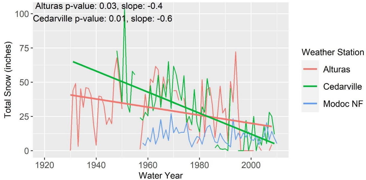
Figure 4. Total snowfall for local Modoc National Forest weather stations (identified in different colors). Linear lines indicate a significant trend. For all significant trends the level of significance (p-value) and magnitude and direction of trend (slope) are presented. *Note that data for the Modoc National Forest (Terra Climate) are Snow Water Equivalent (in inches), while data for the individual weather stations are Total Snow (in inches).
