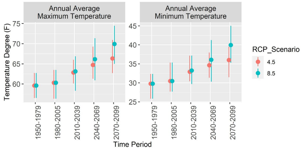
Figure 12. Modeled historic and future average minimum and maximum temperature on the Modoc National Forest summarized for 30-year periods. Points represent average while lines indicate range of data (minimum and maximum). Data source CalAdapt: See Table 4 footnote.
