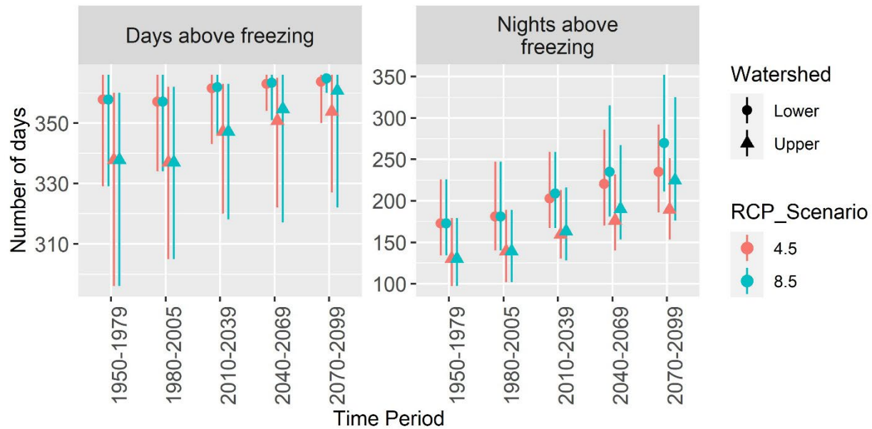
Figure 13. Modeled number of days above freezing (32°F) for the Jess Valley-South Fork Pit River Watershed (upper) and Taylor Reservoir Watershed (lower) on the Modoc National Forest summarized for 30-year periods. Points represent the average while lines indicate range of data. Data source CalAdapt: See Table 4 footnote. Days above freezing and nights above freezing are based on when the daily maximum/minimum exceeds 32°F.
