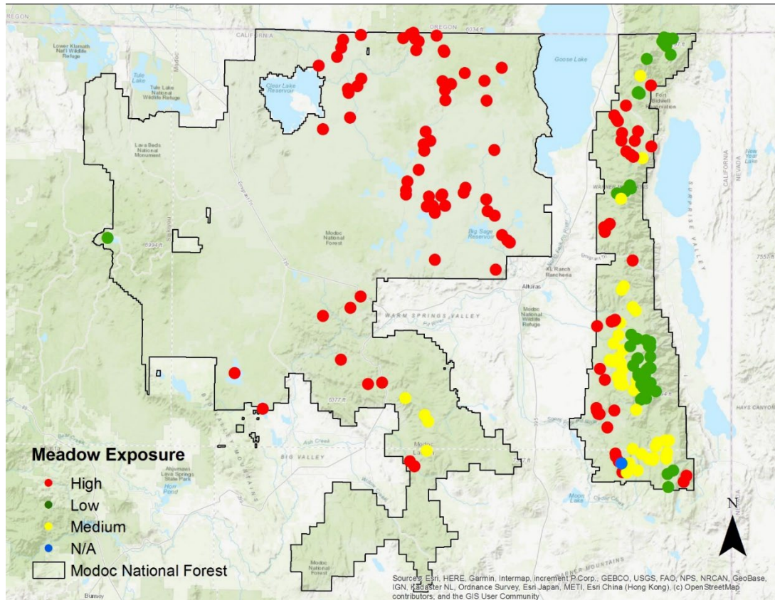
Figure 24. Future exposure of meadows on the Modoc National Forest based on the relative change in April 1 st snowpack between 1981-2010 and 2040-2069 using the climate model MIROC-RCP8.5.
