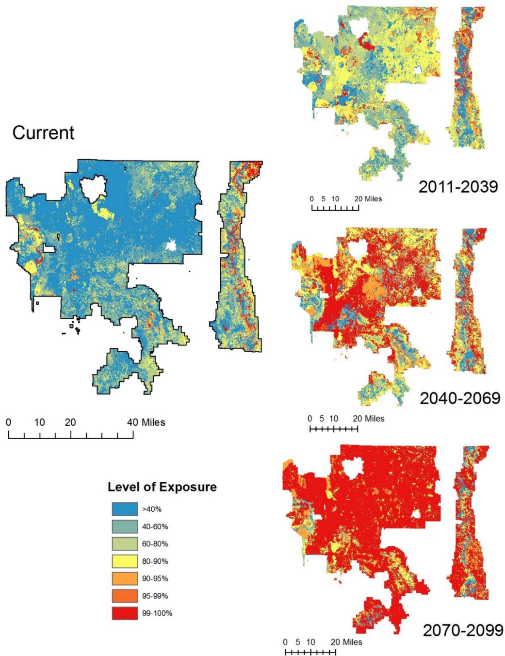
Figure 23. Mapped climate exposure under the “Warm and Wet” CNRM CM5 climate projection under Higher Emissions RCP8.5. This image shows the climate exposure of Modoc National Forest vegetation types at current time and three future periods: 2011–2039, 2040–2069, and 2070–2099. Areas considered to be highly climatically exposed are in the 95–99% and 99–100%. Areas with values <80% are considered to be in climatically suitable conditions for the vegetation that it currently occupies.
