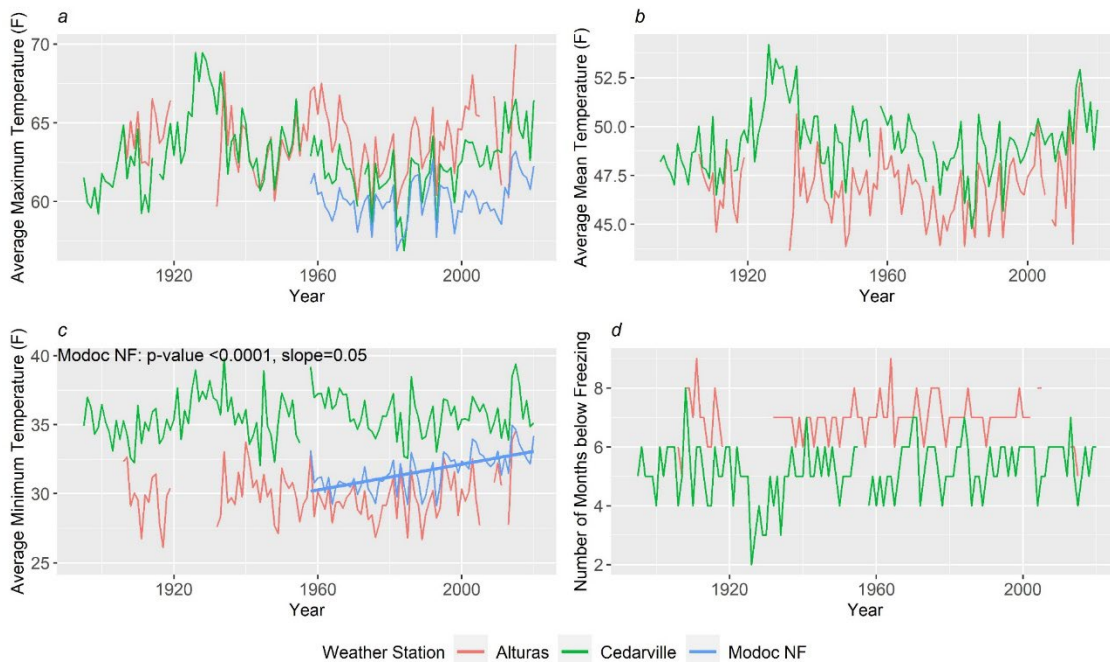
Figure 2. Historic temperature trends for Modoc National Forest weather stations (identified in different colors): a) Average Maximum Temperature, b) Average Mean Temperature, c) Average Minimum Temperature, and D) Number of Months below Freezing (months where the average minimum temperature was <32^{\circ}\text{F} ). Linear lines indicate a significant trend. For all significant trends the level of significance (p-value) and magnitude and direction of trend (slope) are presented.
