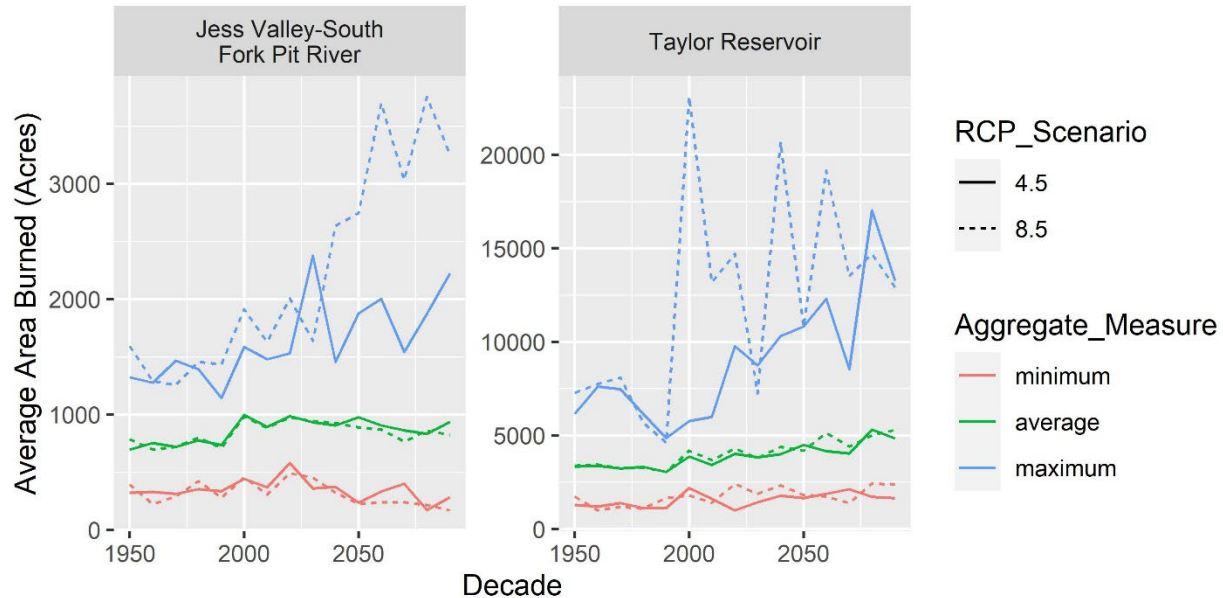
Figure 22. Wildfire simulations for two watersheds on the Modoc National Forest smoothed by decade. Data source CalAdapt using wildfire scenario projections produced by Westerling (2018).
