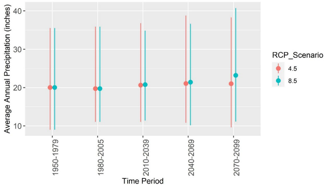
Figure 15. Modeled historic and future average annual precipitation on the Modoc National Forest summarized for 30-year periods. Points represent average while lines indicate range of data (minimum and maximum). Data source CalAdapt: See Table 4 footnote.
