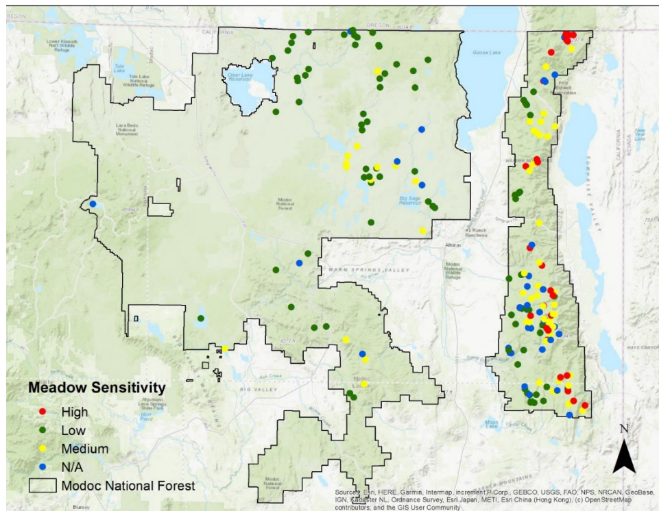
Figure 10. Meadow sensitivity on the Modoc National Forest based on the slope of the relationship between April 1 st snowpack and late season greenness (Normalized Difference Vegetation Index-NDVI) between 1984 to 2016.
