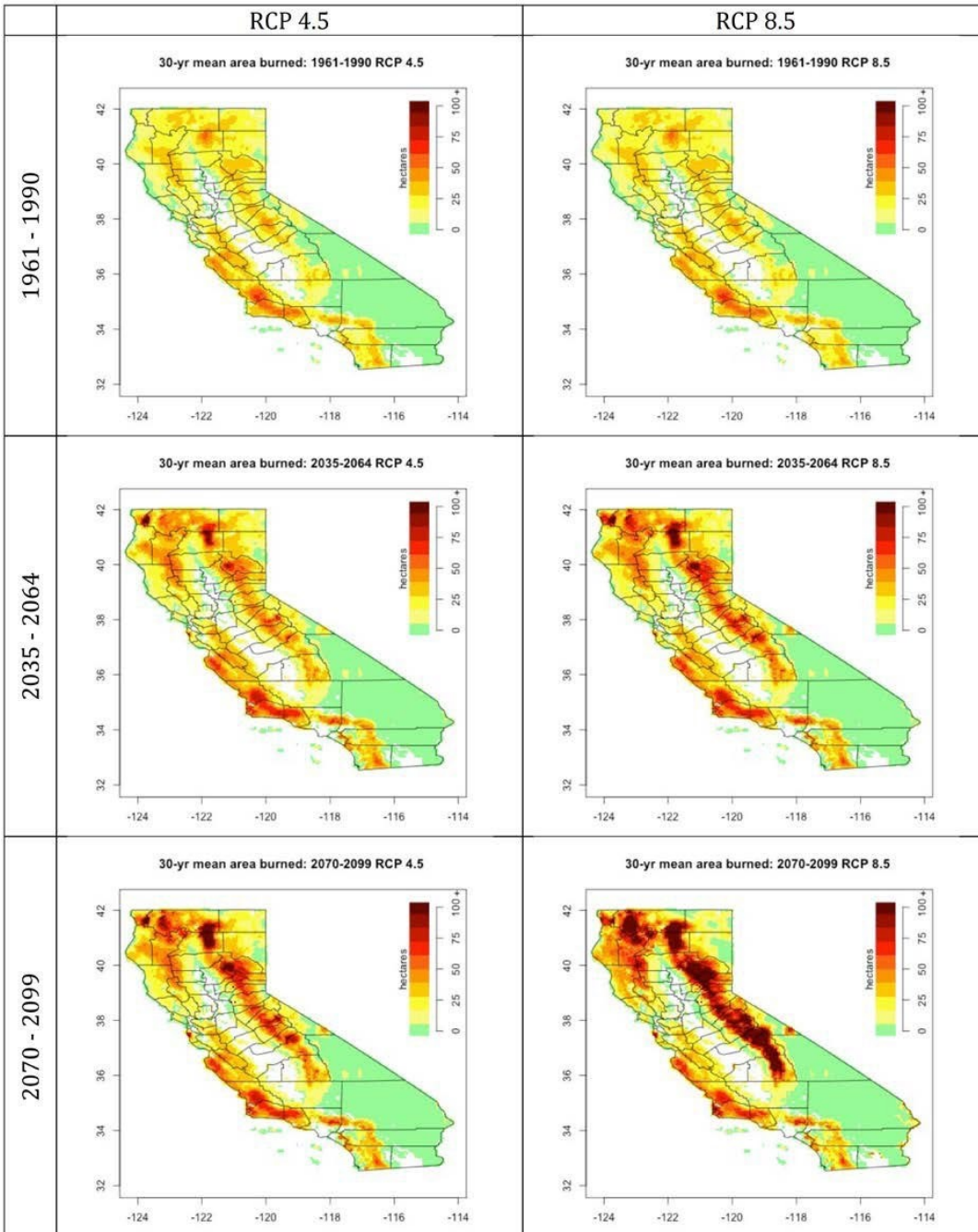
Figure 15. Average annual area burned composites: RCP 4.5 (left), RCP 8.5 (right) from Westerling (2018).
