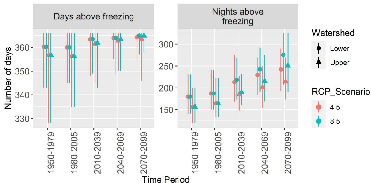
Figure 8. Modeled number of days above freezing (32°F) for the Little Shasta River Watershed (upper) and Thompson Creek-Klamath River Watershed (lower) on the Klamath National Forest summarized for 30-year periods. Points represent the average while lines indicate range of data. Data source CalAdapt: see Table 4 footnote. Days above freezing and nights above freezing are based on when the daily maximum/minimum exceeds 32°F.
