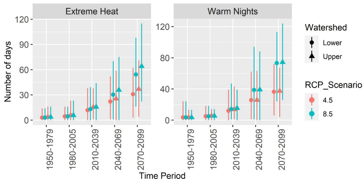
Figure 9. Modeled extreme heat days and warm nights for the Little Shasta River Watershed (upper) and the Thompson Creek-Klamath River Watershed (lower) on the Klamath National Forest summarized for 30-year periods. Points represent the average while lines indicate range of data. Data is based on the 98 th percentile temperature between April and October. The 98 th percentile for extreme heat (max. temp.) is 95.6°F for the Thompson Creek-Klamath River Watershed and 92.2°F for the Little Shasta River Watershed. 98 th percentile for warm nights (min. temp.) is 51.0°F and 51.5°F for the Thompson Creek-Klamath River Watershed and the Little Shasta River Watershed, respectively. Data source CalAdapt: see Table 4 footnote.
