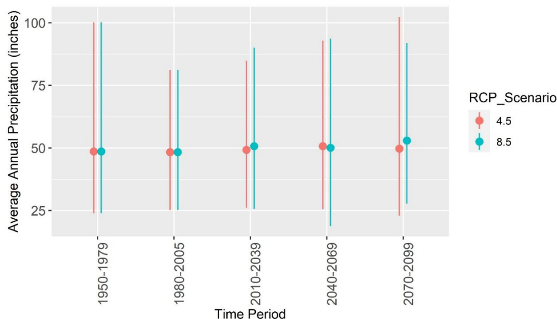
Figure 10. Modeled historic and future average annual precipitation on the Klamath National Forest summarized for 30-year periods. Points represent average while lines indicate range of data (minimum and maximum). Data source CalAdapt: See Table 4 footnote.
