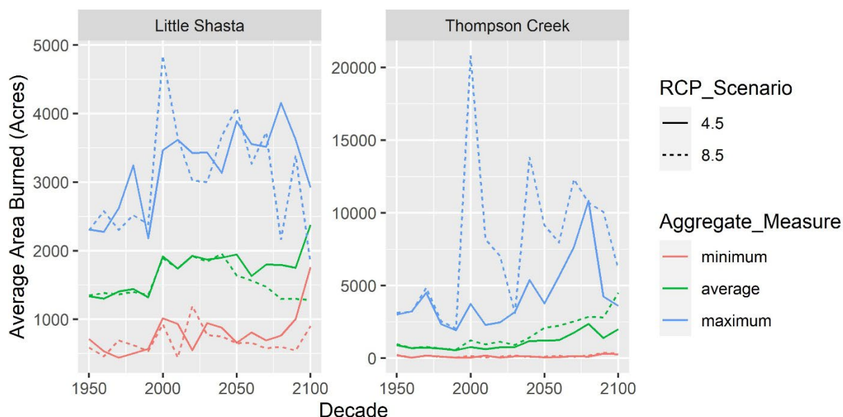
Figure 16. Wildfire simulations for two watersheds on the Klamath National Forest smoothed by decade. Data source CalAdapt using wildfire scenario projections produced by Westerling (2018).
