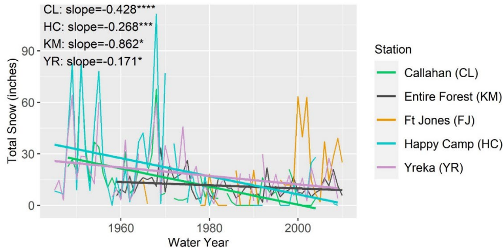
Figure 5. Total snowfall for local Klamath National Forest weather stations (identified in different colors), and for the Klamath National Forest overall (shown in black). Linear lines indicate a significant trend. For all significant trends the magnitude and direction of trend (slope) are presented, and the level of significance is indicated by number of asterisks (* p < 0.05 , ** p < 0.01 , *** p < 0.001 , **** p < 0.0001 ) 2 . Note that data for the Klamath National Forest are snow water equivalent (inches), while data for the individual weather stations are total snow (inches).
