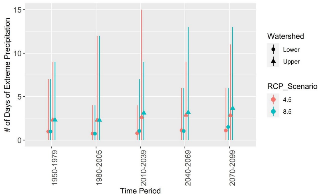
Figure 11. Modeled number of days of extreme precipitation in a water year with 2-day rainfall totals above the extreme threshold for the Little Shasta River Watershed (0.92 inches) and the Thompson Creek-Klamath River Watershed (3.65 inches) on the Klamath National Forest summarized for 30-year periods. Points represent average, while lines indicate the minimum and maximum. Data source CalAdapt: See Table 4 footnote.
