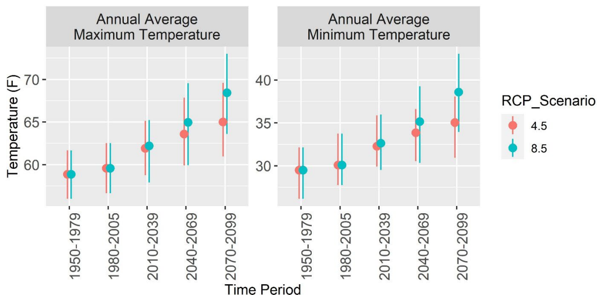
Figure 7. Modeled historical and future average minimum and maximum temperature on the Klamath National Forest summarized for 30-year periods. Points represent average while lines indicate range of data (minimum and maximum). Data source CalAdapt: see Table 4 footnote.
