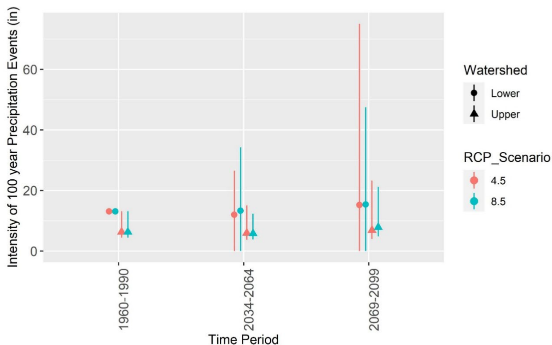
Figure 12. Modeled intensity of extreme precipitation events that on average occur every 100 years for the upper watershed (Little Shasta River) and the lower watershed (Thompson Creek-Klamath River) on the Klamath National Forest summarized for 30-year periods. Points represent average, while lines indicate the maximum upper and maximum lower 95% confidence interval. Data source CalAdapt: See Table 4 footnote.
