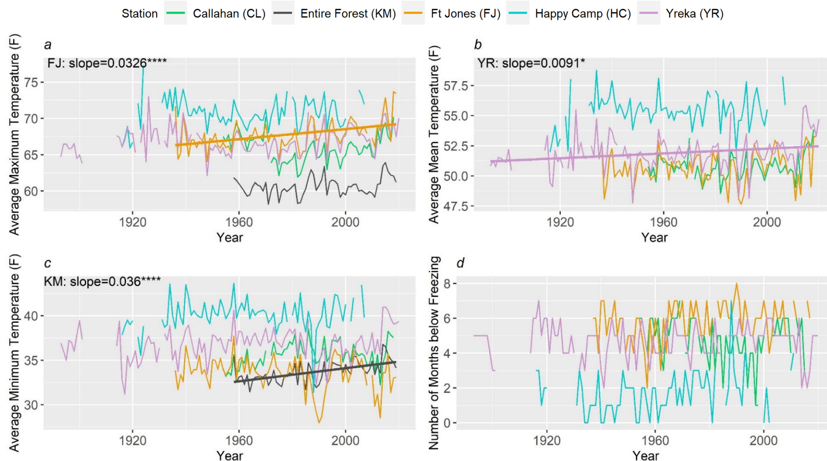
Figure 2. Historical temperature trends for the Klamath National Forest and relevant local weather stations (identified in different colors): a) Average Maximum Temperature, b) Average Mean Temperature, c) Average Minimum Temperature, and d) Number of Months below Freezing (months where the average minimum temperature was <32^{\circ}\text{F} ). Linear lines indicate a significant trend. For all significant trends the magnitude and direction of trend (slope) are presented, and the level of significance is indicated by number of asterisks (* p<0.05 , ** p<0.01 , *** p<0.001 , **** p<0.0001 ).
