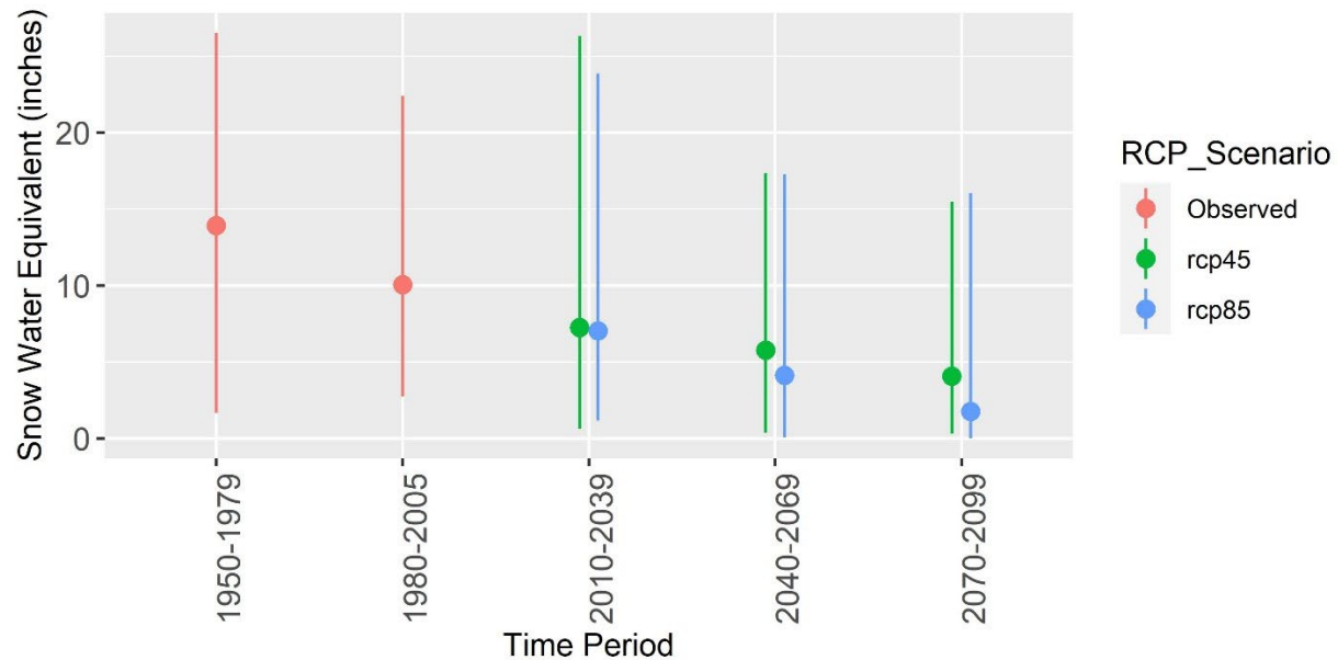
Figure 13. Historical observed and future predicted April 1 st Snow Water Equivalent (SWE) on the Klamath National Forest summarized for 30-year periods under two emission scenarios (RCP 4.5 and RCP 8.5). Points represent average while lines indicate range of data (minimum and maximum). Data source CalAdapt: See Table 4 footnote.
