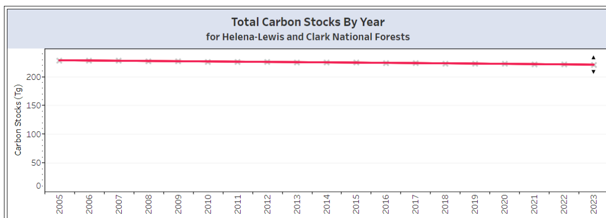
Figure 1. Total forest carbon stocks (Tg) for the years 2005 to 2023. Triangles represent a 95% confidence interval (only available for 2023).
