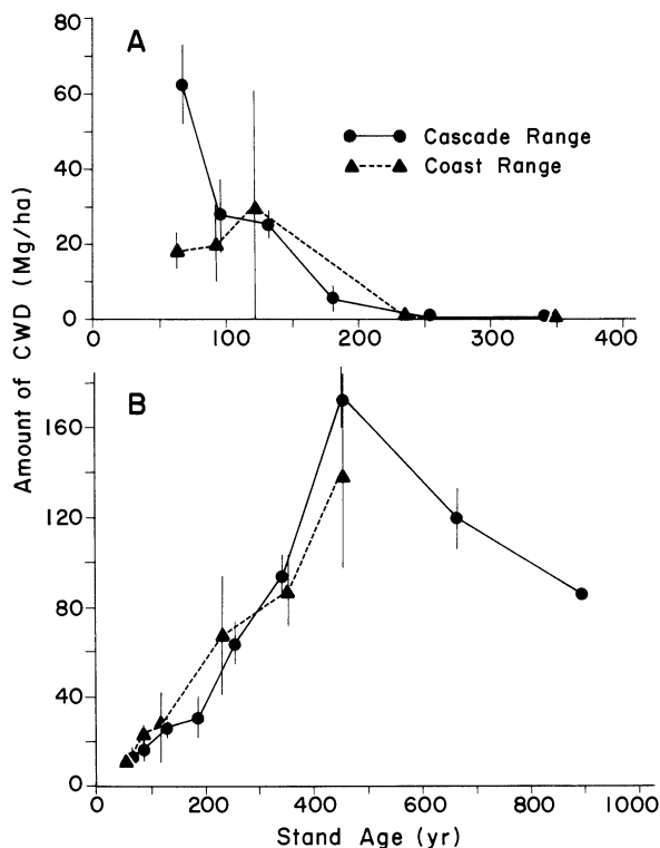
FIG. 5. Mass of total CWD originating in: (A) the preceding stand and (B) the current stand, in a chronosequence of Pseudotsuga stands in the western Cascade Range and in the southern Coast Range. Data points are plotted at age class means. Vertical bars represent standard errors.
