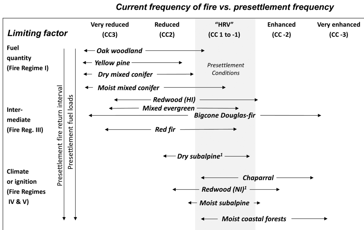
Fig. 1. Major forest ecosystems in California plus chaparral, arranged by their pre-Euroamerican settlement fire regime (y-axis; increasing from top to bottom) and the range of their current departure from presettlement fire frequencies (x-axis; departure ranges from Safford and Van de Water 2013). Locations along both axes are approximate. CC = condition class, see text and Table 1 for details. Dry subalpine and redwood NI (NI = natural ignitions, excluding human ignitions) types estimated without data from Safford and Van de Water (2013). Redwood HI = redwood forest including human ignitions. HRV = historic range of variability. Fire regime types (I, III, IV, V) from Schmidt et al. (2002).
