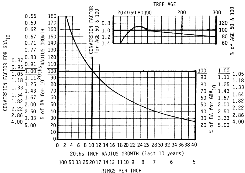
Conversion factor curves for growth basal area (Hall 1983).
