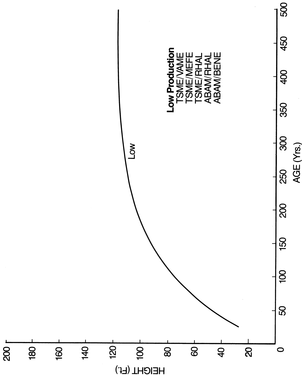
MOUNTAIN HEMLOCK HEIGHT GROWTH BY PRODUCTIVITY CLASS.
