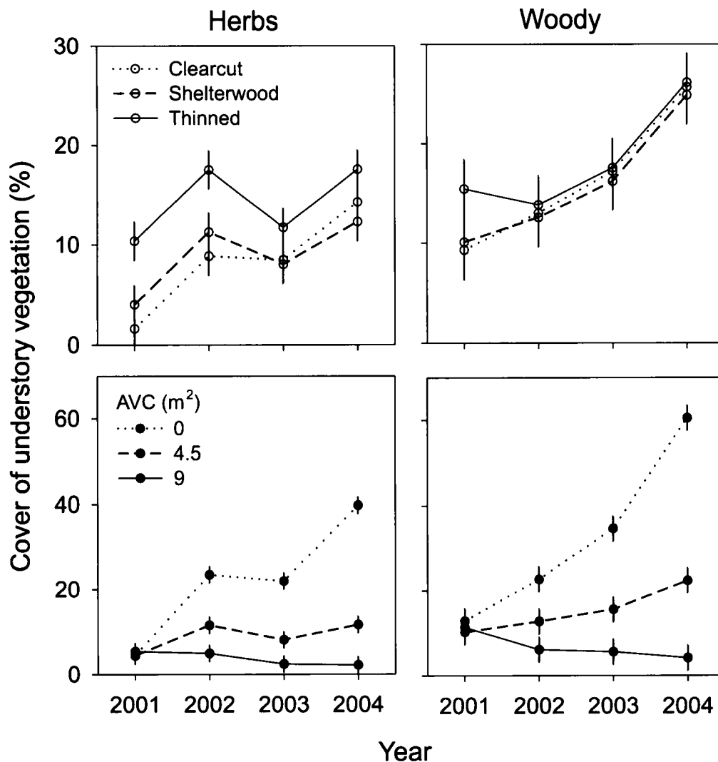
Fig. 1. Average cover of understory herbaceous and woody vegetation (with SE bars) in response to the main effects of overstory level and area of vegetation control (AVC).
