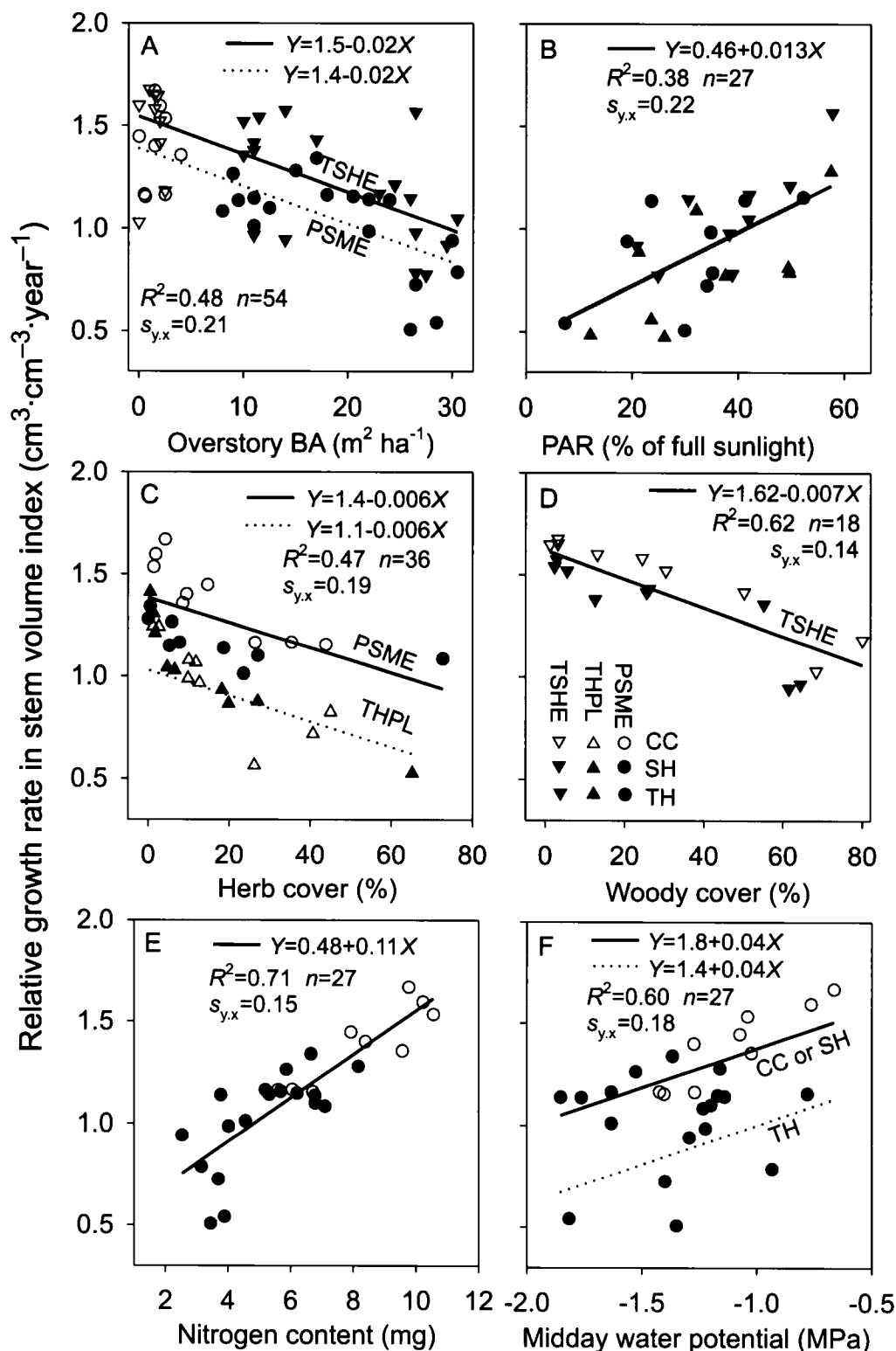
Fig. 5. Regression relationships of conifer seedling relative growth rate in stem volume index to (A) overstory basal area, (B) photosynthetically active radiation (PAR) in thinned stands, (C) herb cover, (D) woody cover, (E) Douglas-fir foliar nitrogen content, and (F) Douglas-fir midday water potential. CC, clearcut; SH, shelterwood; TH, thinned; PSME, Douglas-fir; THPL, western redcedar; and TSHE, western hemlock. Regression equations are shown with values for the coefficient of determination adjusted for degrees of freedom ( R^2 ), sample size ( n ), and standard error of estimate ( s_{y,x} ). Legend in (D) indicates symbols for species and overstory levels.
