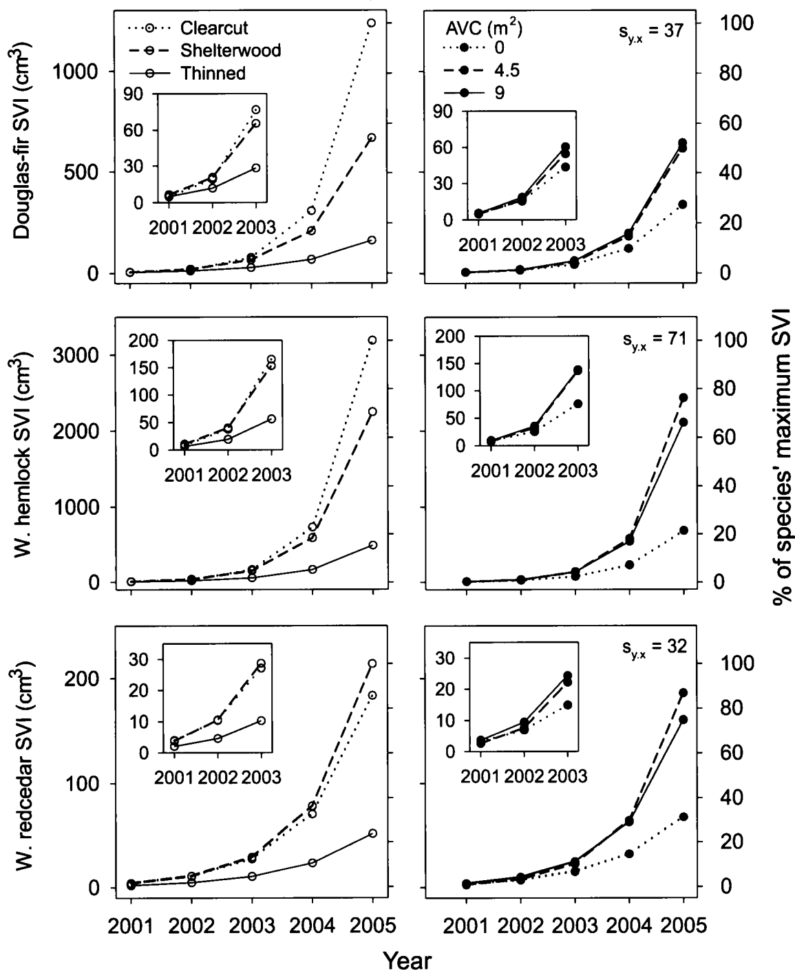
Fig. 2. Predicted average stem volume index (SVI) of Douglas-fir, western hemlock, and western redcedar in response to the main effects of overstory level and area of vegetation control (AVC). S_{y,x} is the standard error of estimate.
