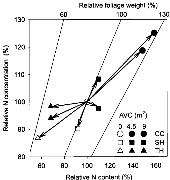
Fig. 4. Relative responses of Douglas-fir foliage dry mass, nitrogen concentration, and nitrogen content to the combined effects of overstory level and area of vegetation control (AVC). CC, clearcut; SH, shelterwood; TH, thinned. Plotted values are expressed relative to the reference treatment (seedlings in clearcuts with 0 m 2 AVC) and vectors (arrows) indicate the magnitude of responses to overstory level and AVC.
