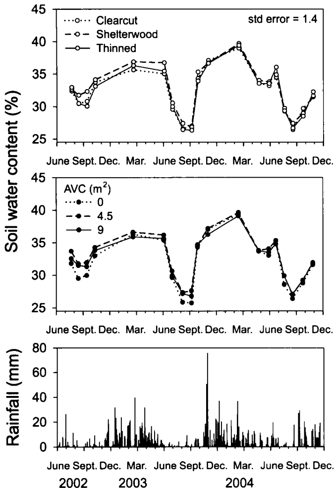
Fig. 3. Average volumetric soil water content at 0–12 cm depth in response to the main effects of overstory level and area of vegetation control (AVC).
