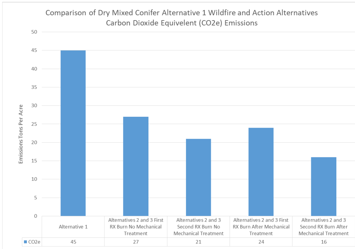
Figure 9. Comparison of Alternative 1 dry mixed conifer estimated greenhouse gas emissions to the action alternatives estimated emissions for mixed conifer (tons per acre)
