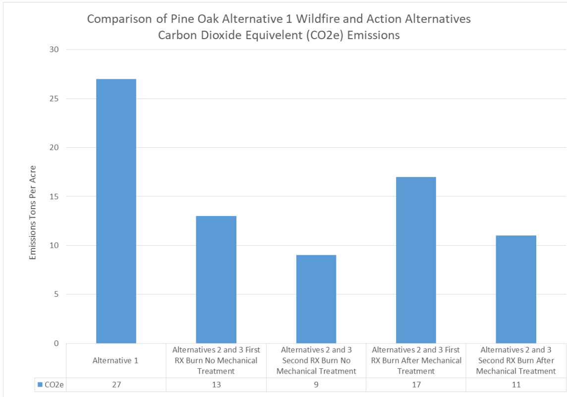
Figure 10. Comparison of Alternative 1 pine oak estimated greenhouse gas emissions to the action alternatives estimated emissions for pine oak (tons per acre)
