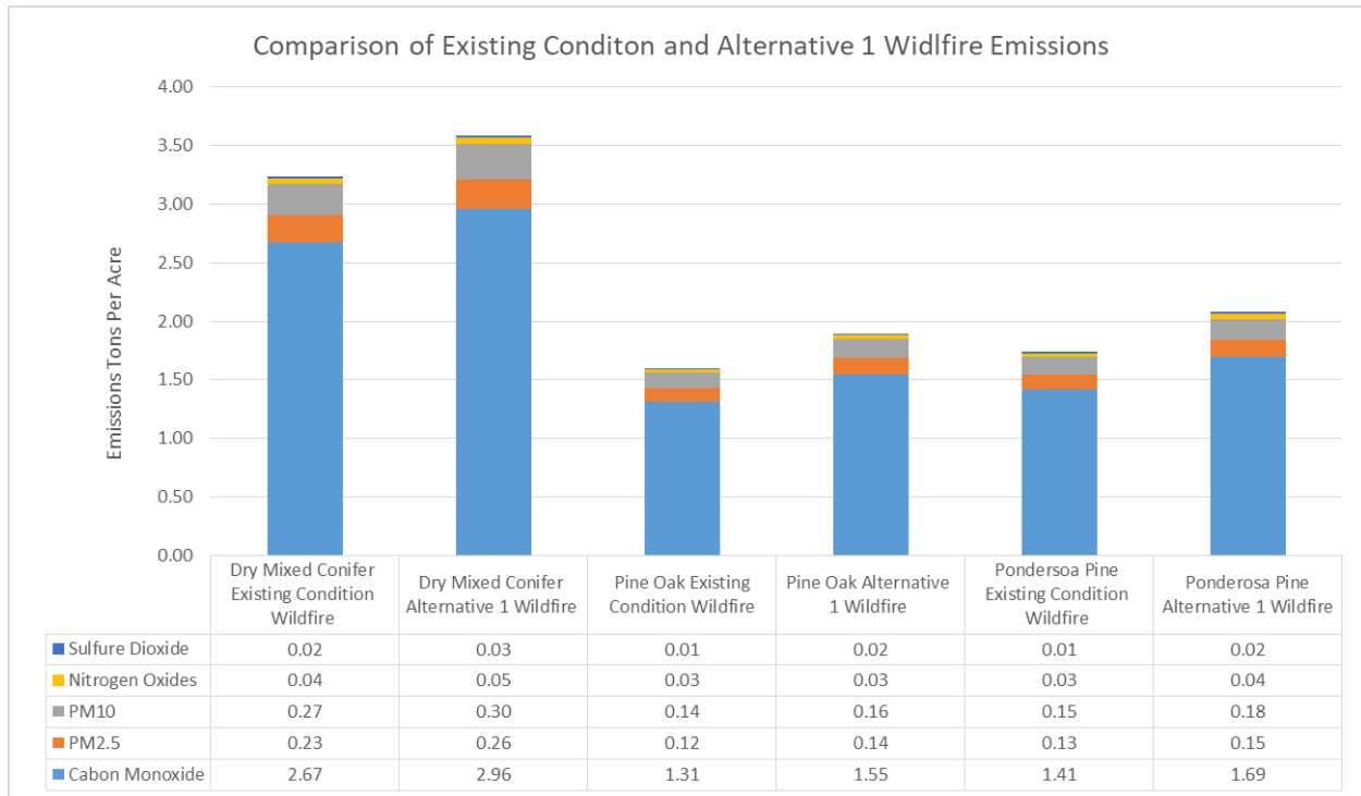
Figure 4. Existing condition (2018) wildfire smoke criteria air pollutant emissions and Alternative 1 (2029) wildfire emissions for dry mixed conifer, pine oak and ponderosa pine ecological response units (tons per acre)
