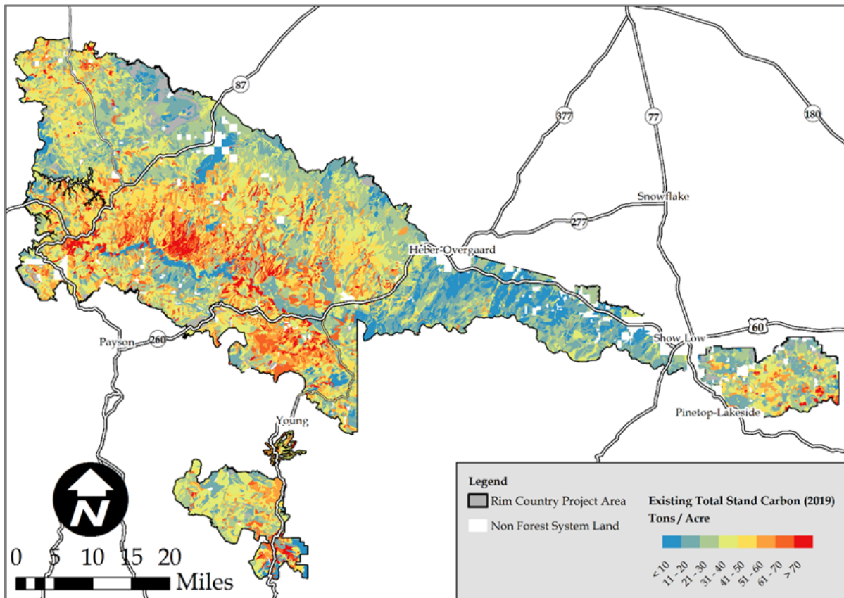
Figure 14. Total estimated above and below ground sequestered carbon in 2019 for the Rim Country project area
