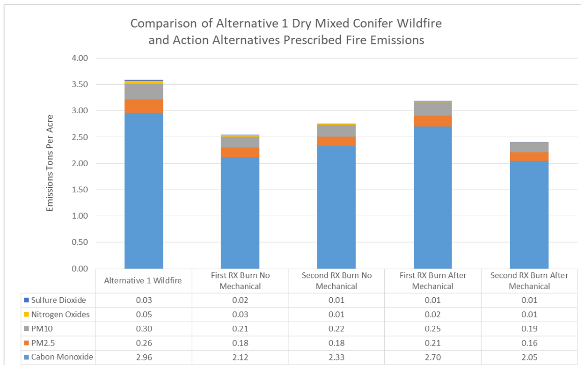
Figure 6. Comparison of Alternative 1 estimated criteria air pollutant emissions to the action alternatives estimated emissions for dry mixed conifer (tons per acre)
