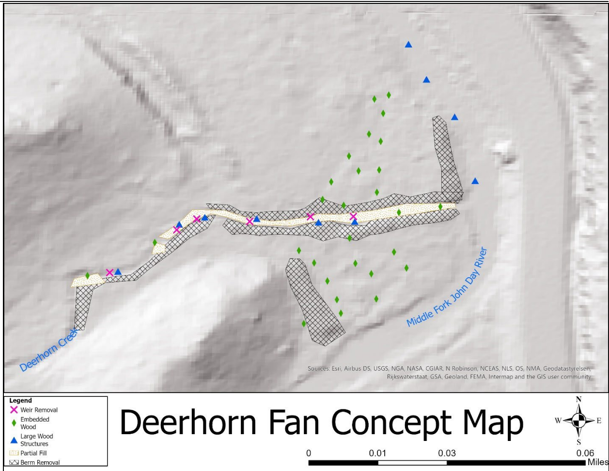
Figure 7. The concept design for the Deerhorn Creek fan at the confluence with the Middle Fork. Designs show locations of log weir removal, embedded wood in the floodplain, locations for large wood structures, berm removal, and partial channel fill.
