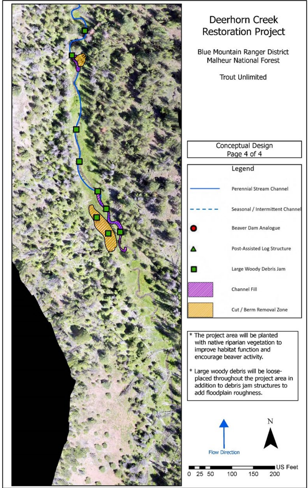
Figure 6. Conceptual map of design for the final quarter mile of Deerhorn Creek. Exact locations of features are subject to change to during implementation for a field fit design. Design includes beaver dam analog, post assisted log structures, large woody debris jams, berm removal zones, and partial fill zones.
