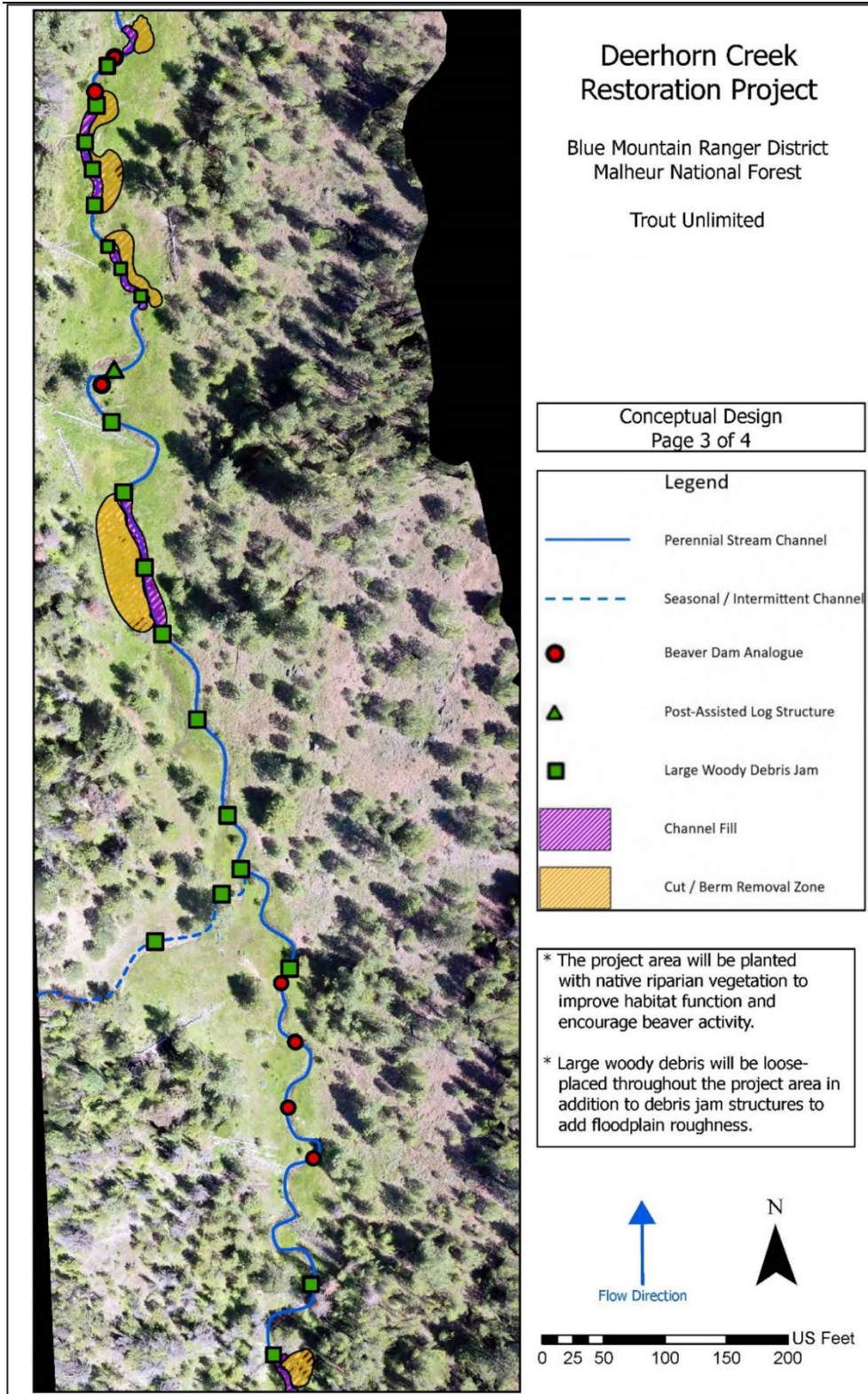
Figure 5. Conceptual map of design for the third quarter mile of Deerhorn Creek. Exact locations of features are subject to change to during implementation for a field fit design. Design includes beaver dam analogue, post assisted log structures, large woody debris jams, berm removal zones, and partial fill zones.
