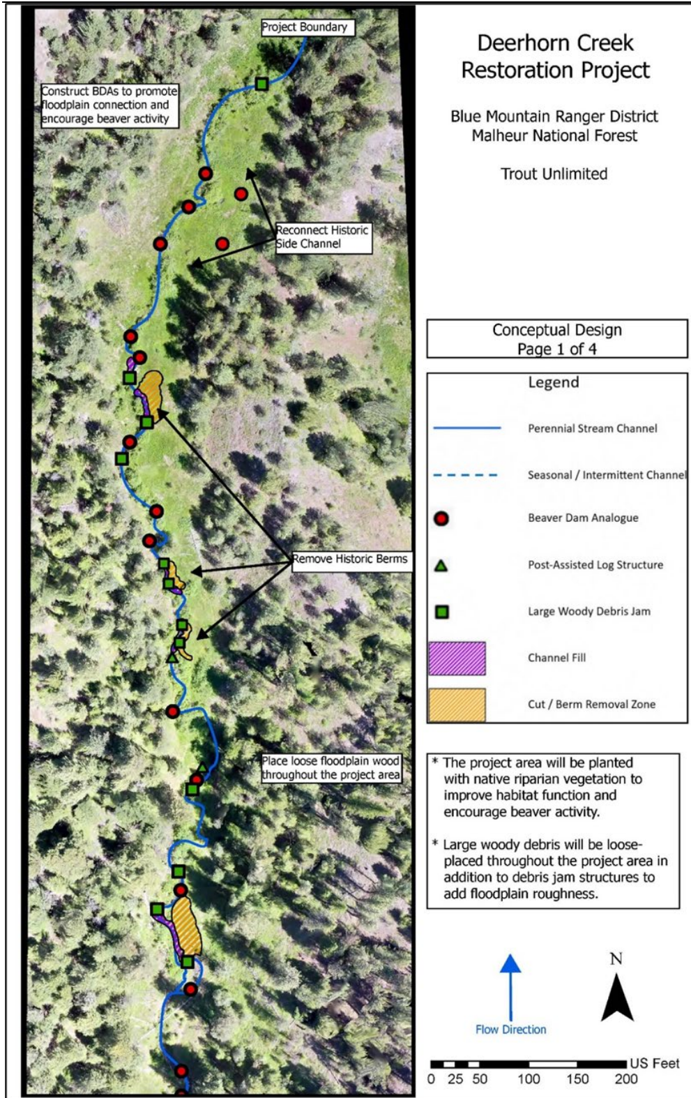
Figure 3. Conceptual map of design for the first quarter mile of Deerhorn Creek. Exact locations of features are subject to change to during implementation for a field fit design. Design includes beaver dam analogue, post assisted log structures, large woody debris jams, berm removal zones, and partial fill zones.
