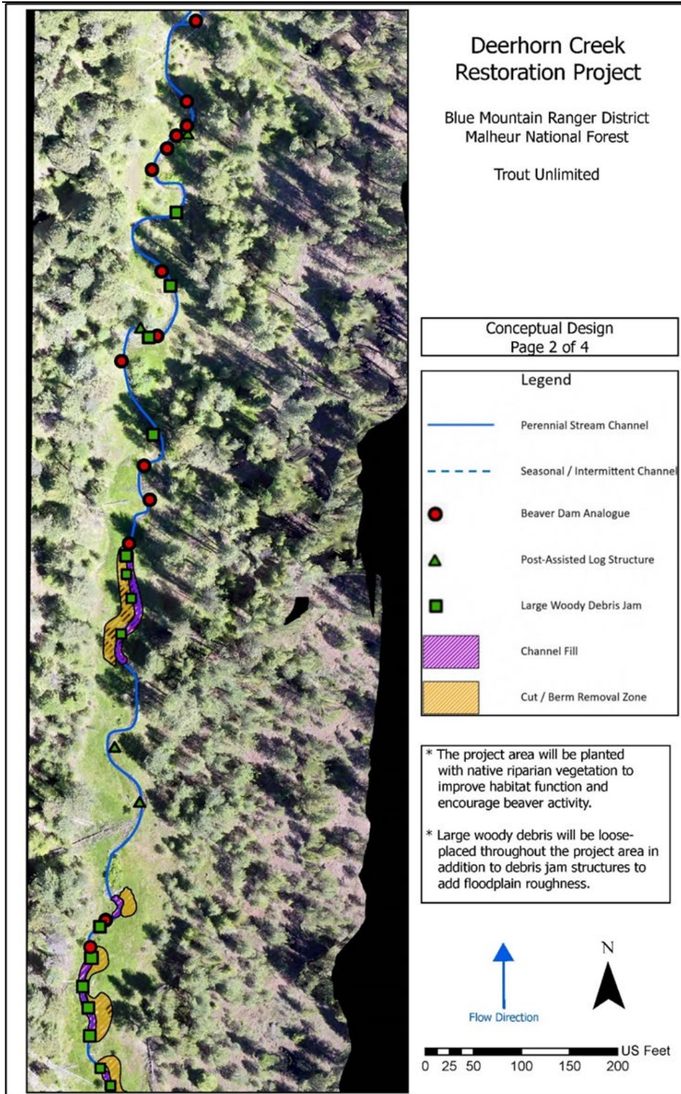
Figure 4. Conceptual map of design for the second quarter mile of Deerhorn Creek. Exact locations of features are subject to change to during implementation for a field fit design. Design includes beaver dam analog, post assisted log structures, large woody debris jams, berm removal zones, and partial fill zones.
