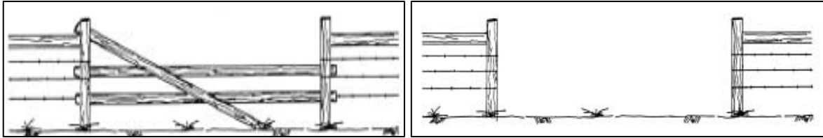
Figure 5. Wildlife jump or gates made of corral poles stacked parallel to the ground. Vertical poles should not be less than 12 feet apart. One or more poles can be removed to allow for easy passage (Hanophy 2009).
