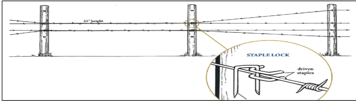
Figure 2. Adjustable fence to allow for wildlife passage around high quality habitats, on steep slopes, swales, gullies, ridges and when livestock are not present (Hanophy 2009).
