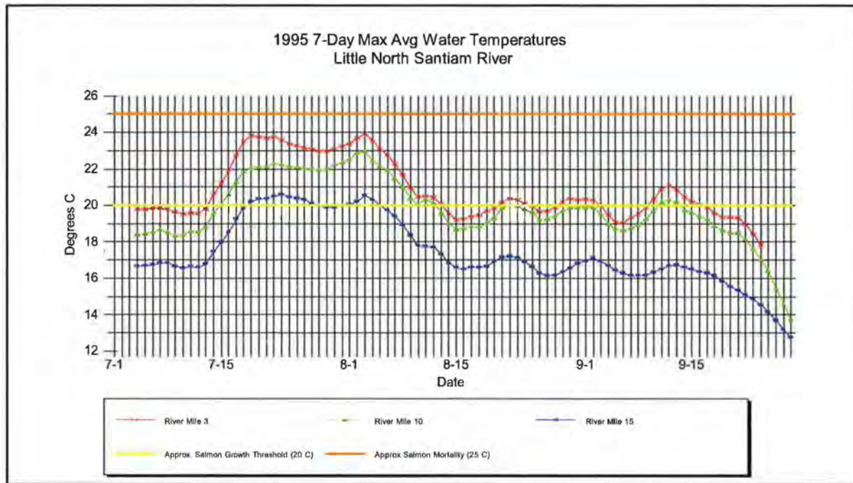
Figure 18 . 1995 Seven Day Maximum Average Water Temperatures
