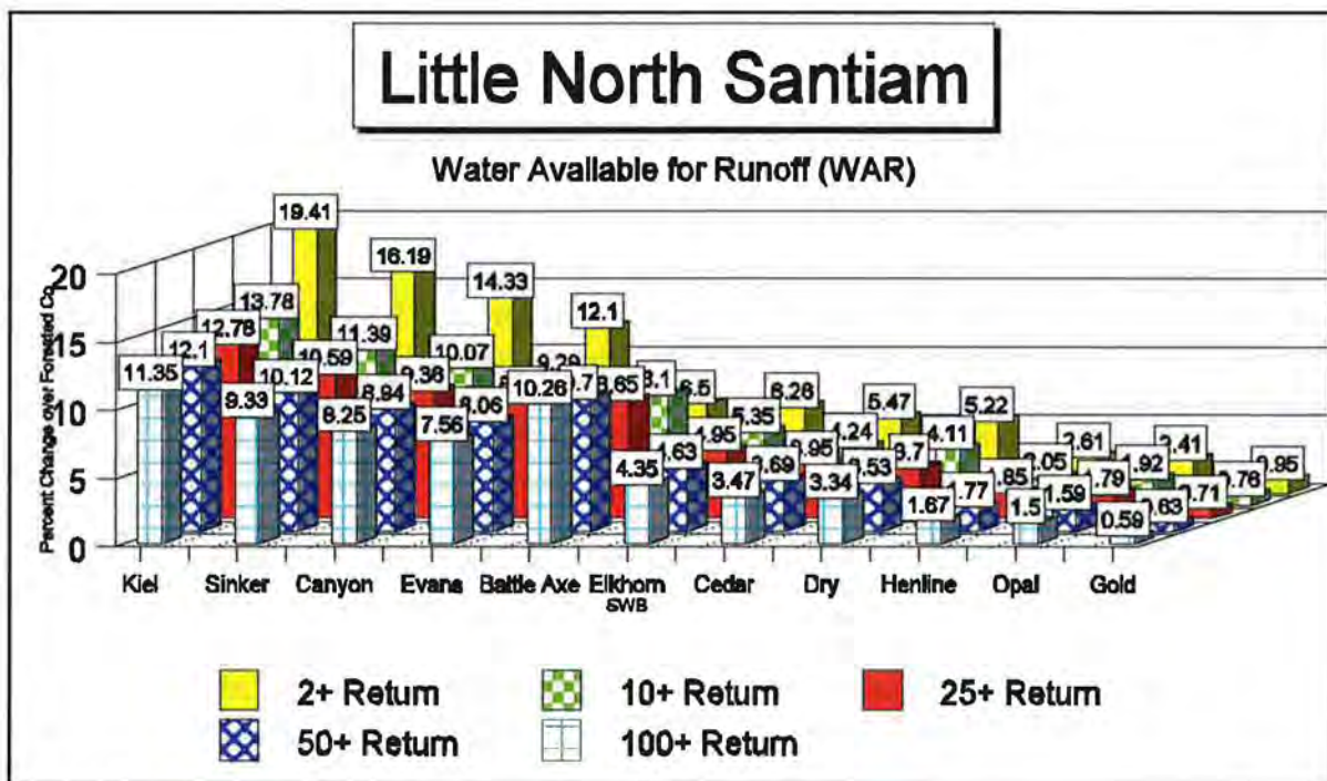
Figure 21. Water Available for Runoff.
