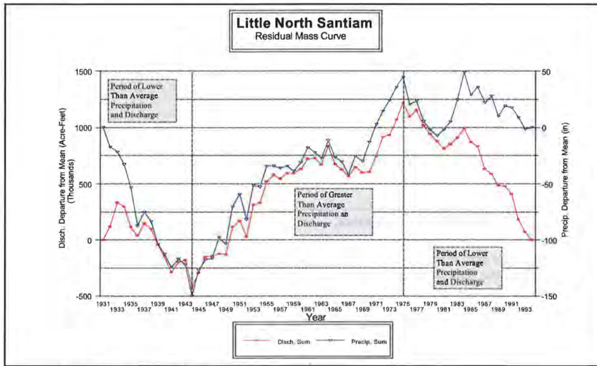
Figure 14.. Residual Mass Curves.
