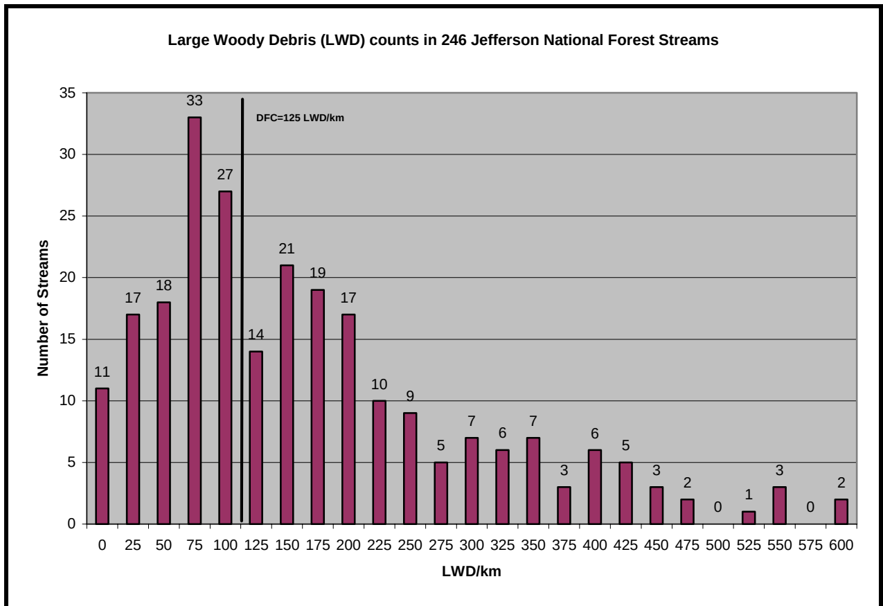
Figure 3-4. Large Woody Debris (LWD) counts in Jefferson National Forest Streams
