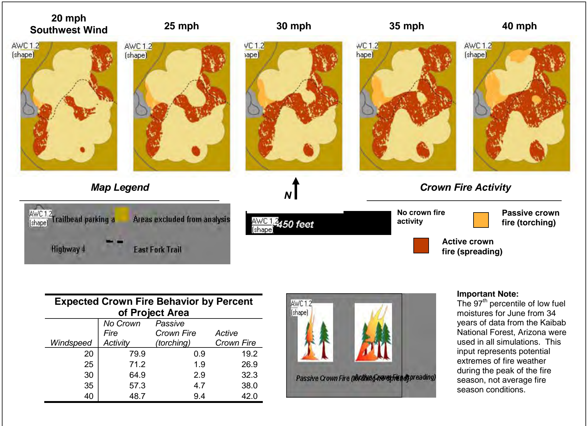
Figure 3: FlamMap Simulated Crown Fire Behavior: East Fork Project Area
