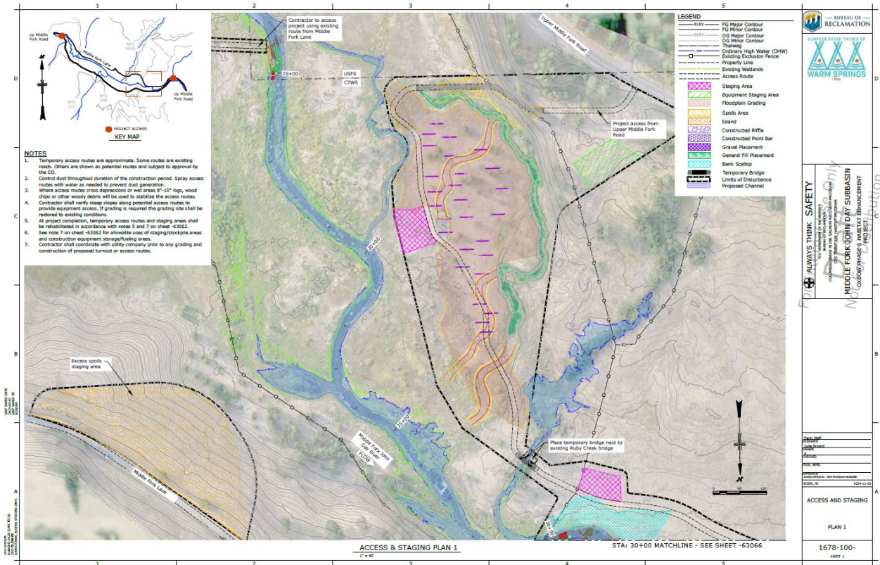
Figure 5. Proposed Conditions for the Upper Project Area.
