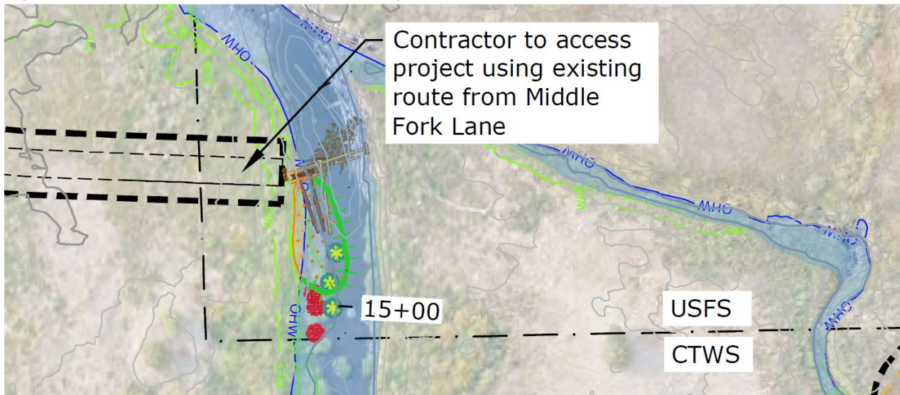
Figure 6. Proposed Conditions for the Forest Service Section of the Project Area.
