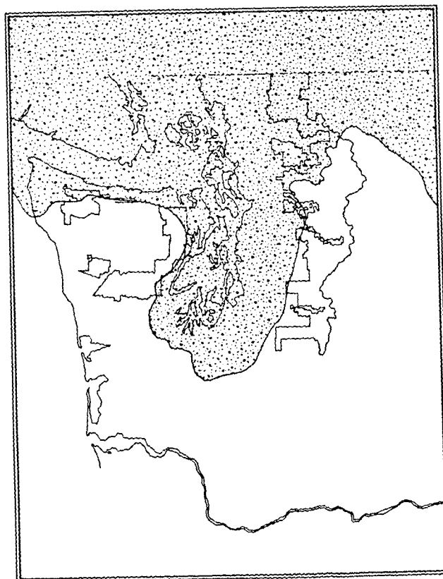
Figure 16. Map of the extent of glaciation during the Vashon Stade (adapted from Armstrong et al. 1965).
