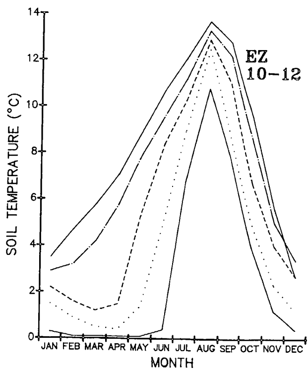
Figure 29. Soil temperature profiles (20 cm depth) by elevation band for environmental zone groups.
