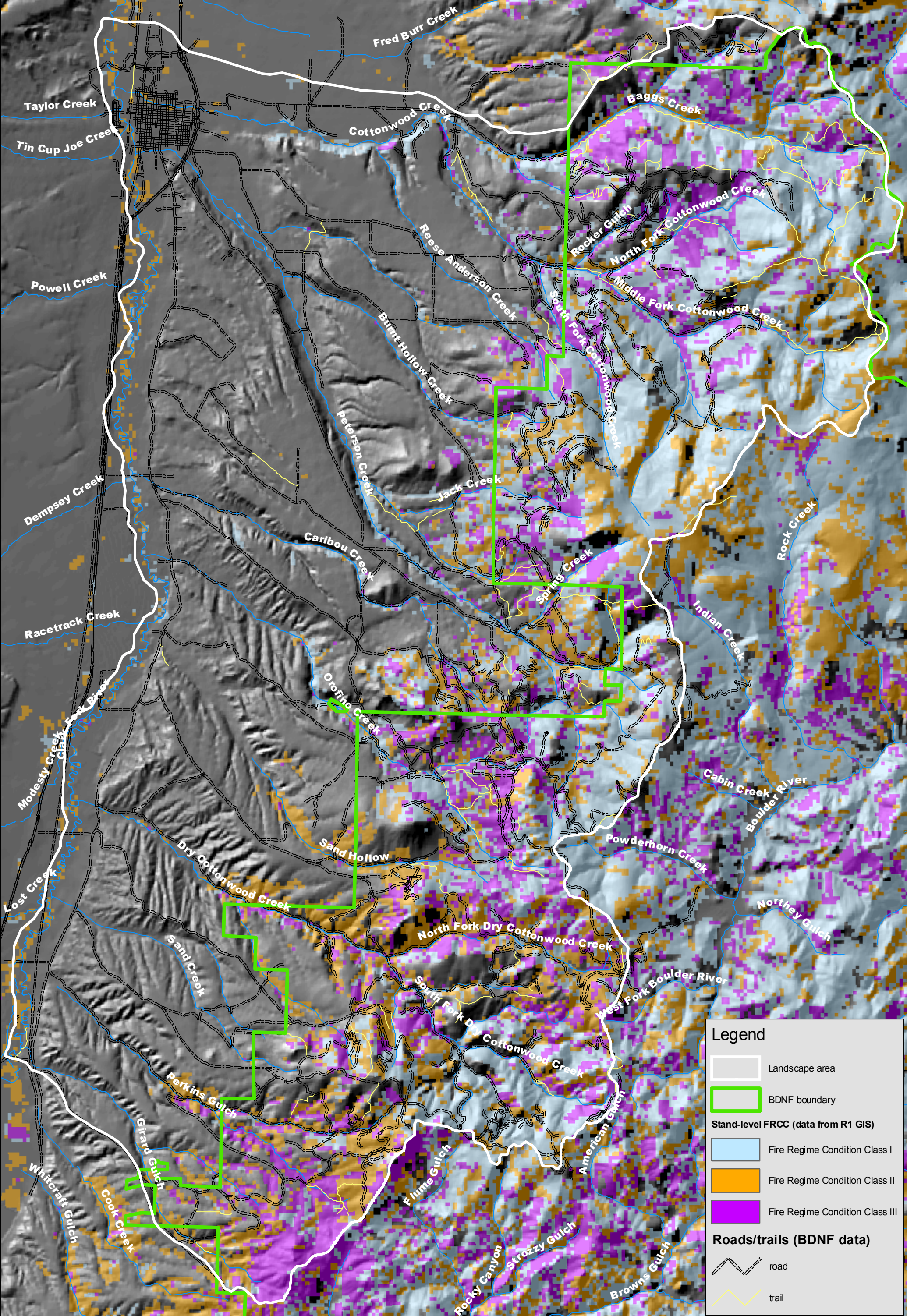
Figure IIC-6 Stand-level Fire Regime Condition Class FRCC not calculated for non-forest vegetation.
