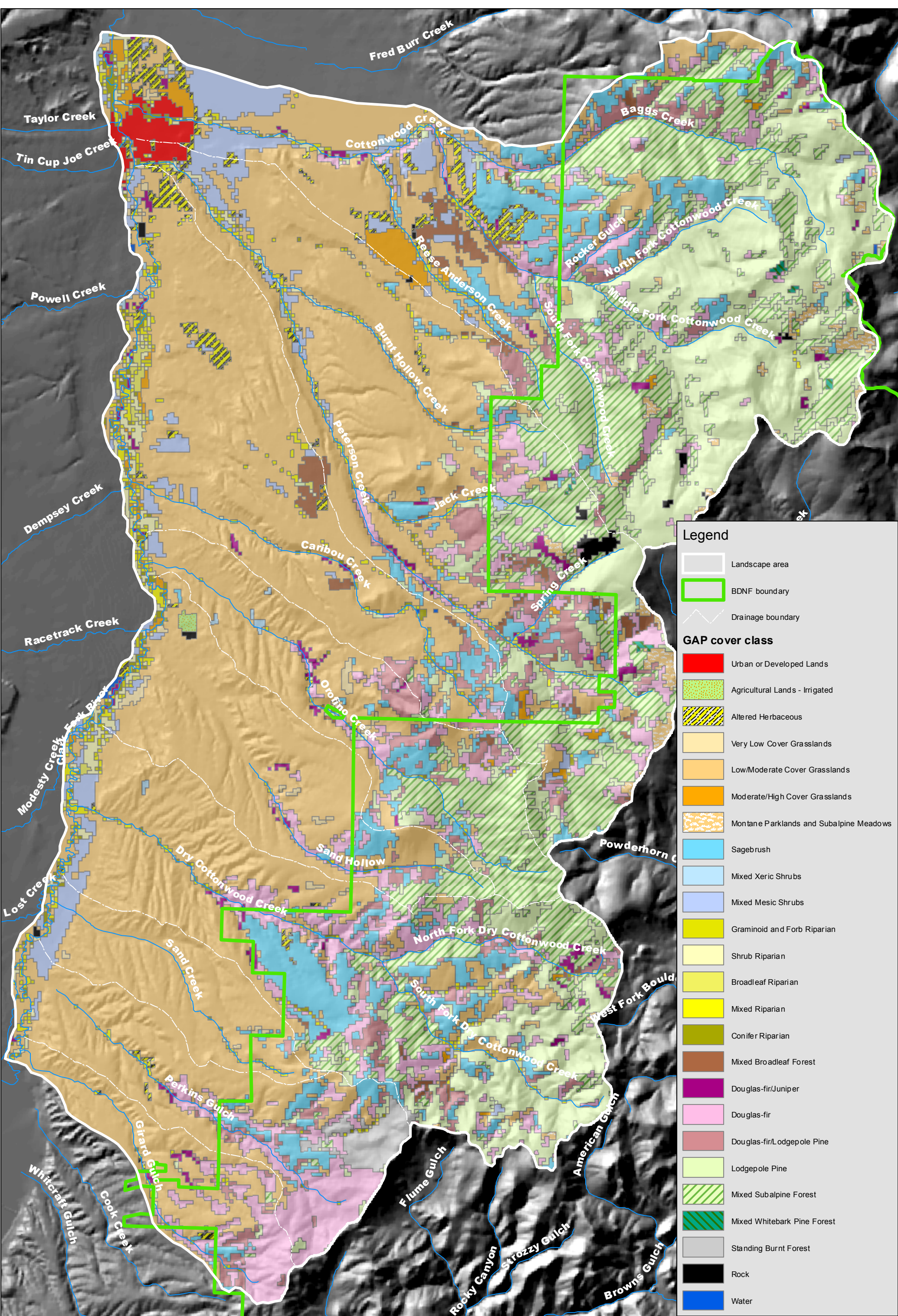
Figure IA-3 GAP Land Cover Classification
