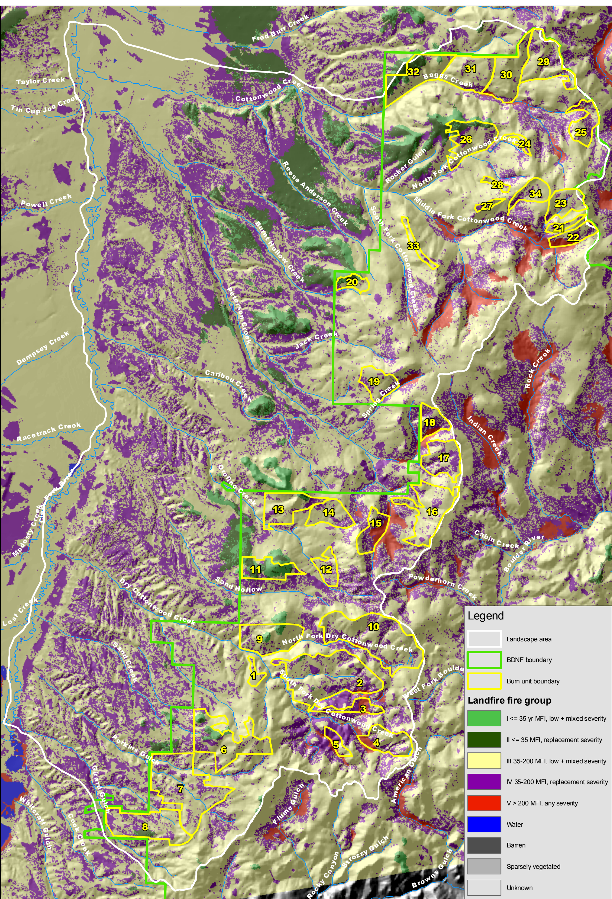
Figure IIC-11 Fire Regime Group and Burn Units (Landscape fire succession model LANDSUM)
