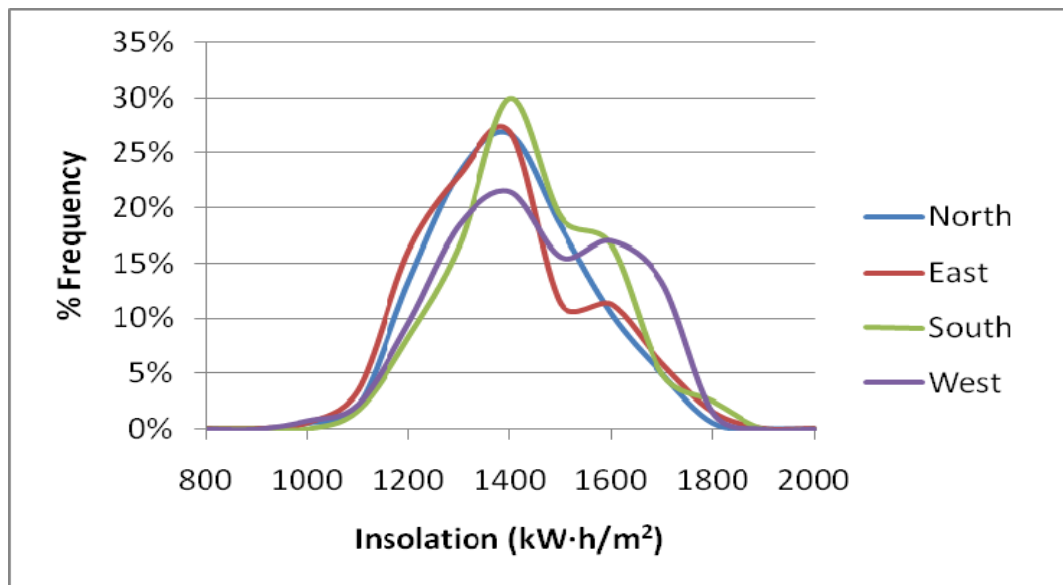
Figure 17: Relationship between mean insolation and aspect for all 660 rock glaciers. Mean insolation values (kW·h/m²) for each respective orientation were: North (1346), East (1340), South (1388), and West (1397).
