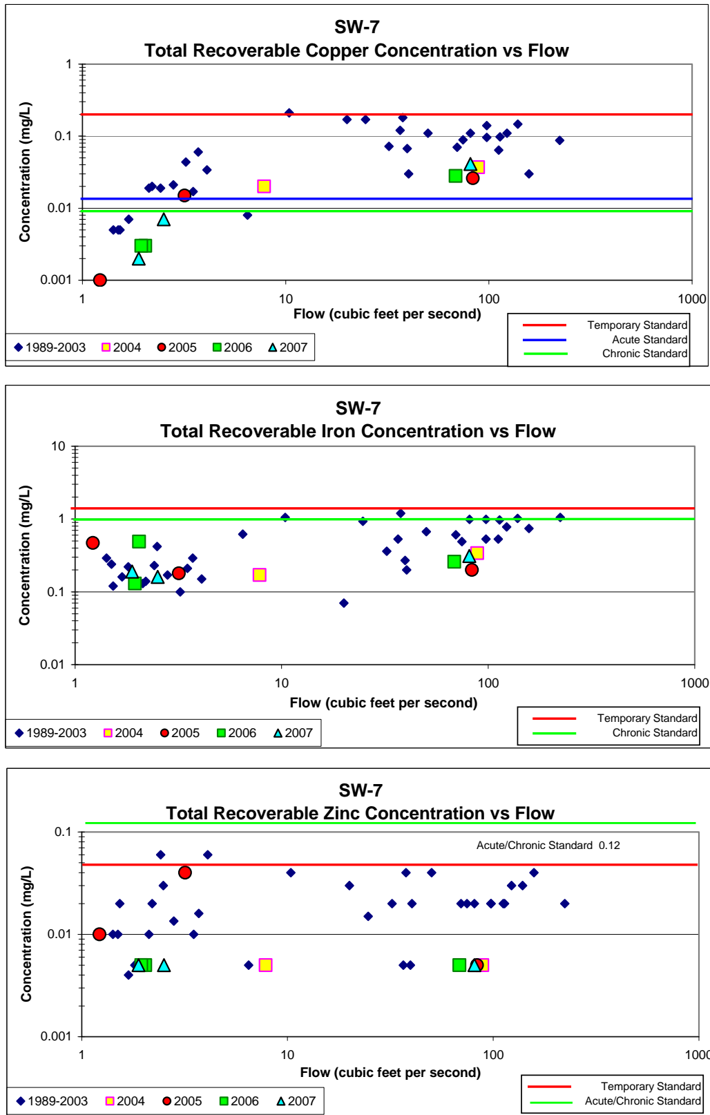
Figure 9 - Concentration vs. Flow Graphs for Station SW-7
