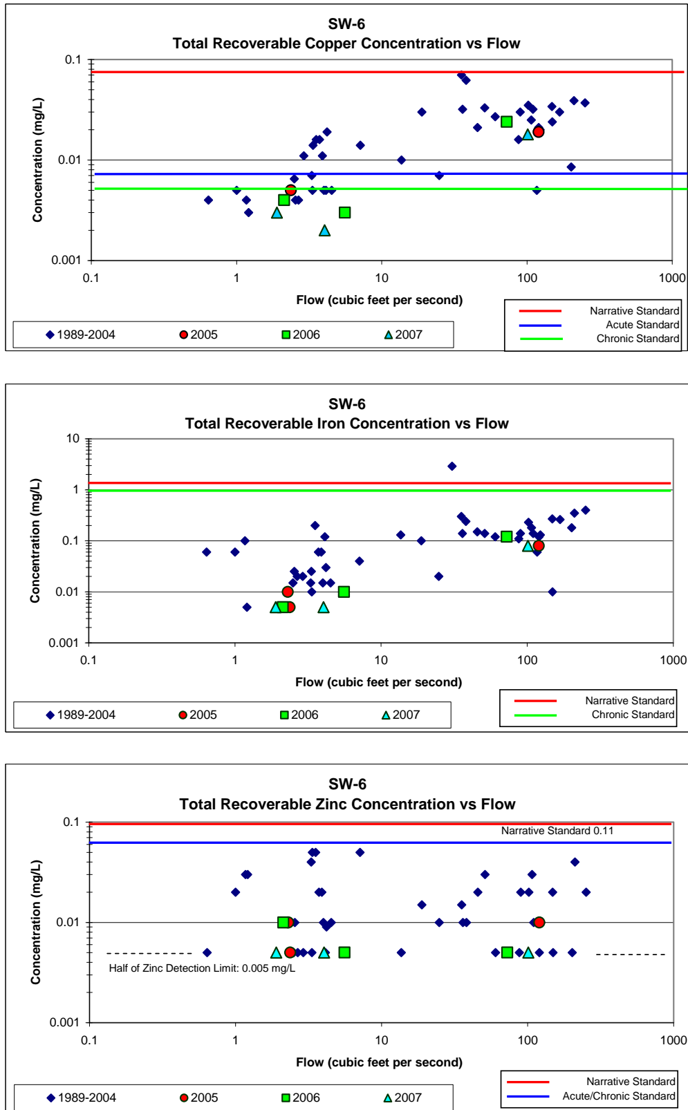
Figure 6 - Concentration vs. Flow Graphs for Station SW-6
