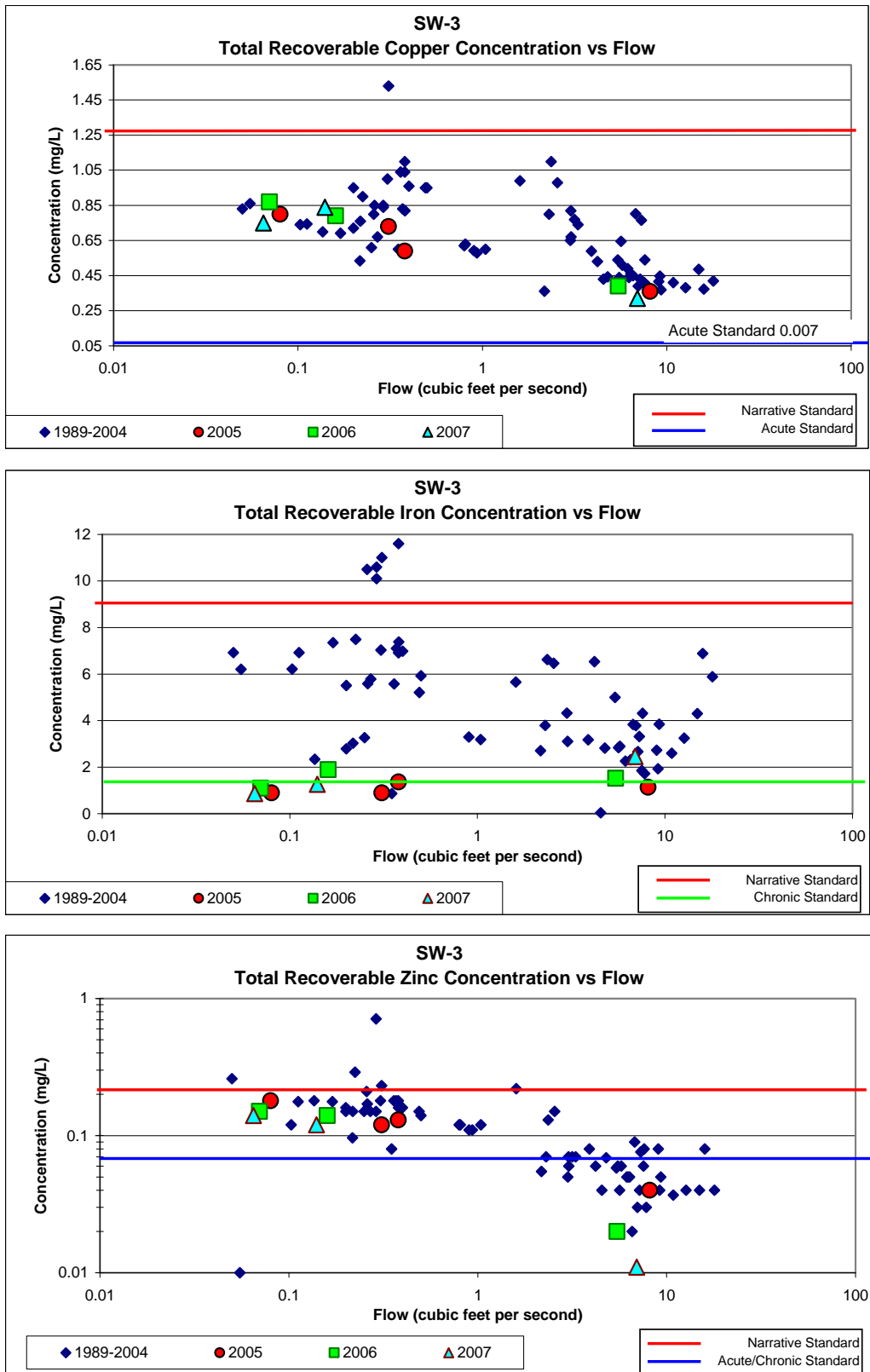
Figure 3 - Concentration vs. Flow Graphs for Station SW-3
