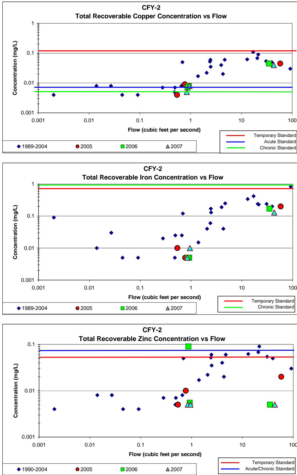
Figure 5 - Concentration vs. Flow Graphs for Station CFY-2
