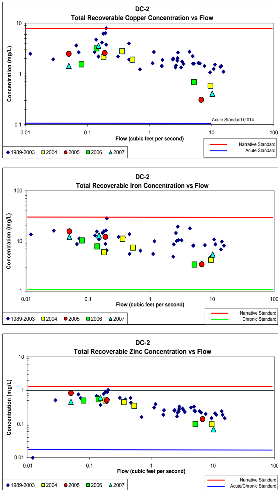
Figure 7 - Concentration vs. Flow Graphs for Station DC-2
