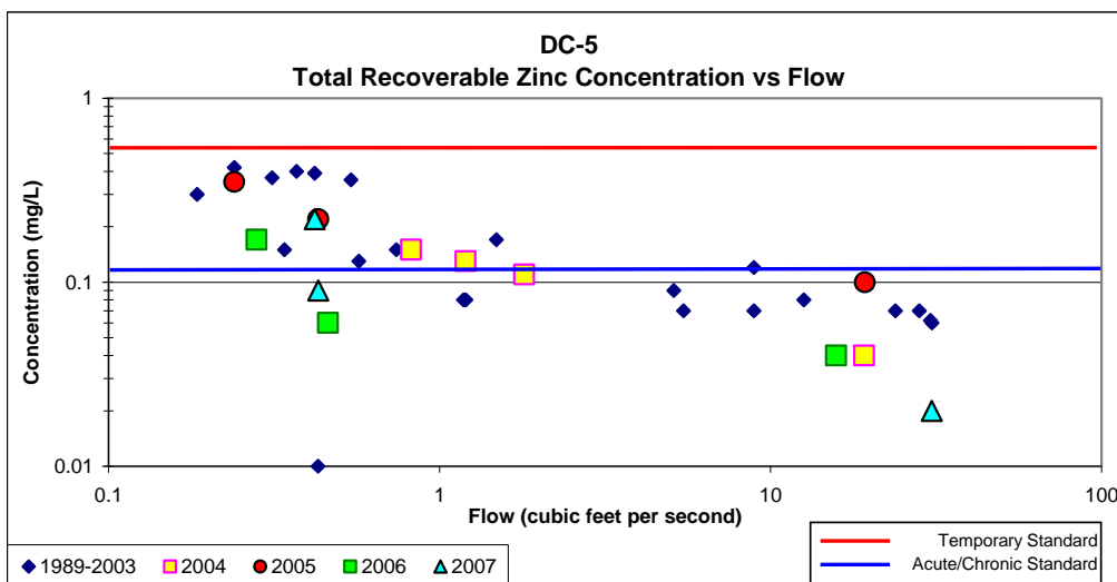
Figure 8 - Concentration vs. Flow Graphs for Station DC-5
