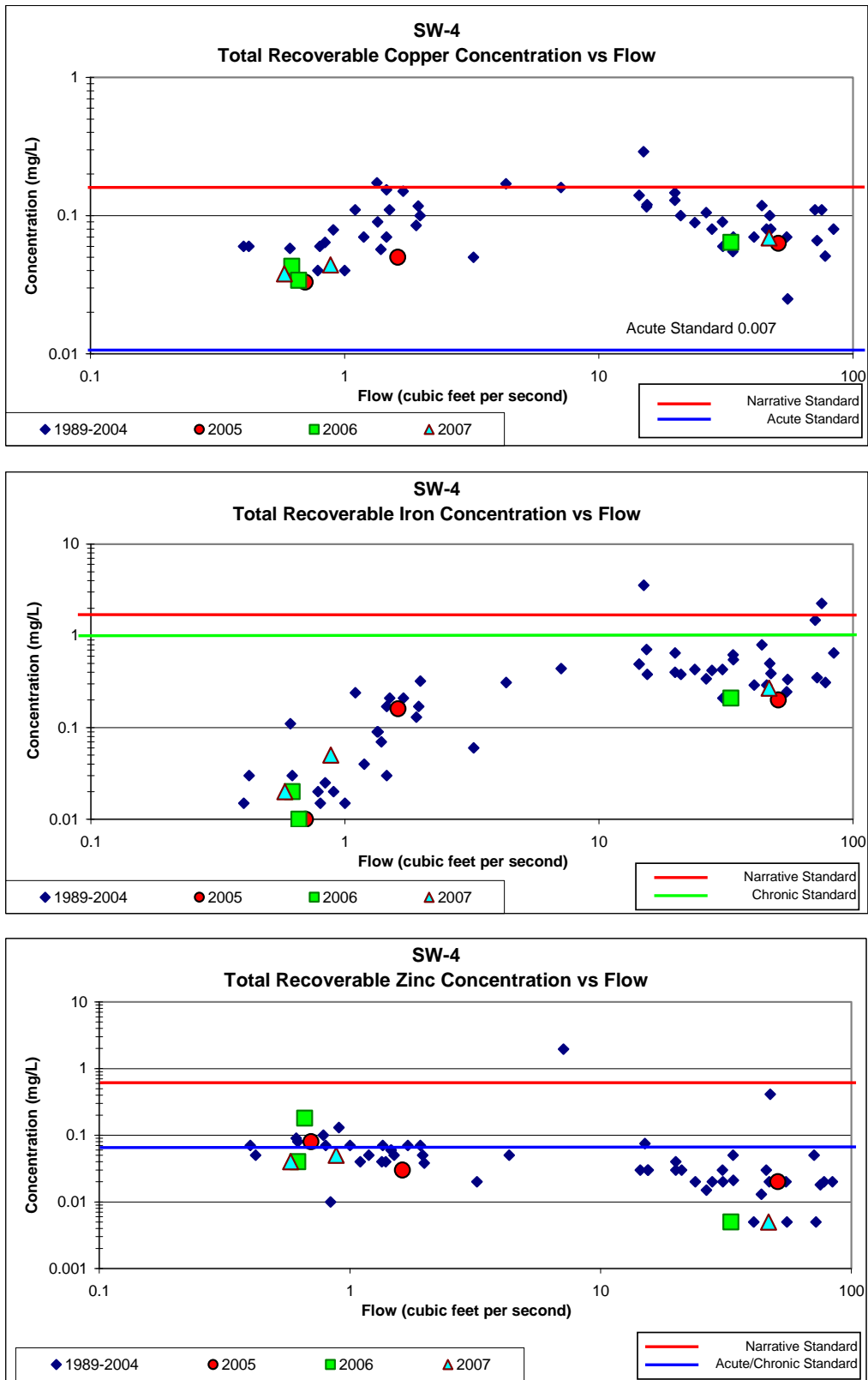
Figure 4 - Concentration vs. Flow Graphs for Station SW-4
