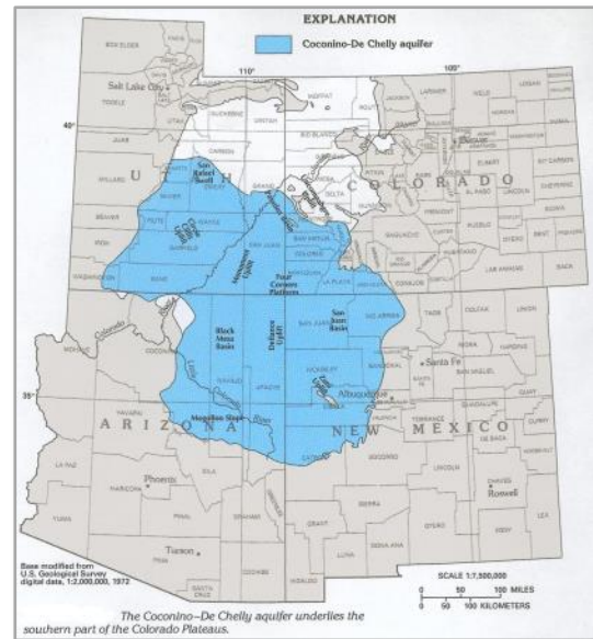
Figure 10. Map showing extent of the Coconino-De Chelly Aquifer (C Aquifer).
