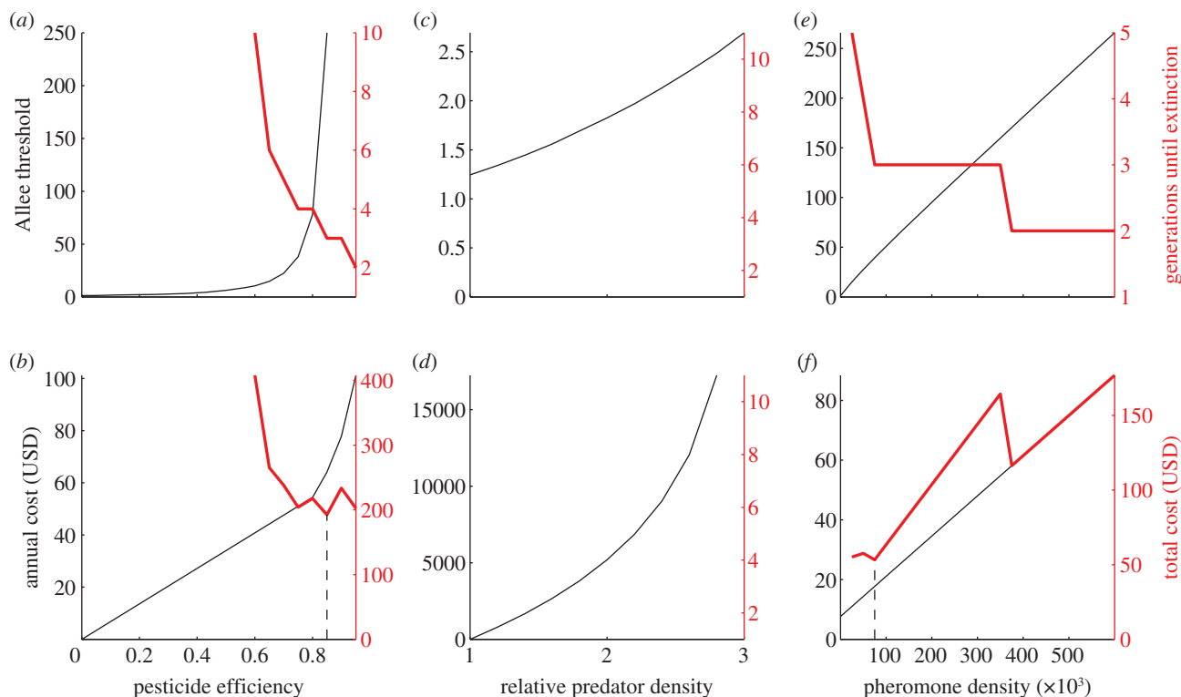
Figure 1. Changes in the Allee threshold after implementing a single control tactic alone. (a,c,e) The top row of figures shows the Allee threshold versus intensity of a particular control tactic (in black) in addition to the number of generations until eradication with an initial number of egg mass of 10 (in red). (b,d,f) The second row shows the annual costs of achieving that level of effectiveness (black) and the total costs that account for generations until eradication (red). When applicable, the vertical dashed line represents the optimal level of a particular control tactic. From left to right, the figures correspond to pesticide application, predator augmentation and mating disruption.
