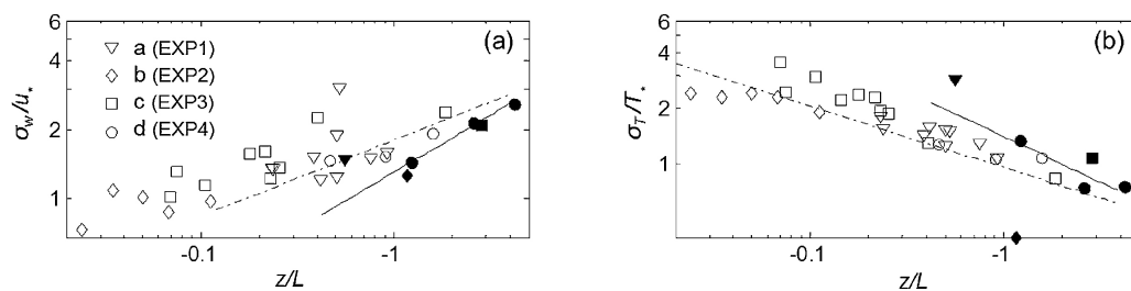
Fig. 2. (a) Normalized \sigma_w and (b) normalized \sigma_T as functions of z/L in unstable conditions. The hollow symbols indicate pre- and post-FFP data and the solid symbols indicate during-FFP data. The dashed line of the 1/3 slope \phi_w = 1.9 in (a) and -1/3 slope \phi_T = 0.95 in (b) are the local free convection prediction shown in Wyngaard et al. (1971). The solid black line represents 1/2 slope with \phi_w = 1.3 in (a) and -1/2 slope \phi_T = 1.4 in (b).
