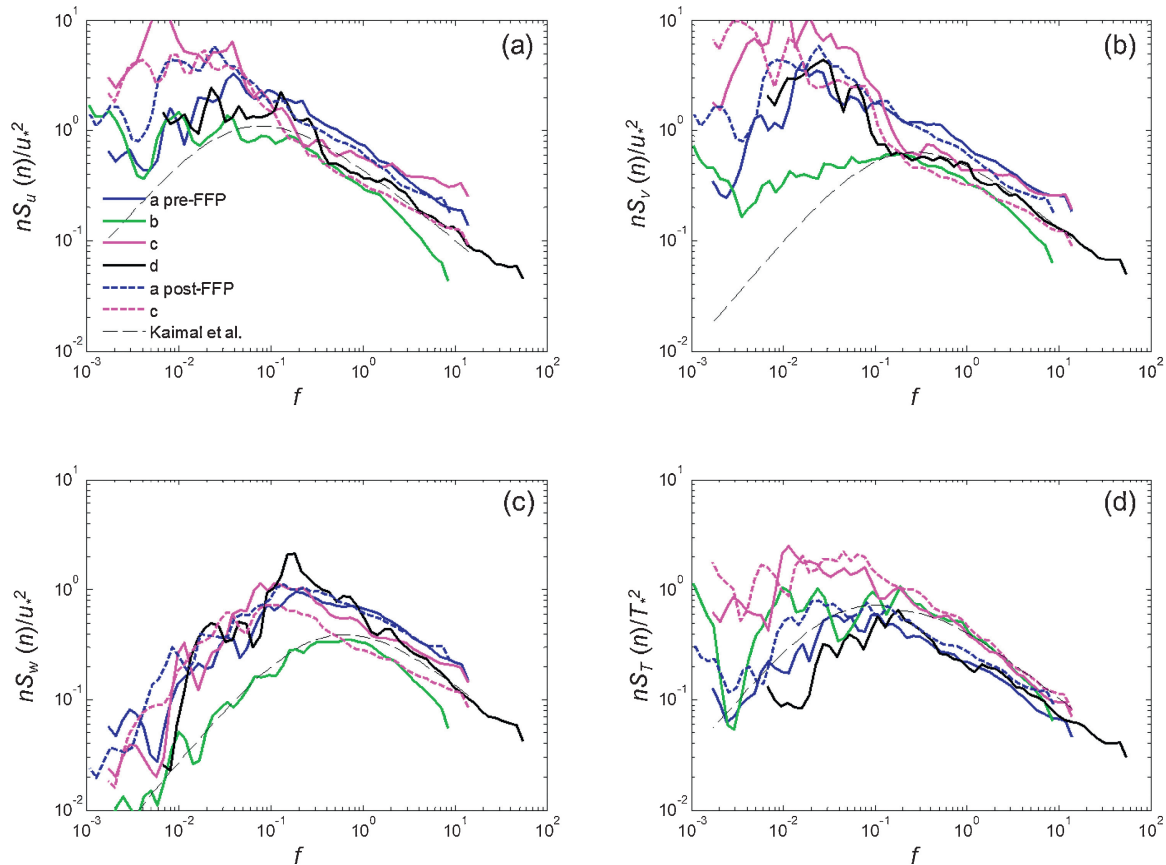
Fig. 8. Normalized spectra of velocity components and temperature observed before and after the FFP during the four experiments: (a) for u ; (b) for v ; (c) for w ; and (d) for T as a function of the normalized frequency, f = nz/U . The dashed lines in the plots indicate the velocity and temperature spectra for neutral stability obtained by Kaimal et al. (1972).
