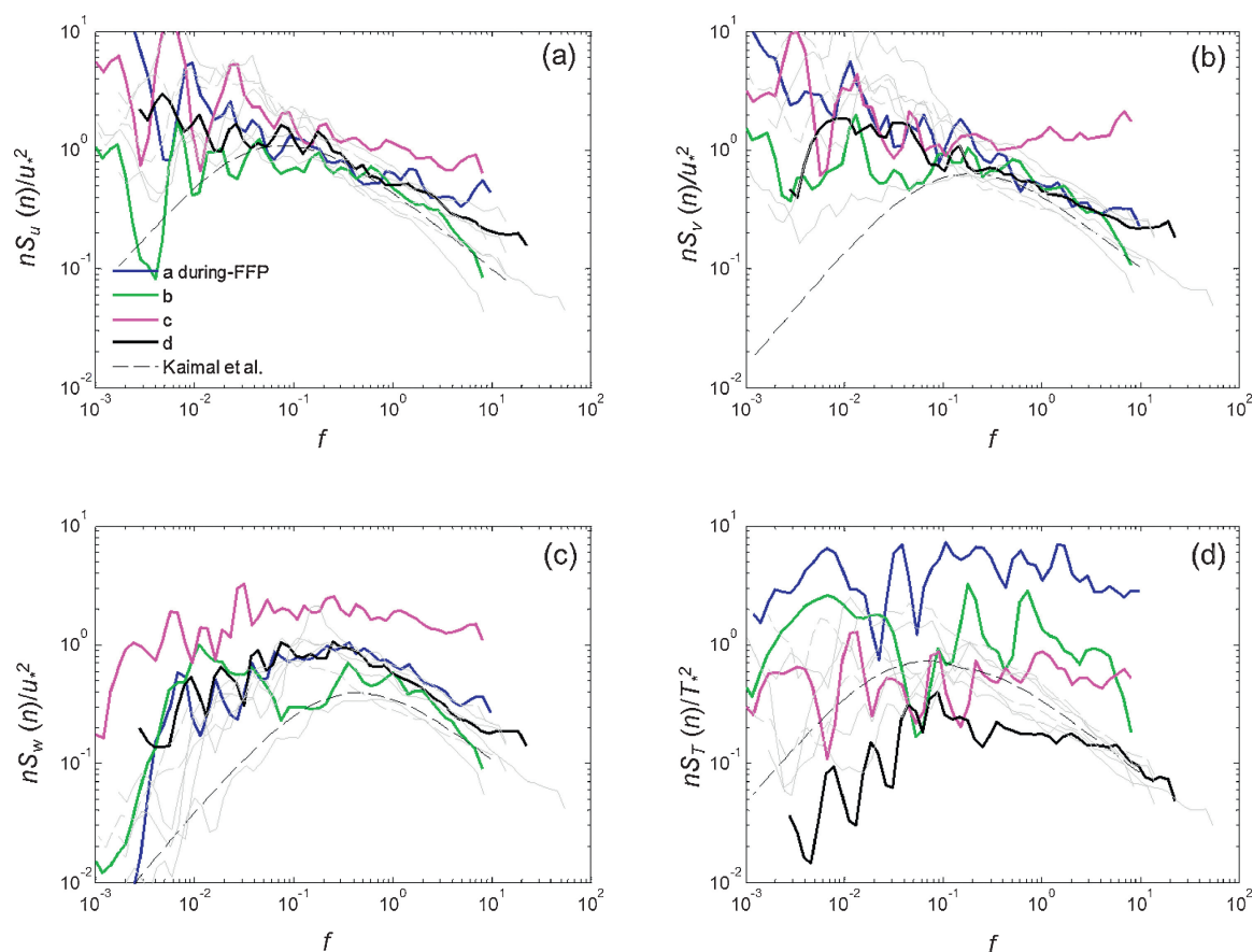
Fig. 9. Normalized spectra of velocity components and temperature observed during FFP for each experiment: (a) for u ; (b) for v ; (c) for w ; and (d) for T as a function of the normalized frequency, f = nz/U . The dashed lines in the plots indicate the velocity and temperature spectra for neutral stability obtained by Kaimal et al. (1972). The pre- and post-FFP spectra shown in Fig. 8 are plotted with light gray color in the background.
