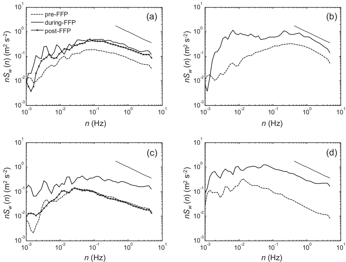
Fig. 6. Non-normalized power spectra of the vertical wind velocity nS_w(n) as a function of the natural frequency n for the experimental burns (a)–(d) as shown in Fig. 1. Short line represents -2/3 slope of inertial subrange. Pre-, during-, and post-FFP spectra are shown in blue, red, and black, respectively. (For interpretation of the references to color in this figure legend, the reader is referred to the web version of the article.)
