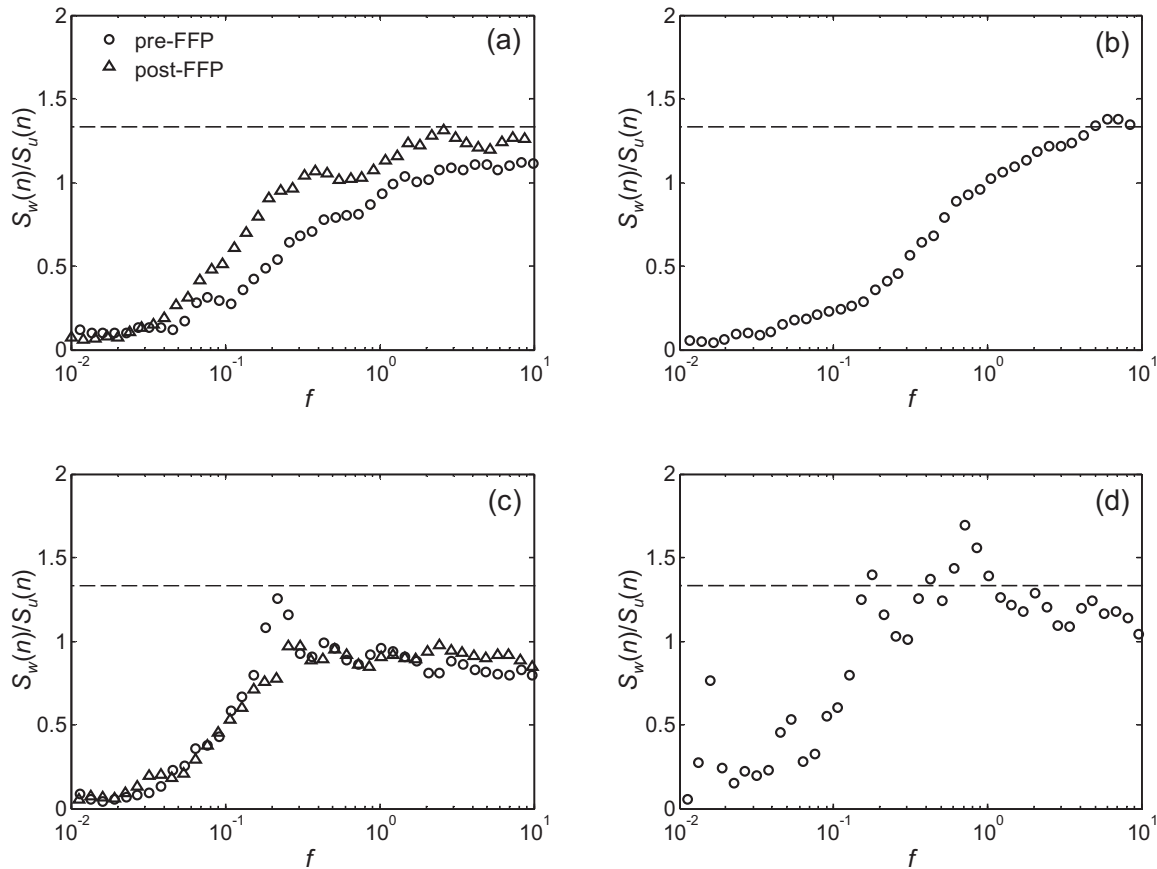
Fig. 4. Ratios of vertical to streamwise power spectra as a function of the normalized frequency, f = nz/U for the experimental burns (a)–(d) as shown in Fig. 1. Pre- and post-FFP spectra are shown with circles and triangles, respectively. The ratio of 4/3 is indicated by a dashed line to allow for assessment of isotropy.
