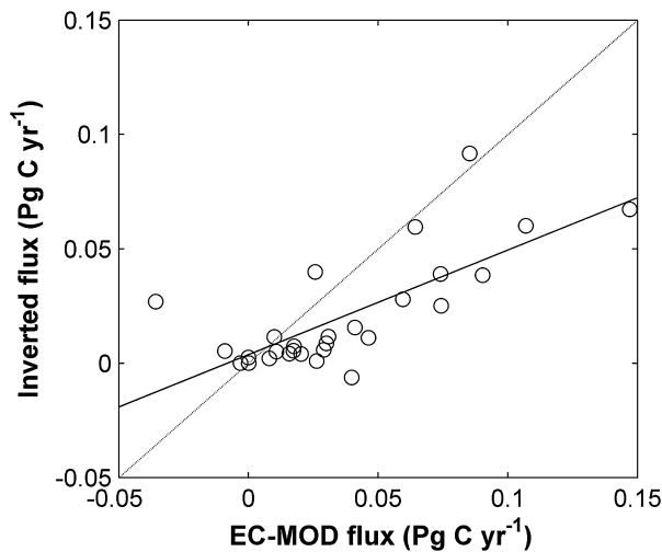
Fig. 5. Comparison of our annual NEP estimate (EC-MOD) against the inverted flux from a nested atmospheric inversion model.
