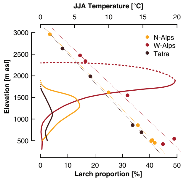
Figure 6 Proportion of European larch in the N-Alps, W-Alps and Tatra, as well as corresponding regional summer temperature conditions. JJA temperatures are derived from station data (dots, 1961–1990) and linear regressions (straight lines). Dashed curves are distribution estimates for high elevation locations up to the regional treelines. [Colour figure can be viewed at wileyonlinelibrary.com ].
