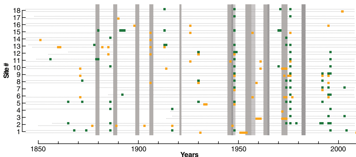
Figure 3 Comparison of reported larch budmoth (LBM) outbreaks in the Central and Eastern Alps (grey bars, based on Baltensweiler & Rubli, 1999) with growth anomalies ( >2 \times SD based on Fig. 2) in larch (orange) and spruce (green) 30 year spline detrended ring width indices ( RWI_{30} )-chronologies from the Northern pre-Alps. Sites are sorted by elevation. Dotted lines represent individual chronology lengths (Table 1). Grey bars indicate LBM outbreaks in the Central Alps; these are light grey in the Eastern Alps and dark grey in both the Central and Eastern Alps. [Colour figure can be viewed at wileyonlinelibrary.com ].
