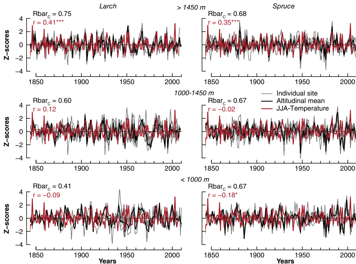
Figure 2 Larch and spruce chronologies from 18 locations in the Northern pre-Alps compared with local summer temperatures. All records were high-pass filtered (30-year spline) and normalized. R\bar{r}_c is the inter-chronology correlation within an elevational belt, and r is the correlation coefficient between temperatures and elevational mean chronologies over the period 1850–2000 (* P < 0.05 , *** P < 0.0001 ). [Colour figure can be viewed at wileyonlinelibrary.com ].
