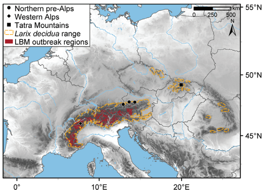
Figure 1 Natural distribution of Larix decidua and delimitation of larch budmoth (LBM) outbreak regions in Central Europe and tree-ring sampling sites. In the Northern pre-Alps, L. decidua (LBM host species) and Picea abies (nonhost species) were sampled at 18 sites. In the Western Alps and Tatra Mountains, only L. decidua was sampled. [Colour figure can be viewed at wileyonlinelibrary.com ].
