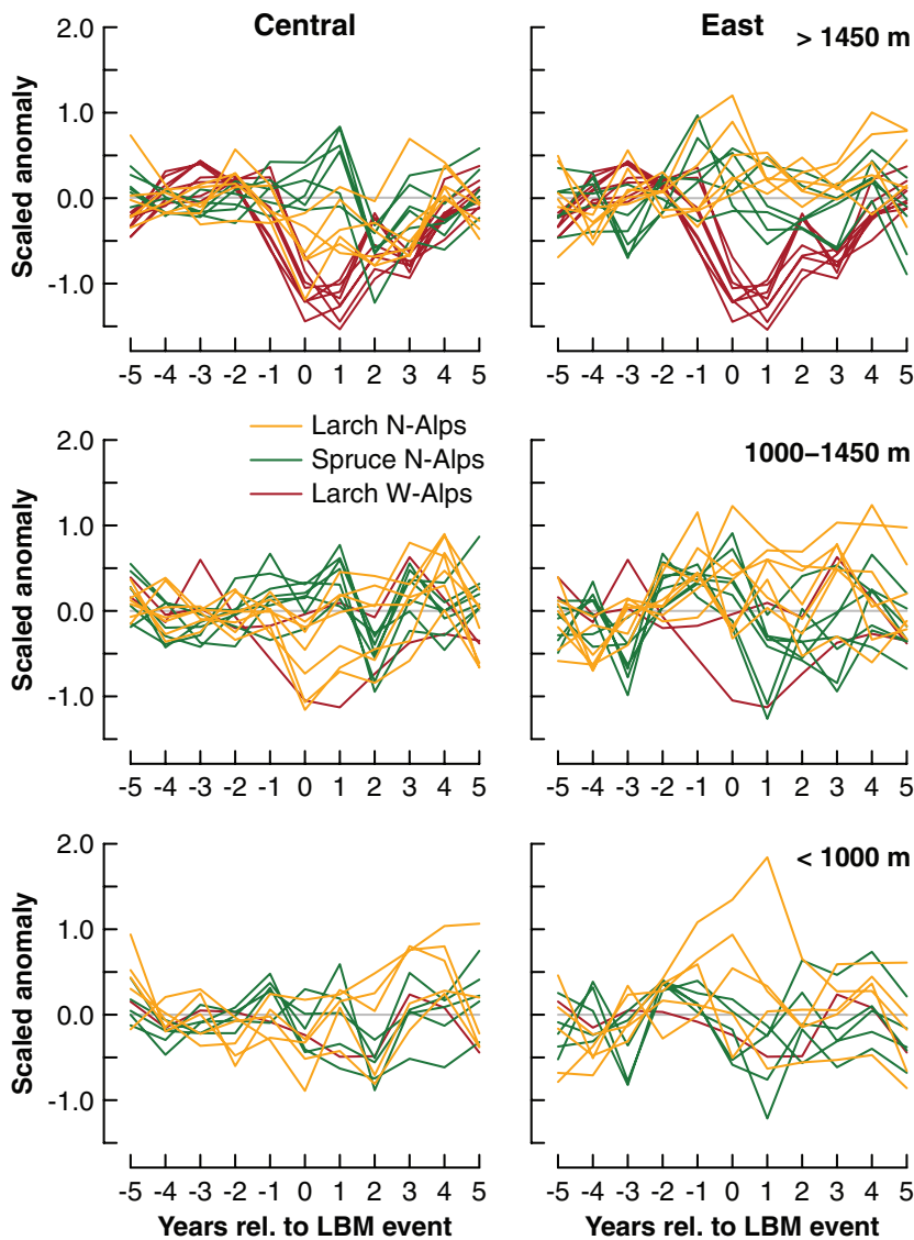
Figure 4 Superposed epoch analysis for N-Alps larch (orange) and spruce (green) 30 year spline detrended ring width indices ( RWI_{30} )-chronologies. Records are aligned (=year 0) considering reported larch bud-moth (LBM) outbreaks in the Central (1906, 1921, 1946, 1954, 1963, 1972 and 1982) and Eastern Alps (1947, 1957, 1965 and 1982). The typical LBM outbreak pattern is indicated by the W-Alps larch chronologies (red). These records were aligned (=year 0) considering outbreaks in 1900, 1908, 1915, 1923, 1929, 1937, 1945, 1954, 1963, 1972 and 1981. [Colour figure can be viewed at wileyonlinelibrary.com ].
