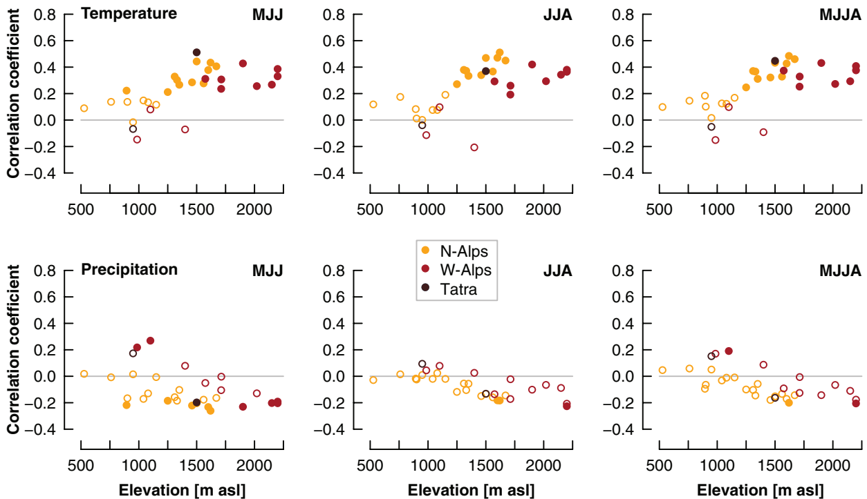
Figure 5 Seasonal growth/climate responses in different larch growing regions (orange = N-Alps, red = W-Alps, brown = Tatra) as a function of elevation. Top: results for temperatures; bottom results for precipitation. Correlations calculated using 200 year spline detrended ring width indices ( RWl_{200} )-chronologies. Filled dots indicate significant correlations ( P \leq 0.05 ). [Colour figure can be viewed at wileyonlinelibrary.com ].
