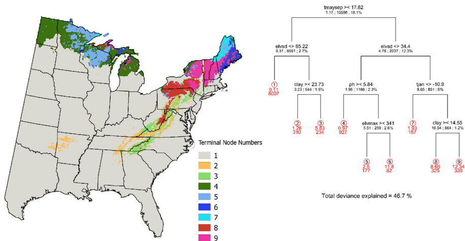
Fig. 5 Mapped decision tree. The terminal node numbers (numbers inside rounded circles) in the decision tree correspond to the classes in the map legend. In order to understand what predictor rules are driving the distribution of hemlock, we trace the decision tree rules from the terminal node. For example, the rule that corresponds to the highest abundance predicted (terminal node number 9 (magenta), average diameter of 12.34) has the rule TMAYSEP \leq 17.62 C and ELVSD > 34.4 and TJAN > -10.9 C and CLAY < 14.55%. The numbers below the terminal nodes correspond to the average response (in this case average diameter) and the number below that is the number of cells in the map (339 for class 9)
