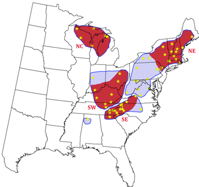
Fig. 2 The original polygonized TESS clusters (blue outline) are subset to Northcentral (NC), Northeast (NE), Southwest (SW) and Southeast (SE) zones to reflect FIA plots density and geographic separation (the red areas). We discount the original extreme Southwest outlier cluster because of the small size and few FIA plots. The yellow stars are the sampled microsatellite populations
