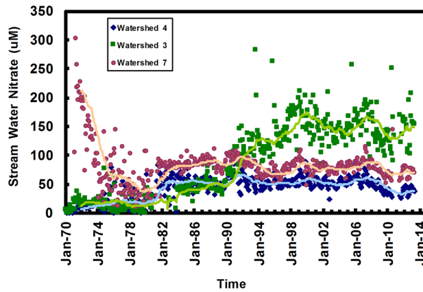
Figure 5. Long-term (40 years) volume-weighted monthly stream-water nitrate concentrations for each of the study watersheds. Ammonium sulfate additions to WS3 (35 kg N/ha/yr) began in 1989. Fitted lines are 24-month running means. Initially high values for WS7 were the result of a clearcutting and herbicide treatment that ended in October of 1969. Based on data from Edwards and Wood (2011) with updates: https://doi.org/10.2737/RDS-2011-0017 .
