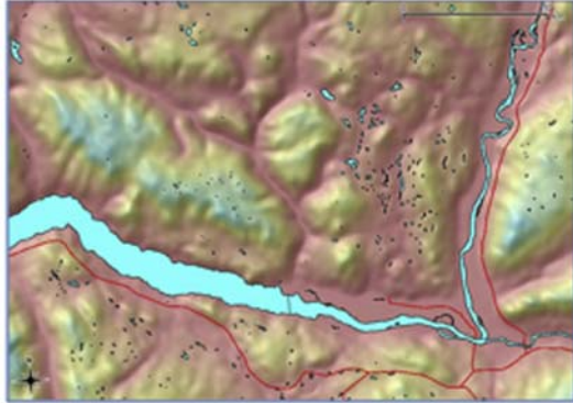
Altitude above channel network
