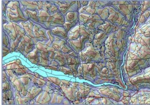
Relative hydrologic slope position with soil lines
