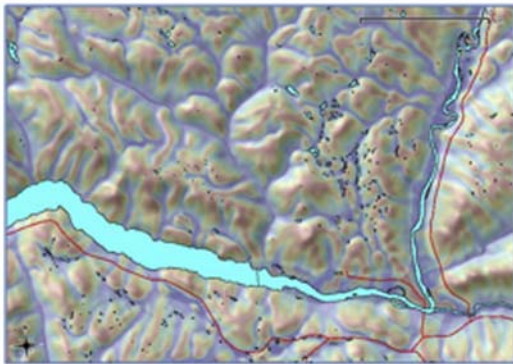
Relative hydrologic slope position
