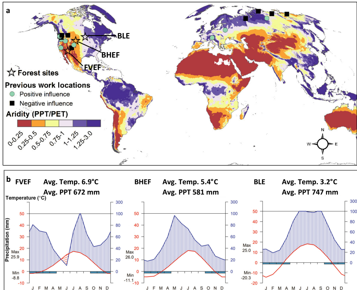
FIG. 1. (a) Previous work locations where researchers investigated the relationship of snow to forest growth, are shown in cyan circles where a positive influence was found (Kirdyanov et al. 2003, Guarín and Taylor 2005, Littell et al. 2008, Hu et al. 2010, Trujillo et al. 2012, Anderegg et al. 2013, Castagneri et al. 2015, Kharuk et al. 2015a), and in black squares where a negative influence was found (Peterson et al. 2002, Littell and Peterson 2005, Littell et al. 2008, Kharuk et al. 2015b). The three forest research sites included in this study (Fort Valley Experimental Forest [FVEF], Black Hills Experimental Forest [BHEF], and Birch Lake Experimental research area [BLE]) are shown as black stars. PPT, precipitation; PET, mean annual potential evapotranspiration. (b) Monthly ensemble mean values of PRISM-derived temperature and precipitation data are shown as Walter-Lieth diagrams, as well as average temperature (Avg. Temp.) and average precipitation (Avg. PPT) for the three forest research sites from the experimental period of 1960–2009.
