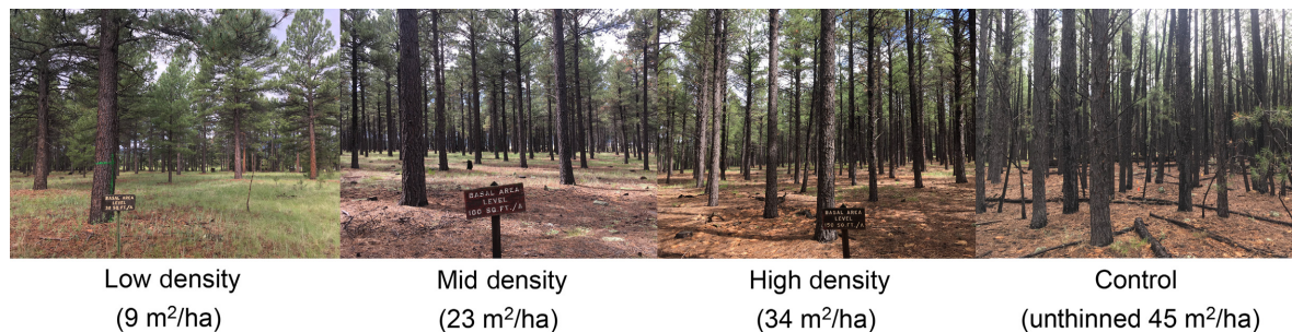
FIG. 2. Control (untreated) and high, mid, and low forest density treatments in ponderosa pine forests at the Fort Valley Experimental Forest site near Flagstaff, Arizona, USA. Photos: K. Gleason.
