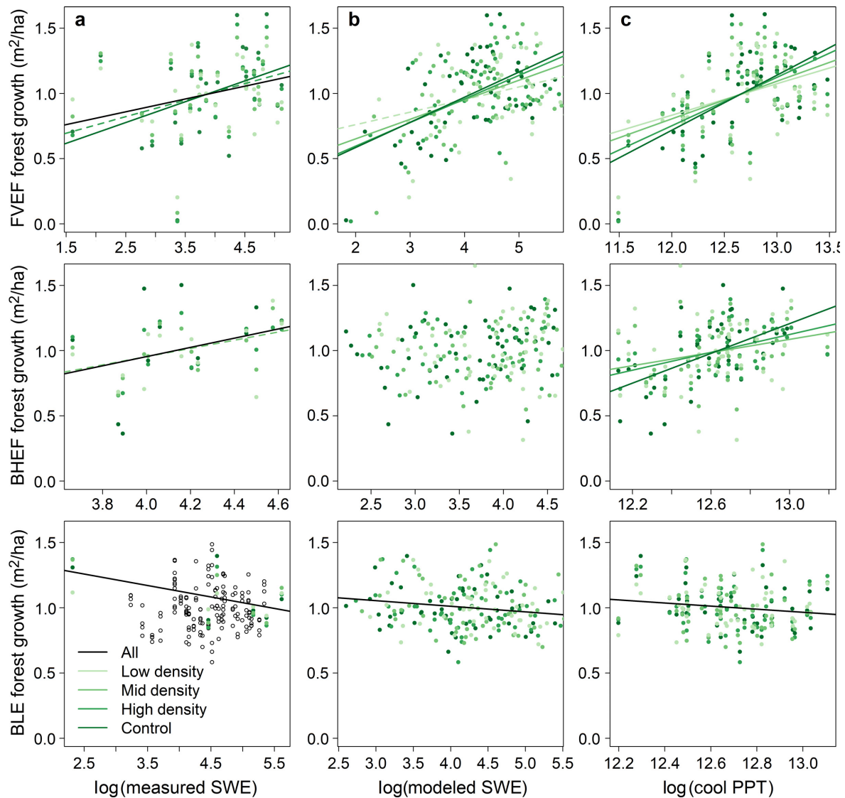
FIG. 4. Forest growth and snow metrics for each density treatment at each site for all treatments (shown in black) and for low, mid, and high density and control treatment plots (shown as green gradient). (a) Relationship between forest growth ( \text{m}^2/\text{ha} ) and measured SWE (mm) at the nearest SNOTEL/SCAN site to each research site (Fort Valley [FVEF, 1981–2009], Black Hills [BHEF, 1997–2009], Birch Lake [BLE, 2000–2009]), and black open circles in measured SWE at BLE are from Marcell Experimental Forest (1962–2009). (b) Relationship between forest growth ( \text{m}^2/\text{ha} ) and modeled SWE (mm). (c) Relationship between forest growth ( \text{m}^2/\text{ha} ) and PRISM-derived winter precipitation (mm; October–April). Linear models, P , and R^2 values are shown in Table 1 for each significant linear regression model. Linear models shown as solid lines indicate a P < 0.05 , and as dashed lines indicate a P < 0.1 . All modeled and PRISM-based snow accumulation parameters extended the full observed experimental period (FVEF, 1962–2009; BHEF, 1963–2009; BLE, 1960–2008).
