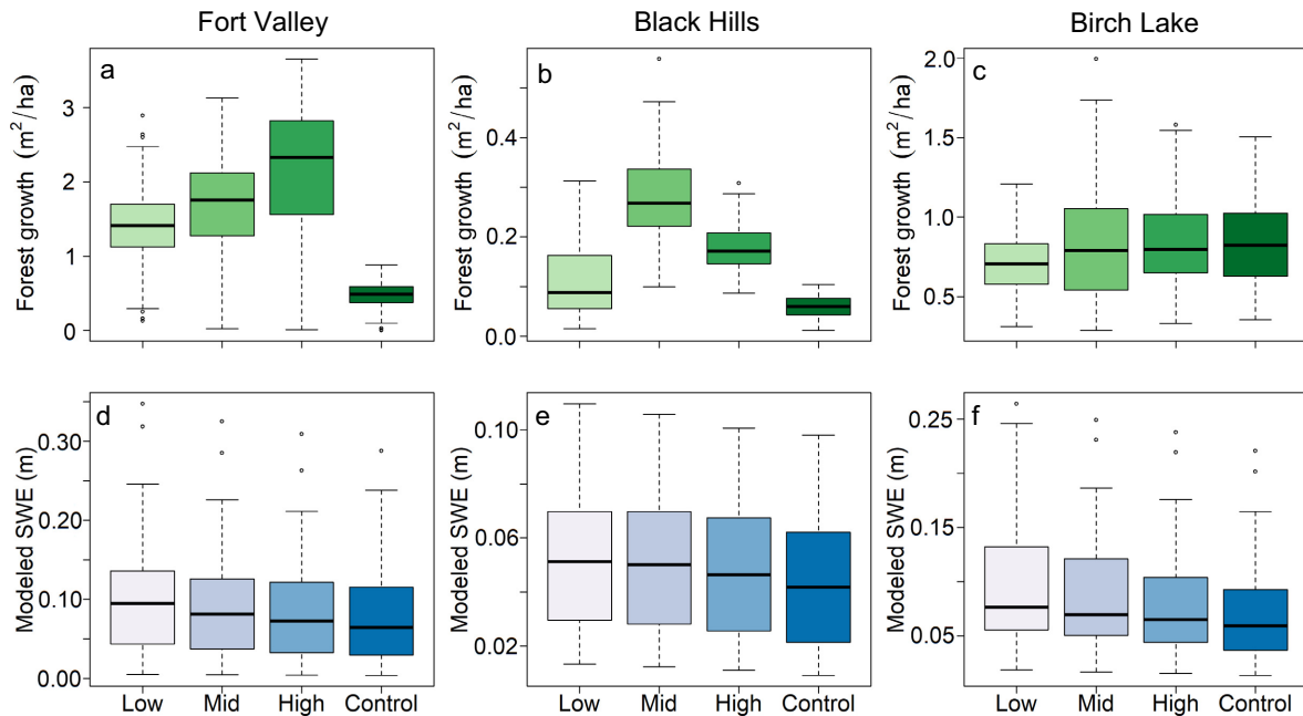
FIG. 3. Measured forest growth (or basal area increment, BAI) and modeled snow water equivalent (SWE) in low, mid, and high density and control treatments for each site. Uncorrected forest growth (BAI) for low, mid, high, and control density treatments from the experimental period of 1960–2009 in (a) Fort Valley, (b) Black Hills, and (c) Birch Lake research sites. Modeled SWE in low, mid, high, and control density treatments from the experimental period of 1960–2009 in (d) Fort Valley, (e) Black Hills, and (f) Birch Lake sites. Box plot components are mid line, median; box edges, 2nd and 3rd quartiles; and whiskers, 1st and 4th quartiles.
