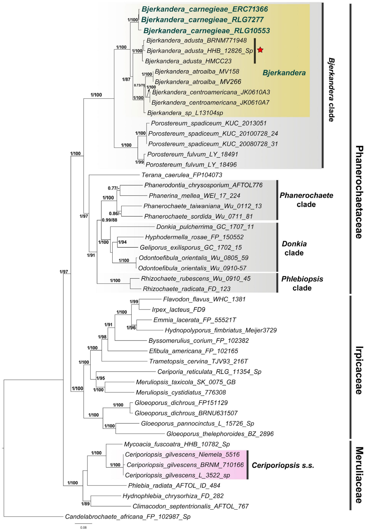
Figure 1. Maximum Likelihood (ML) tree of Phanerochaetaceae based on concatenated dataset of ITS + LSU + rpb1 + rpb2 + tef1-α sequence data. Branch support values are shown as BPP/BS, Bayesian posterior probability above 0.7 and Bootstrap values above 70%. ★ = type species of Bjerkandera .
