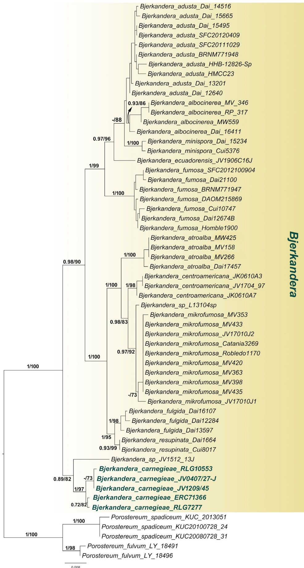
Figure 2. Maximum Likelihood (ML) tree of Bjerkandera based on concatenated dataset of ITS + LSU sequence data. Branch support values are shown as BPP/BS, Bayesian posterior probability above 0.7 and Bootstrap values above 70%.
