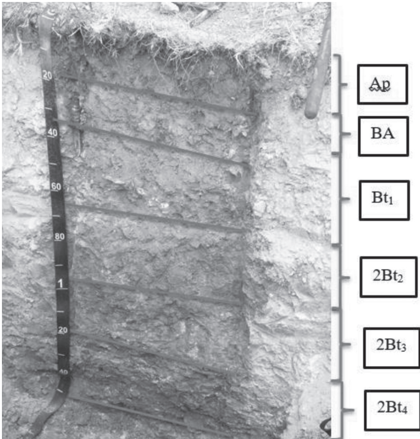
FIGURE 5. Horizon depths and designations of the Poynor soil profile.
