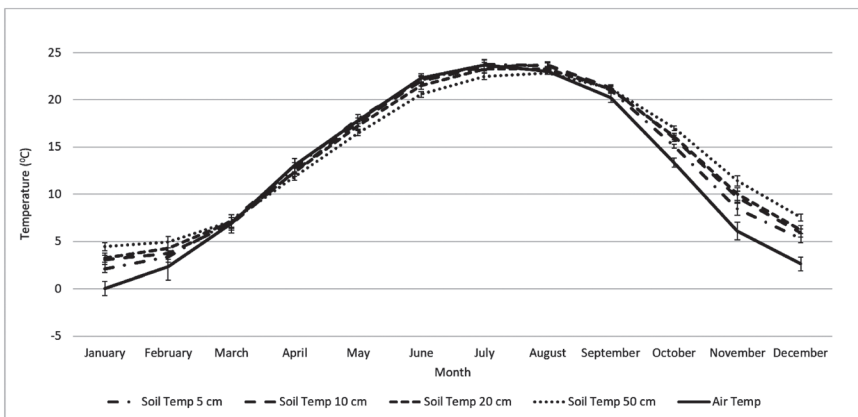
FIGURE 7. Mean monthly air and soil temperature data at different depths for Poynor soils (2012-2019). Error bars represent \pm 1 standard error.
