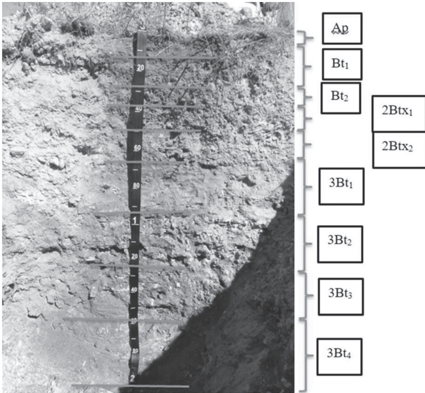
FIGURE 4. Horizon depths and designations of the Scholten soil profile.
