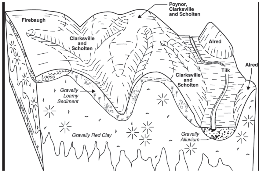
FIGURE 1. Typical pattern of soils and parent material of the Poynor-Scholten series (Benham and Daniel Childress, 2005).
