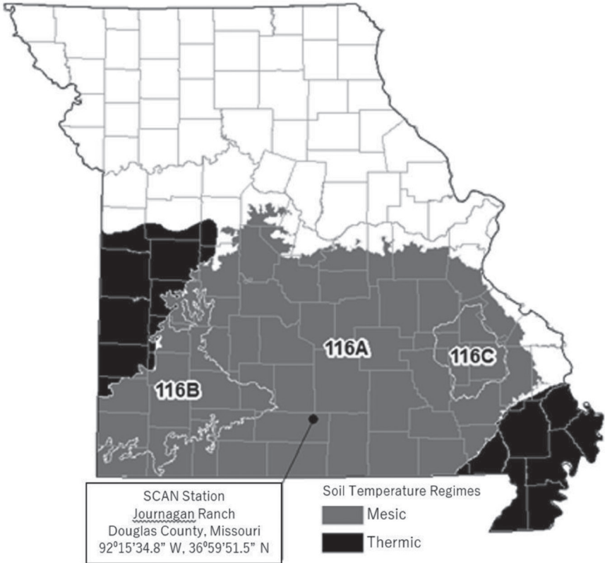
FIGURE 2. Location of the Journagan Ranch SCAN site, Douglas County, MO, in relation to Major Land Resource Areas (MLRAs) and Soil Temperature Regimes.
