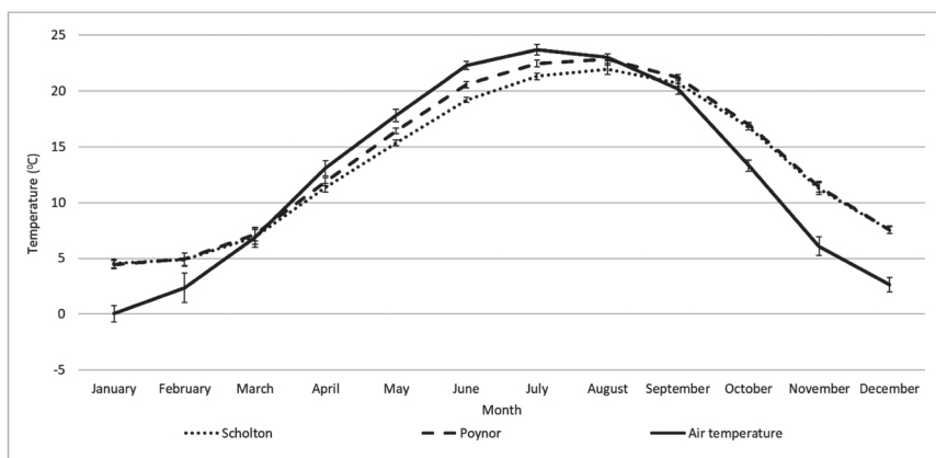
FIGURE 8. Mean monthly soil temperature (50 cm) and air temperature for the Scholten and Poynor pedons at the Journagan Ranch SCAN station. Error bars represent 1 standard error.
