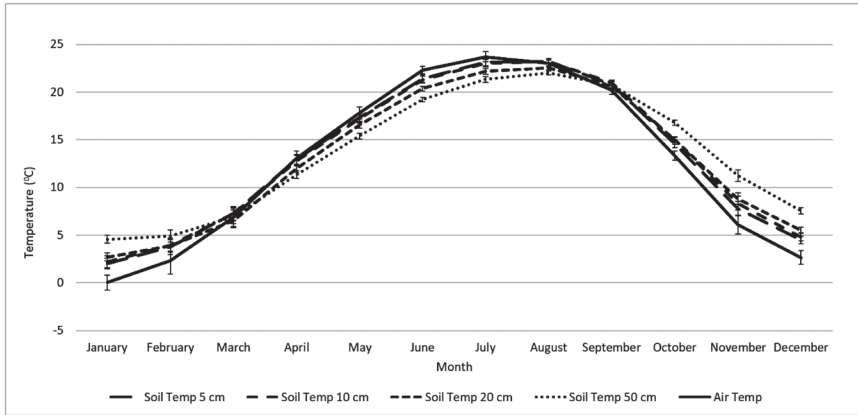
FIGURE 6. Mean monthly air and soil temperature data at different depths for Scholten soils (2012-2019). Error bars represent \pm 1 standard error.
