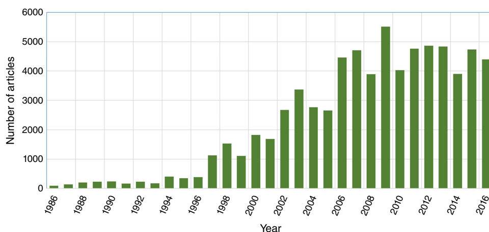
Fig. 1. Number of wildfire-related newspaper articles per year.
