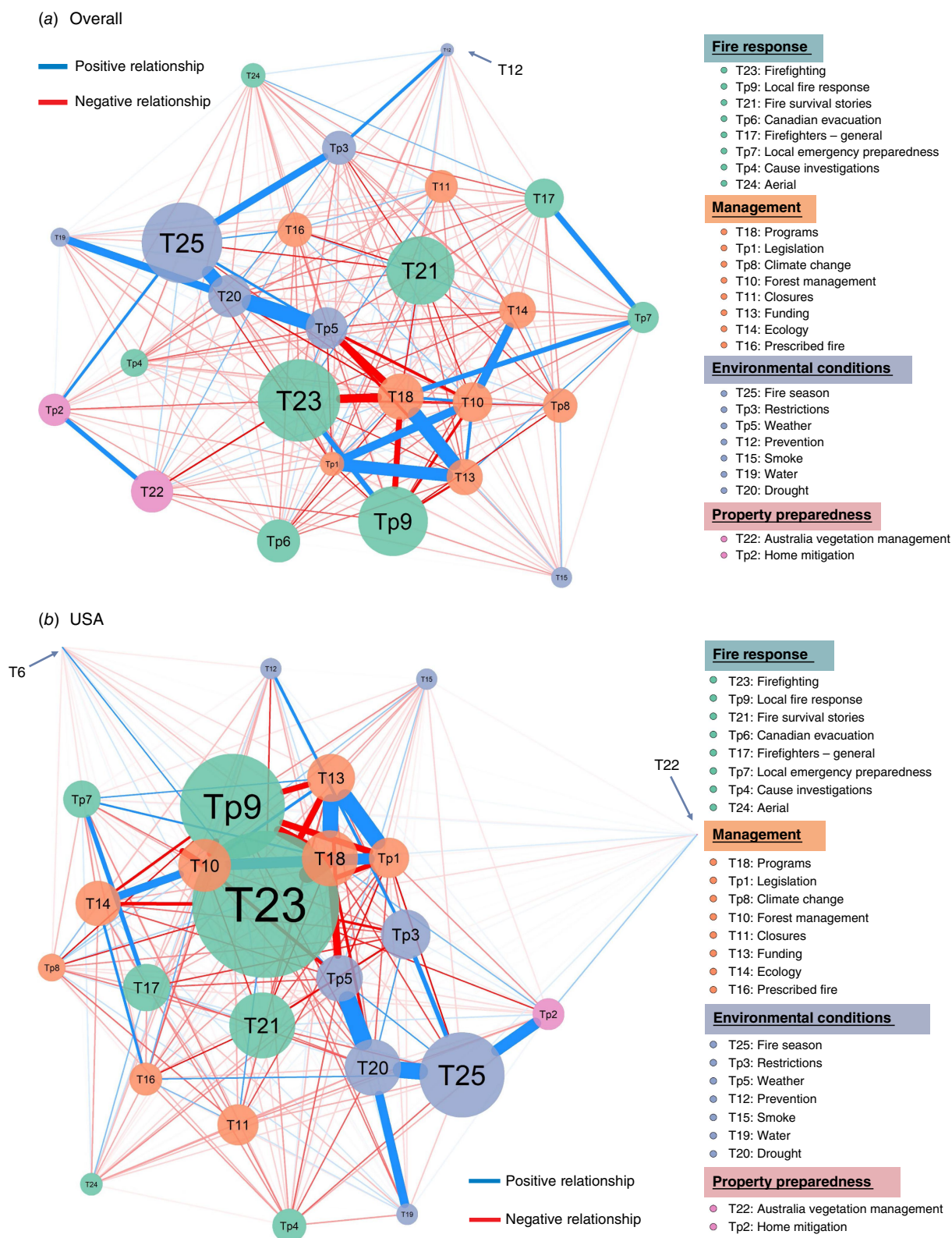
Fig. 3. Correlation network graphs of topic communities – (a) overall, (b) USA, (c) Canada and (d) Australia corpora. Topics in each grouping are listed in order of prevalence. Topics listed with a prefix 'T' vs 'Tp' are an artifact of the qgraph package used to create these network graphs, e.g. Topic 5 defaults to Tp 5 and Topic 15 defaults to T15.
