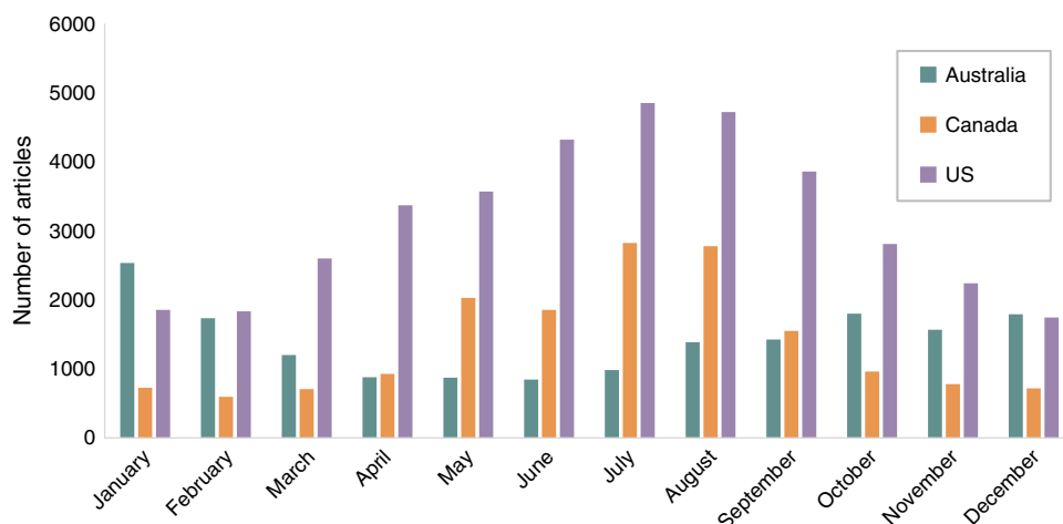
Fig. 2. Seasonality by month of wildfire-related articles per country.
