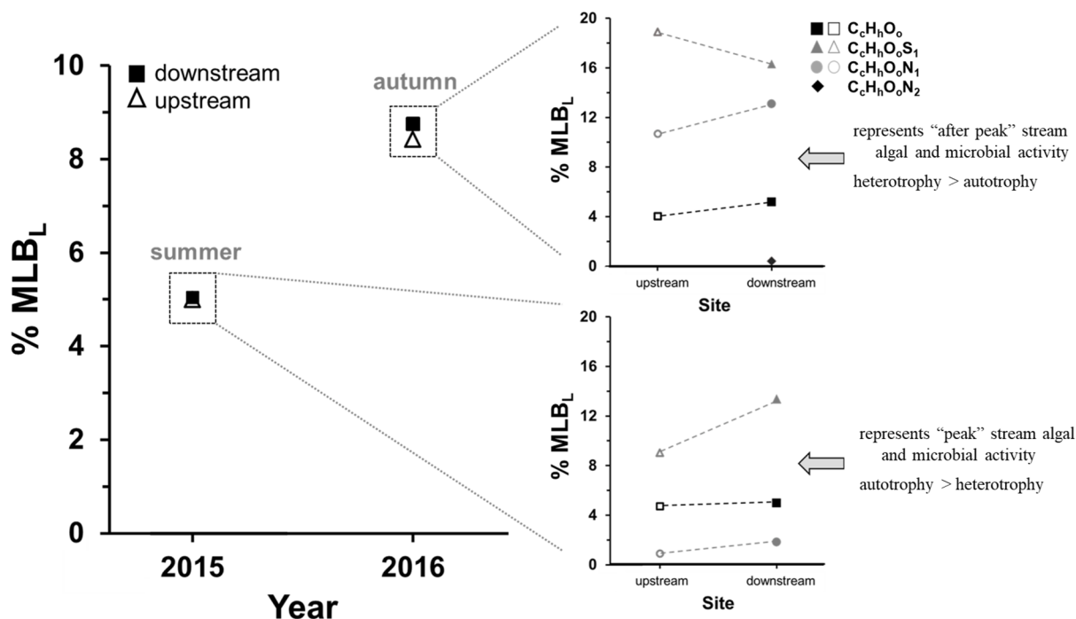
Fig. 5. Dissolved organic matter (DOM) molecular composition metrics of overall MLB_L and heterogeneous MLB_L for the stream samples collected from the West fork of the Gallatin River (Big Sky, Montana, USA) for summer 2015 and autumn 2016. The terms 'upstream' and 'downstream' refer to sampling locations on the river relative to the golf course adjacent to the reach between them. Heterogeneous MLB_L insets on the right represent "peak" and "after peak" microbial activity in the stream in different seasons. Black and white figure.
