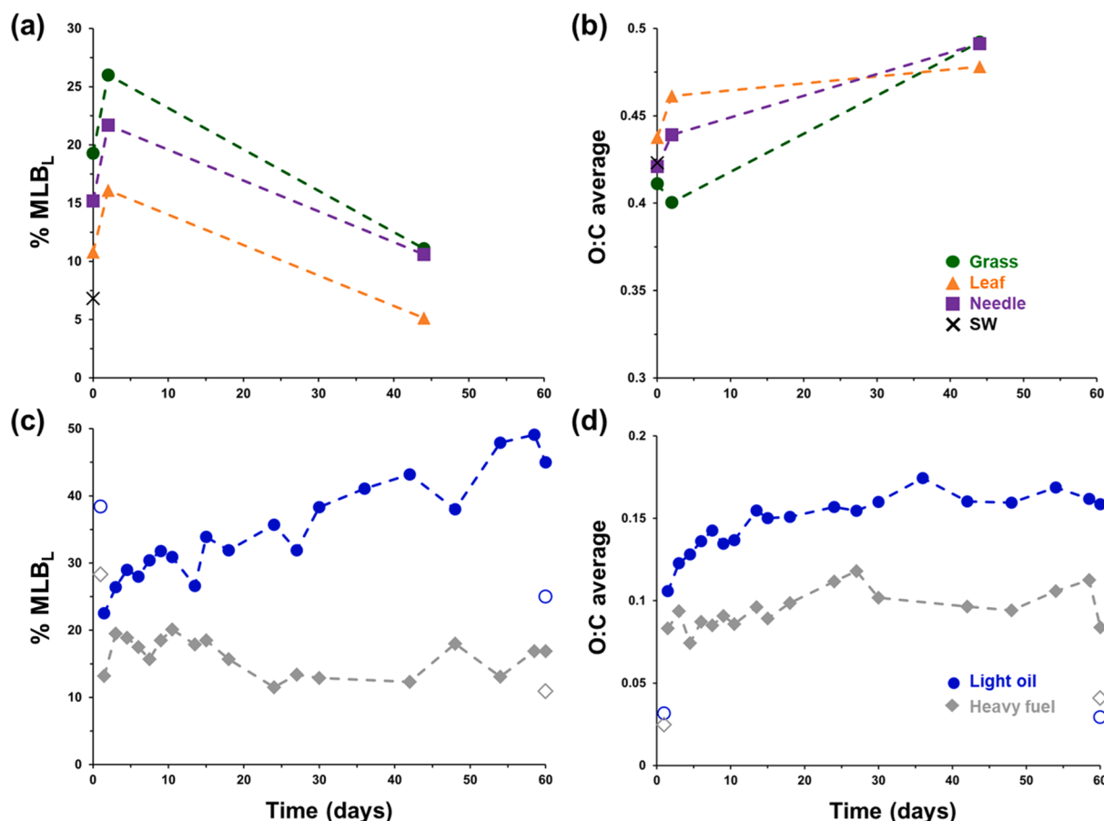
Fig. 3. Molecular composition metrics of MLBL percentages and oxygen-to-carbon ratio averages for (a–b) montane plant litter leachate dissolved organic matter (DOM) across a 44-day heterotrophic microbial degradation incubation (sources: grass, leaf, and needle) (D'Andrilli et al., 2019) and (c–d) two types of oil (light and heavy fuel) across a 60-day photodegradation experiment; open symbols denote dark controls. SW: Stream water from Sourdough Creek (Fig. S3c).
