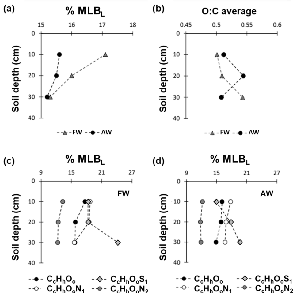
Fig. 6. Dissolved organic matter (DOM) molecular composition metrics of (a) overall MLB_L , (b) oxygen-to-carbon ratio averages, and (c-d) heterogeneous MLB_L from semi-arid arable soils in western Montana of fallow wheat and annual cropping systems across 0–10, 10–20, and 20–30 cm depths; adapted from Romero et al. (2018). FW: fallow wheat from conventional till, AC: annual cropping of no-till wheat. Black and white figure.
