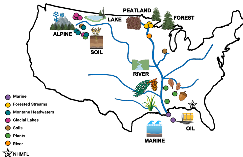
Fig. 1. Conceptual drawing of the greater Mississippi River Basin, USA, where our samples for organic matter characterization by FT-ICR MS analysis were collected. The location of the National High Magnetic Field Laboratory (NMHFL) is shown as a star (Tallahassee, Florida, USA).
