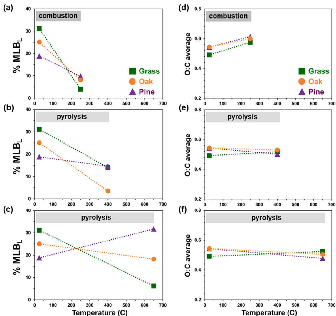
Fig. 4. Percent MLB L (a-c) and oxygen-to-carbon ratio averages (d-f) as a function of temperature for combustion (250 °C) and pyrolysis (400 °C and 650 °C) from FT-ICR MS data of Fakahatchee Grass (Grass), Laurel Oak (Oak), Loblolly Pine (Pine) biochar leachates. The parent biomass sources are depicted at room temperature (25 °C).
