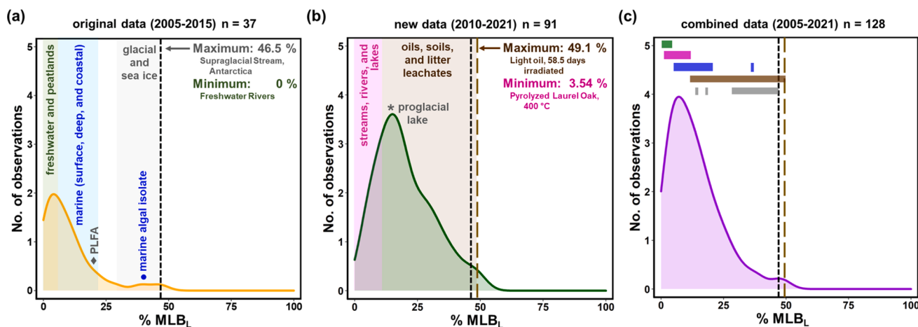
Fig. 2. MLB_L frequency distributions across samples from a) the original lability study (D'Andrilli et al., 2015), b) the new samples in this study, and c) the combined distribution of both studies. The black and brown dashed lines show the maximum calculated biolability values and the colored bars in (c) show the general grouping of sample types and their overlap; colors consistent with font color in the shaded regions in (a) and (b). Distributions represent smoothed kernel density estimates of environmental samples. The MLB_L values are available in Table S1. PLFA: Pony Lake Fulvic Acid.
