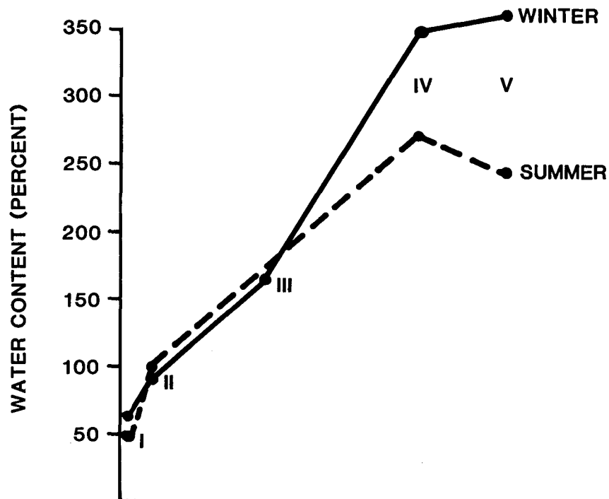
Figure 15.—Water content of fallen Douglas-fir trees in winter and summer; each point represents a decay class from I (newly fallen trees) to V (fallen trees decomposed to a mound of brown cubical rotted wood).
