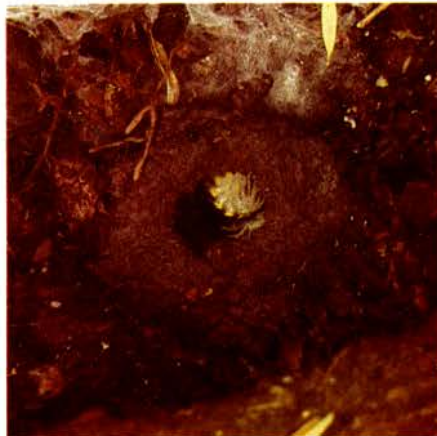
Figure 18.—A millipede ( Harpaphe haydeniana ) in a molting chamber made of organic debris under the loose bark of a class III fallen Douglas-fir tree.
