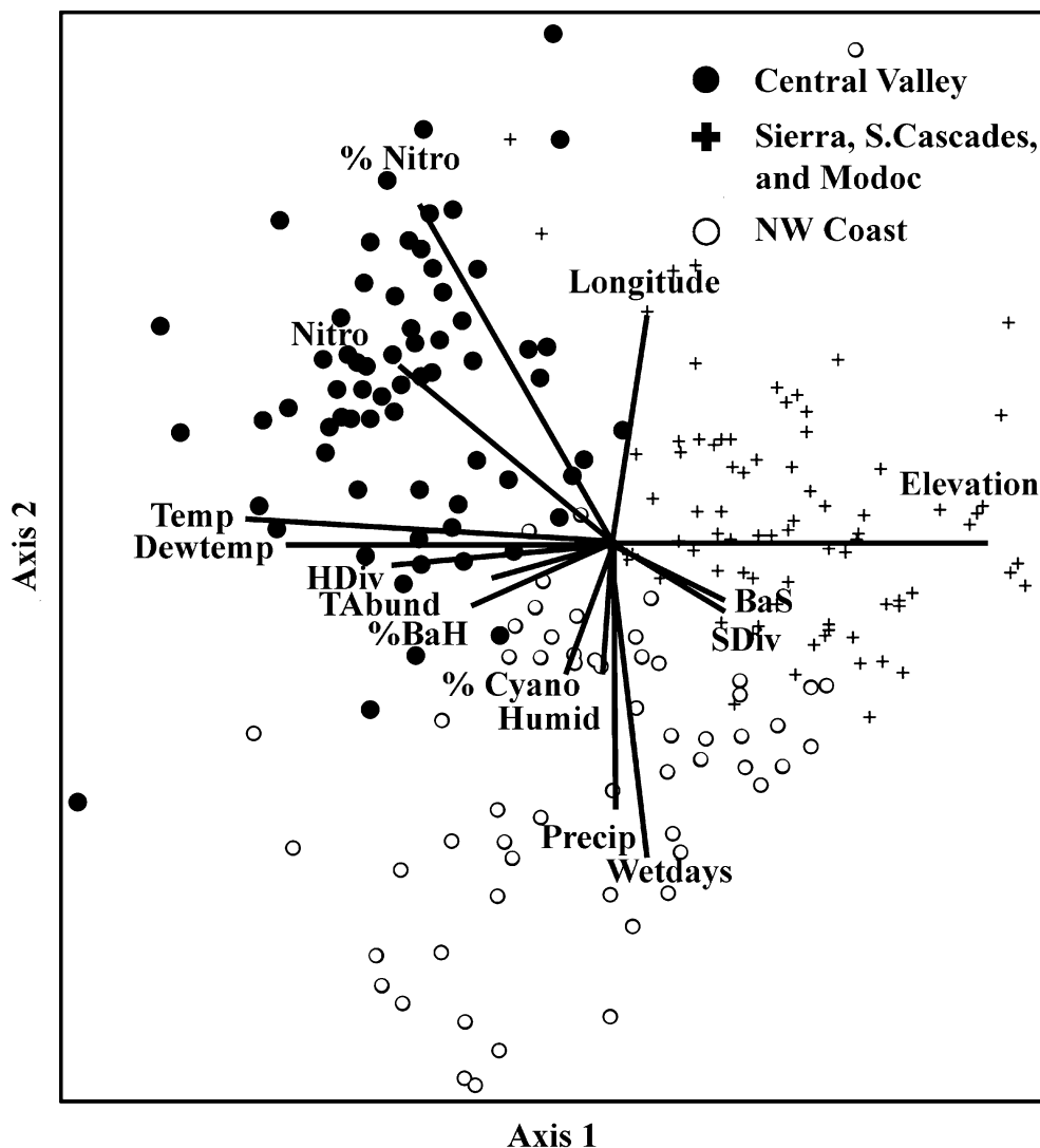
FIGURE 2. Ordination plotted to scale in a joint plot with environmental variables overlaid. Vector length and direction indicates correlations of the variable with ordination axes. Only vectors with an -0.42 < r > 0.42 for one axis are shown to prevent crowding. Related variables with overlapping vectors of similar strength are designated by a single label: "Temp" (temperature) includes mean temperature, minimum temperature, and maximum temperature. Nitro = nitrophile diversity, % Nitro = percent nitrophile diversity, BaS = basal area in softwoods, SDiv = softwood diversity, Precip = precipitation, Humid = humidity, % Cyano = percent cyanolichens, % BaH = percent basal area in hardwoods, TABund = total lichen abundance, HDiv = hardwood diversity, Dewtemp = dew temperature.
