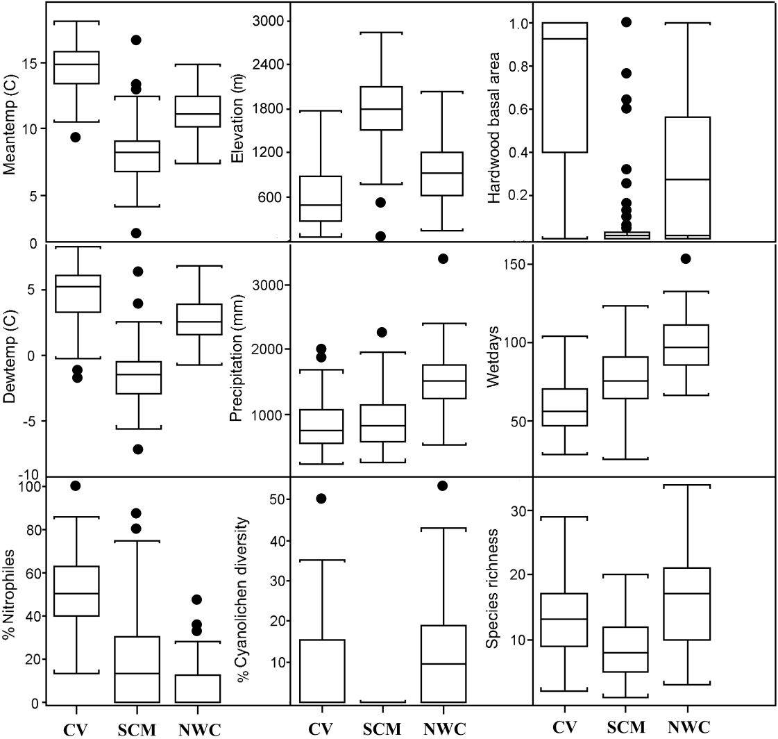
FIGURE 3. Boxplots of selected environmental variables, functional group indices, and species richness. The horizontal lines divide the data into quartiles. The center lines indicate medians and points represent outliers. CV = Greater Central Valley; SCM = Sierra, Southern Cascades, and Modoc; NWC = Northwest Coast.
