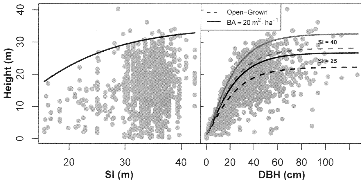
Figure 3. Prediction of maximum potential height for any Oregon white oak in a stand based on Douglas-fir site index (SI) (left), and prediction of potential height for individual trees based on their DBH and stand basal area (BA) (right). Lines show quantile regression fits for 95th quantile (left) and 90th quantile for two levels of stand density and site index (black lines show SI = 25 m, grey lines show SI = 40 m) (right).
