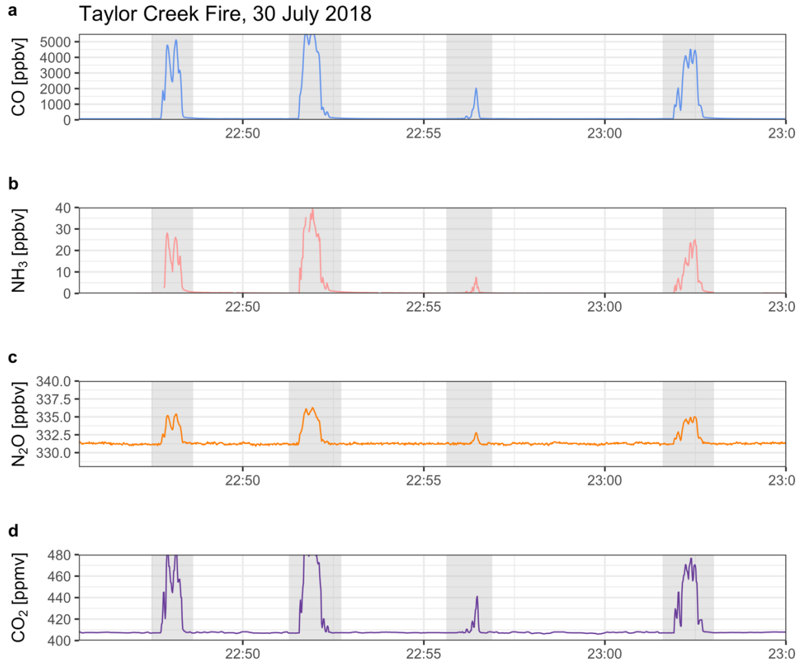
Figure S7. Timeseries of a) CO, b) NH 3 , c) N 2 O, and d) CO 2 for the Taylor Creek Fire, RF03. Grey shading represents emission transects.
