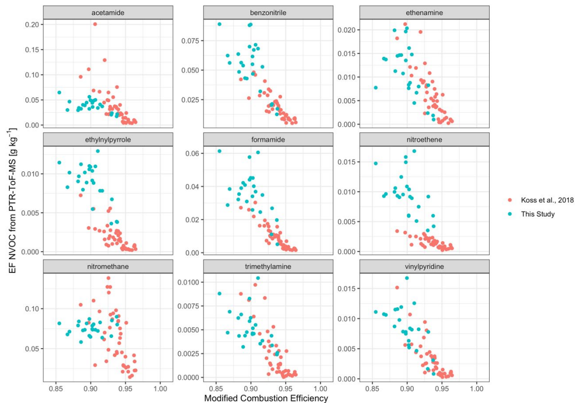
Figure S12. Comparison of the relationship between NVOC EFs and MCE from this study with those from Koss et al. (2018) for 9 identified species in common.
