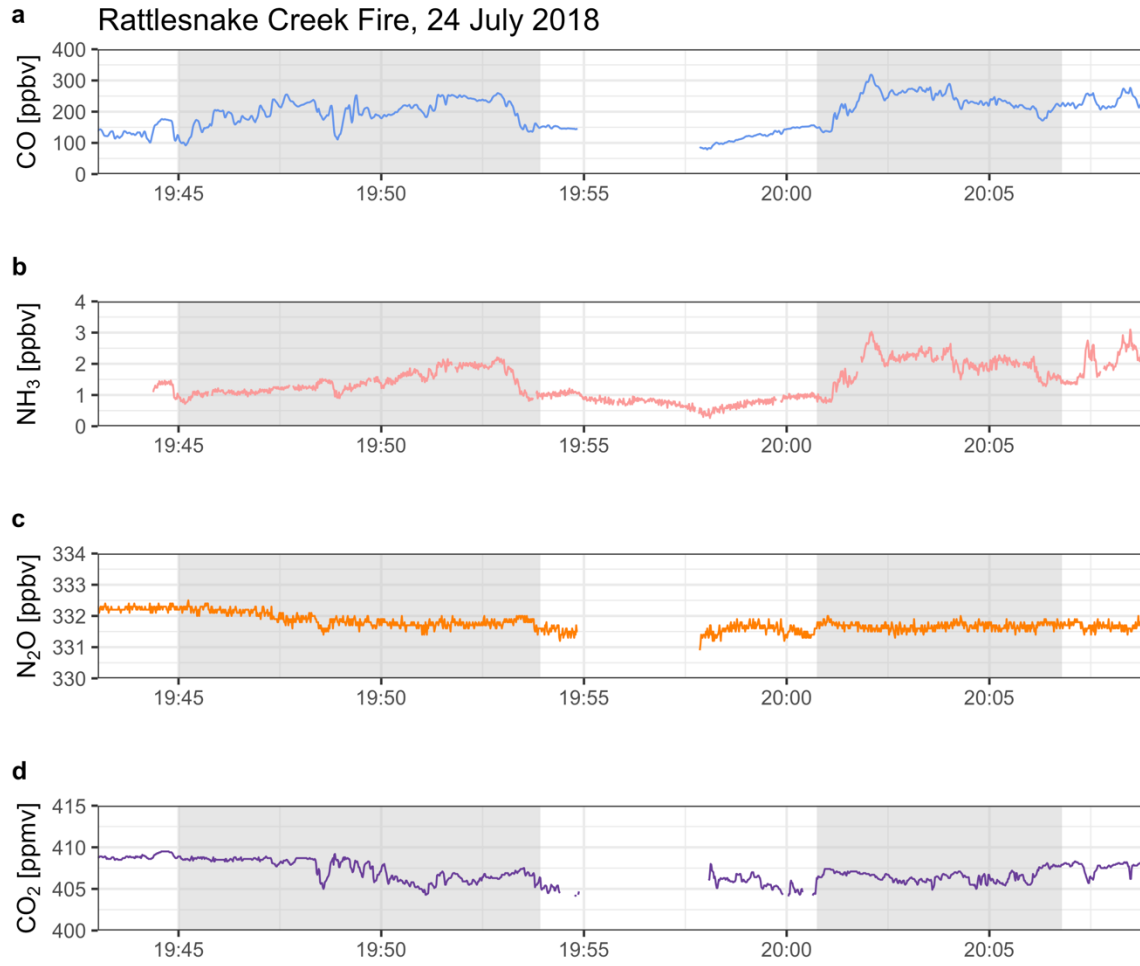
Figure S6. Timeseries of a) CO, b) NH 3 , c) N 2 O, and d) CO 2 for the Rattlesnake Creek Fire, RF01. Grey shading represents emission transects.
