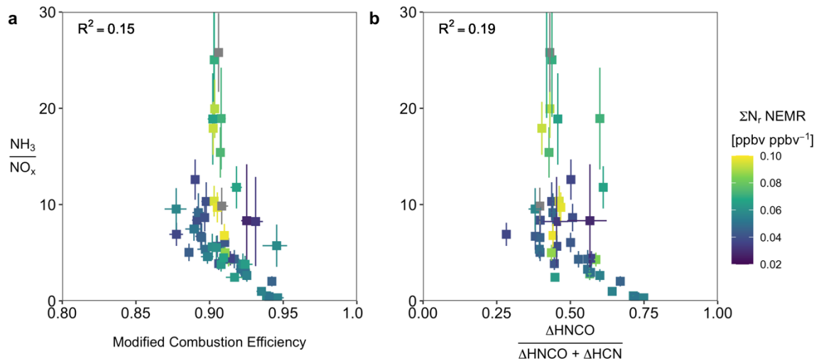
Figure S8. Relationship between the ratio of \text{NH}_3 to \text{NO}_x with, a) MCE, and b) the fraction of \text{HCNCO} + \text{HCN} that exists as \text{HCNCO} .
