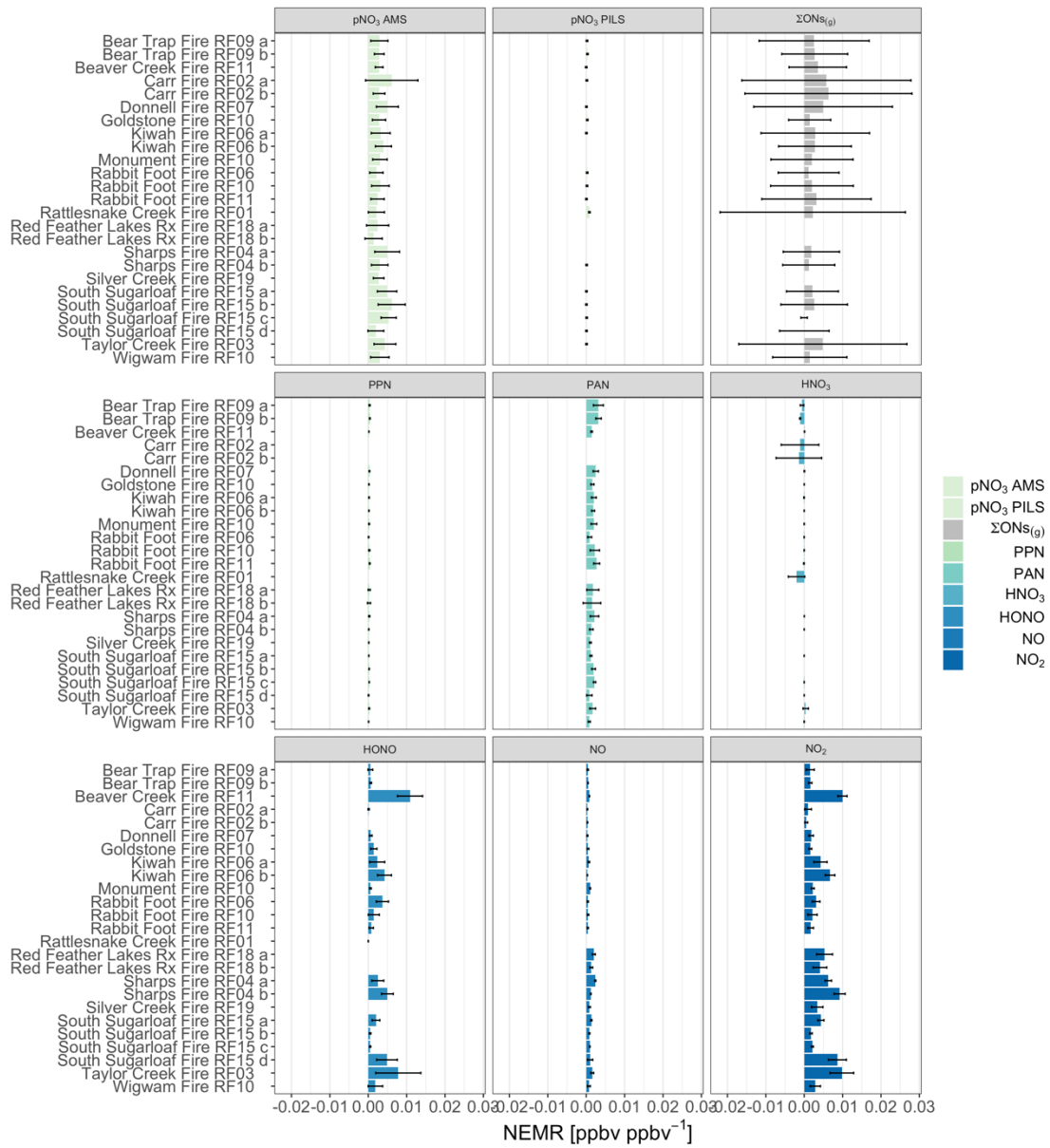
Figure S3. Normalized excess mixing ratios (NEMRs) of measured oxidized N_r species for emission passes of WE-CAN fires, plotted by measured species.
