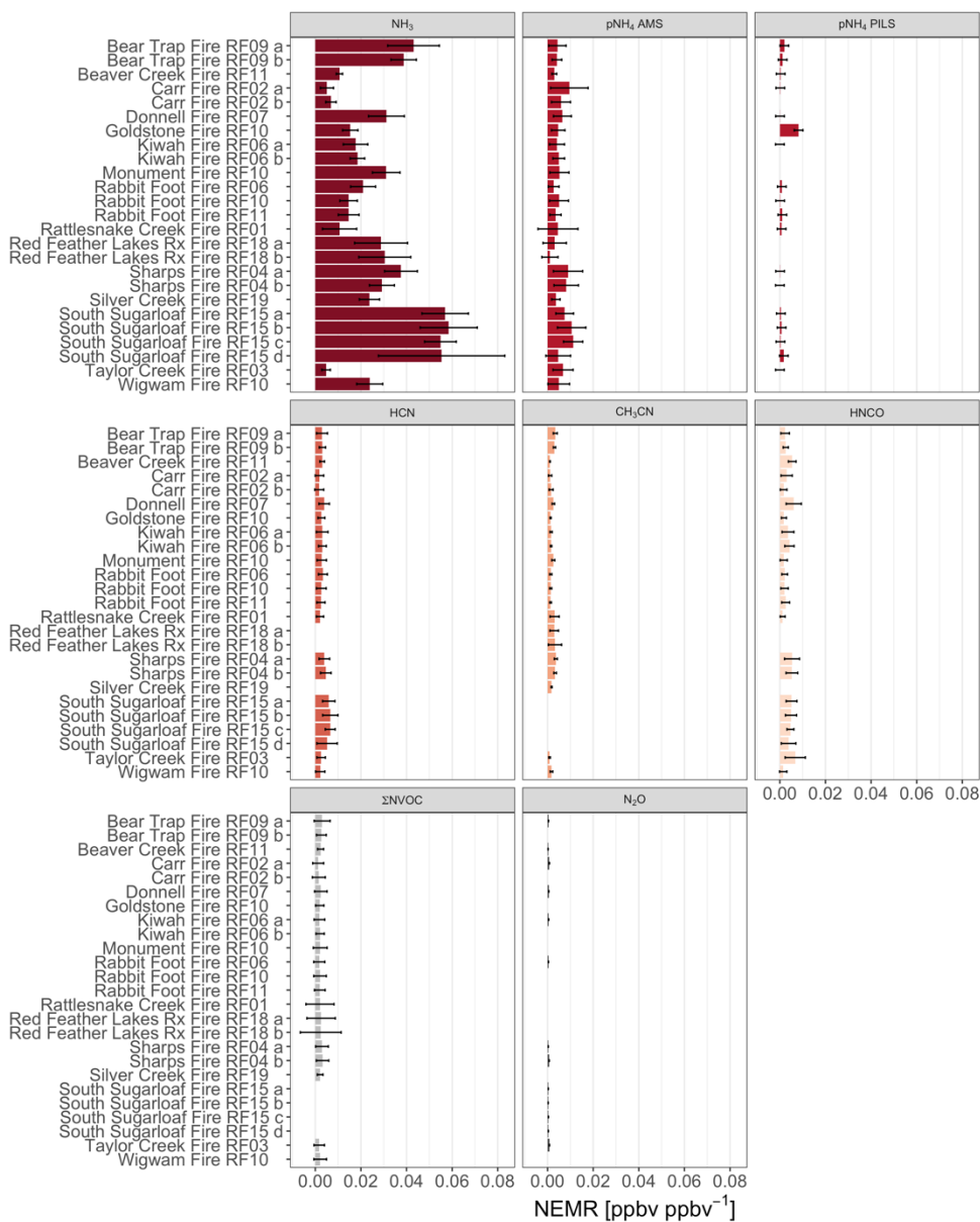
Figure S2. Normalized excess mixing ratios (NEMRs) of measured reduced N_r species for emission passes of WE-CAN fires, plotted by measured species. While not all NVOCs in \Sigma NVOCs are reduced, this quantity is also plotted here.
