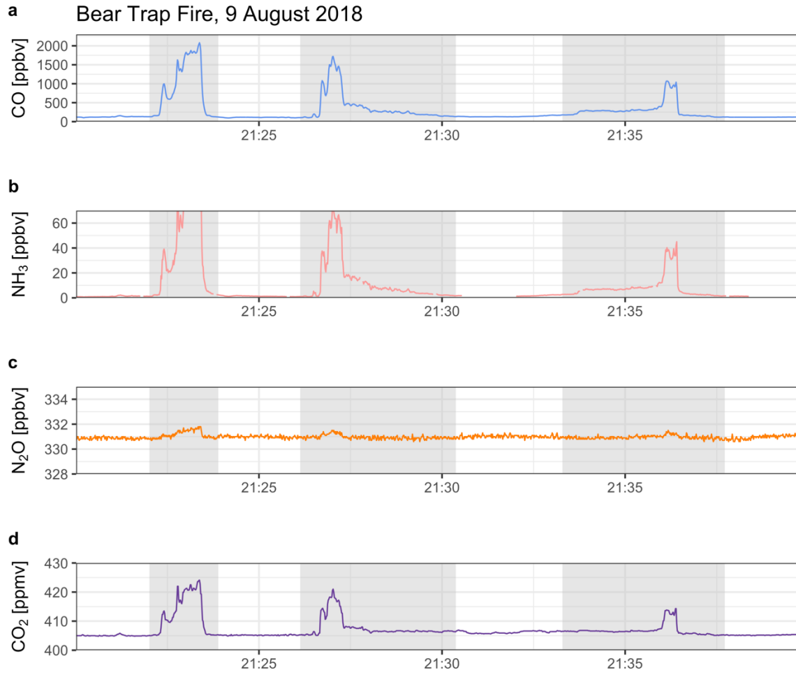
Figure S4. Timeseries of a) CO, b) NH 3 , c) N 2 O, and d) CO 2 for the Bear Trap Fire, RF09. Grey shading represents emission transects.
