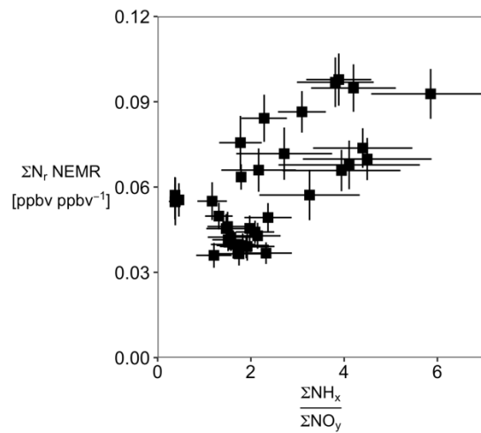
Figure S9. Relationship between the ratio of \Sigma\text{NH}_x/\Sigma\text{NO}_y with total measured \Sigma\text{N} .
