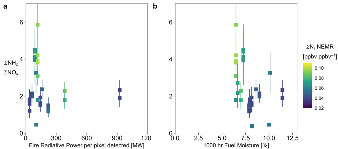
Figure S10. Relationships between the ratio of \Sigma\text{NH}_x [= \text{NH}_3 + \rho\text{NH}_4 ] to \Sigma\text{NO}_y with: a) fire radiative power from MODIS, and b) 1000hr fuel moisture estimates at the time of burn from GRIDMET.
