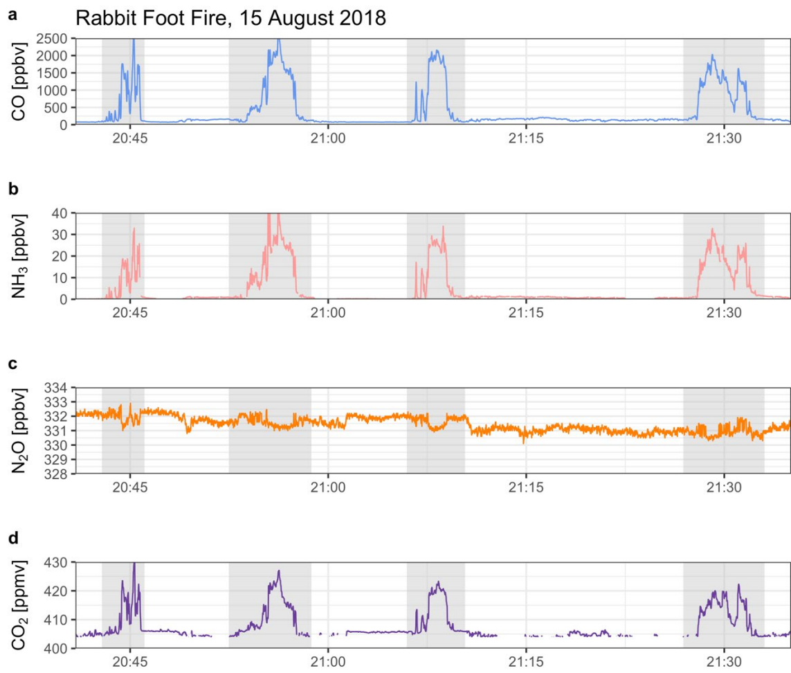
Figure S5. Timeseries of a) CO, b) NH 3 , c) N 2 O, and d) CO 2 for the Rabbit Foot Fire, RF11. Grey shading represents emission transects.
