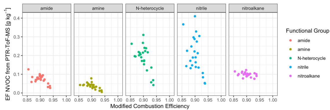
Figure S11. Comparison of the relationship between NVOC EFs and MCE.
