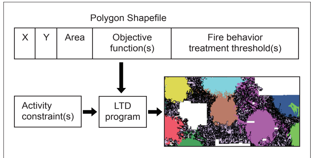
Figure 1—Diagram showing the input data and outputs of the Landscape Treatment Designer (LTD) program. Each record of the polygon shapefile contains data on (1) polygon XY centroid, (2) polygon area, (3) objectives, and (4) constraints. The latter two variables can be integer or real values. The outputs include a polygon shapefile that identifies the objective value for each polygon, and a code that specifies whether it was selected to be in a patch, and whether it was also selected for treatment.
