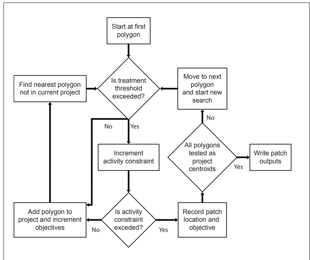
Figure 2—Flow chart of program control for the Landscape Treatment Designer program showing the decision framework for simulations that use the aggregation option.
