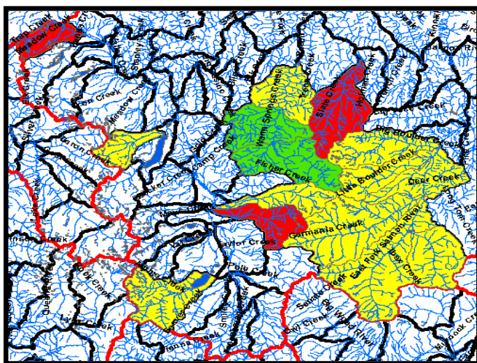
Figure 17—Predicted bull trout persistence in 2080. Red subwatersheds are at high extinction risk; yellow are at moderate risk, and green are at low risk.
