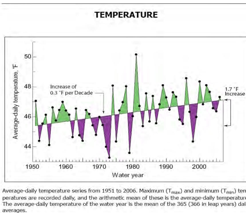
Figure 10—Average daily air temperatures from Flagstaff, 1950–2006 (Staudenmaier et al. 2007).
