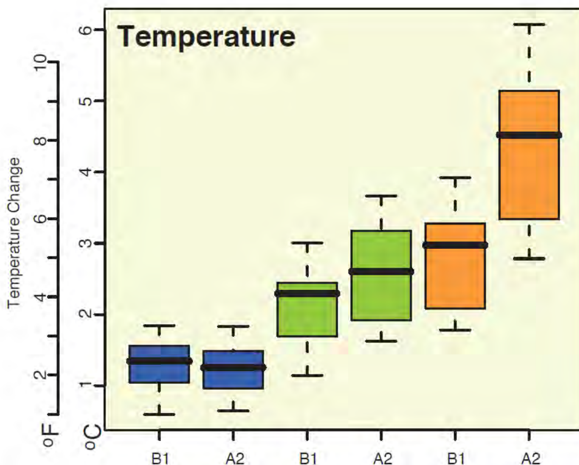
Figure 2—Possible air temperature changes predicted from down-scaled global circulation models for the Colorado River basin (Christensen and Lettenmaier 2006).
