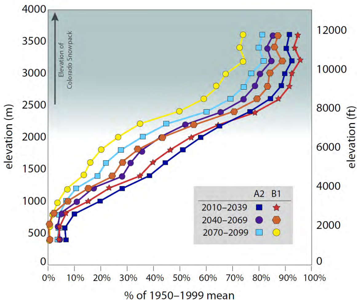
Figure 4—Predicted changes in Colorado River basin snowpack (Christensen and Lettenmaier 2006).
