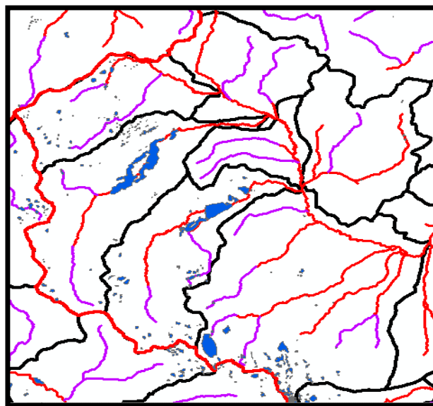
Figure 13—Available thermal bull trout habitat in Valley Creek on the Sawtooth NRA in 2080. Streams with optimal temperatures are portrayed in purple and those outside optimal range in red.
