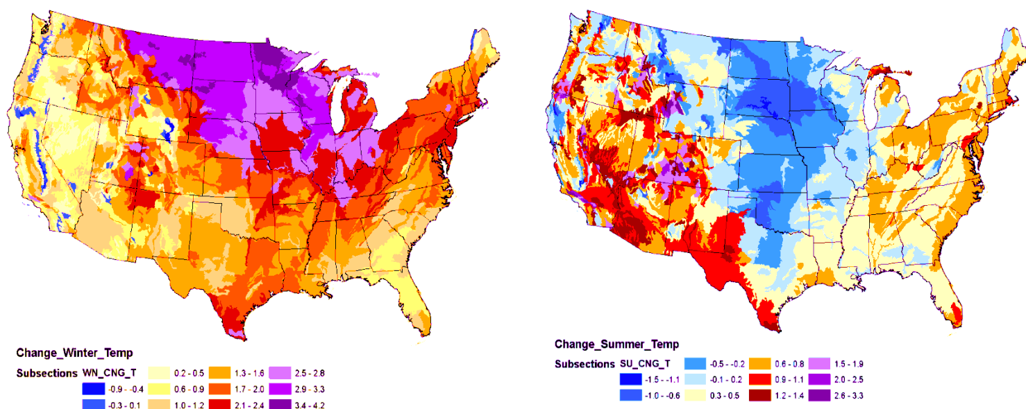
Figure 3—Winter (left) and summer (right) mean temperature changes in the United States, 1961–1990 compared with 1991–2007 (from Cleland, 2010)
