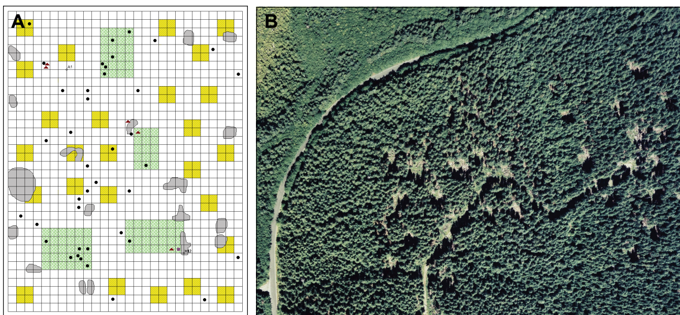
Figure 14—Example of a stand within the Olympic Habitat Development Study (OHDS). Corners of 66- by 66-ft (20- by 20-m) squares were marked on the ground (squares in diagram are 33 by 33 ft [10 by 10 m]). (A) This preexisting grid framework was used to map snags—black circles represent snags from previous stand, red triangles represent snags from current stand) and existing openings (gray). Subsequently, the grid was used to layout the skips (green) and gaps (yellow). (B) Aerial photo shows two OHDS plots at a different site shortly after treatment.
