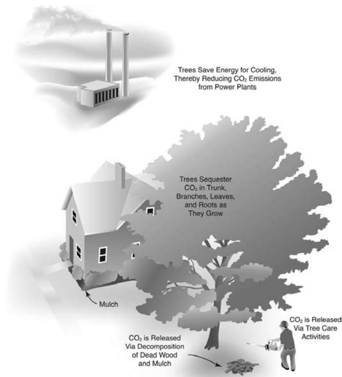
Figure 5 . Trees sequester CO 2 as they grow and indirectly reduce CO 2 emissions from power plants through energy conservation. At the same time, CO 2 is released through decomposition and tree care activities that involve fossil-fuel consumption (drawing by Mike Thomas).
