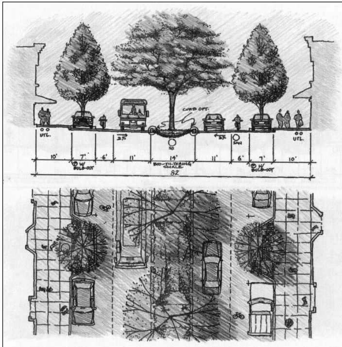
Figure 29. Tree canopy can create a continuous canopy for maximum rainfall interception, even in commercial areas. In this example, a swale in the median filters runoff and provides ample space for large trees. Parking space-sized planters contain the soil volume required to grow healthy, large trees (from Metro 2002).
