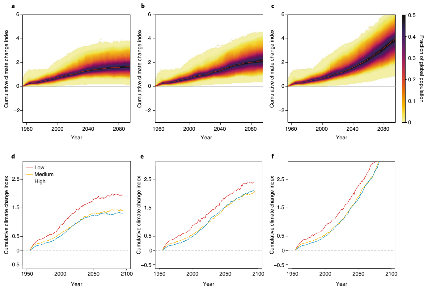
Fig. 3 | Human population exposure to simultaneous climate hazards. a–c , The fraction of the world’s human population exposed to varying levels of cumulative hazards under three RCPs: RCP 2.6 ( a ), RCP 4.5 ( b ) and RCP 8.5 ( c ). d–f , Exposure to cumulative climatic hazards for half of the total population in countries with low, medium and high incomes under the same scenarios.
