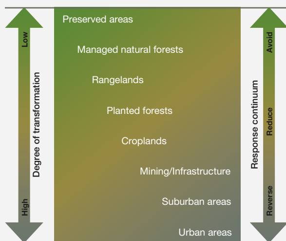
Figure 6.15 A schematic diagram showing the degree of land transformation (none or minimum in dark green colour to substantial transformation in dark grey colour) resembling land use types from preserved natural areas to urban areas with a response continuum (avoid, reduce and reverse).
