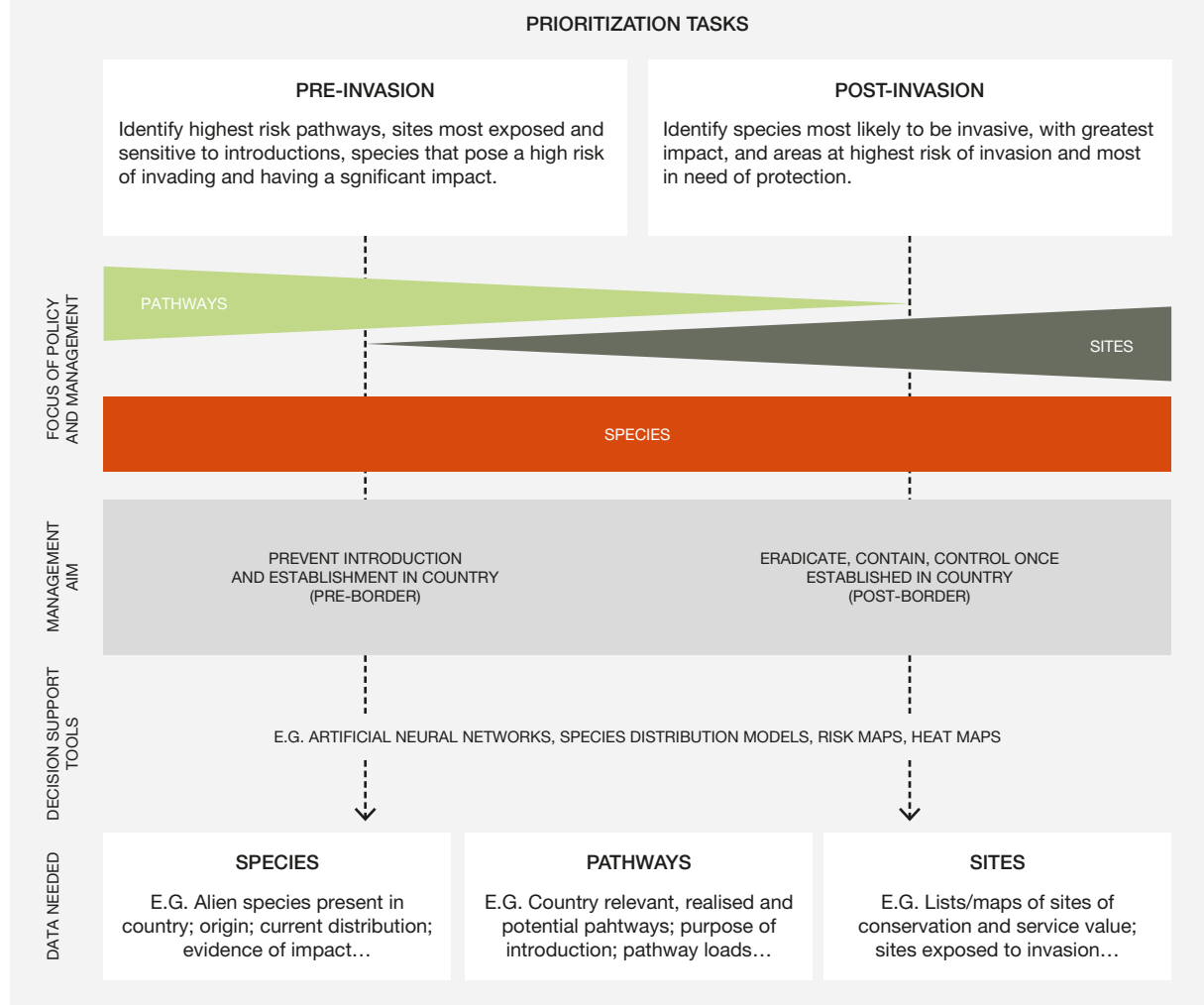
Figure 6 8 Prioritization to support cost-effective allocation of resources is part of decision-making at nearly every stage of the invasion process, from preventing introduction of invasive alien species, to preventing their spread, to eradication or containment. Source: McGeoch et al. (2016).
