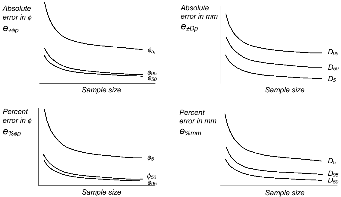
Fig. 5.23: Comparison of error curves around the D_5, D_{50}, and D_{95} percentile for different computations of error (absolute, percent, \phi -units and mm). All computations are for the same gravel deposit. A normal and symmetrical parent distribution was assumed in (A), and an asymmetrical distribution positively skewed towards a tail of fines was assumed in (B).
