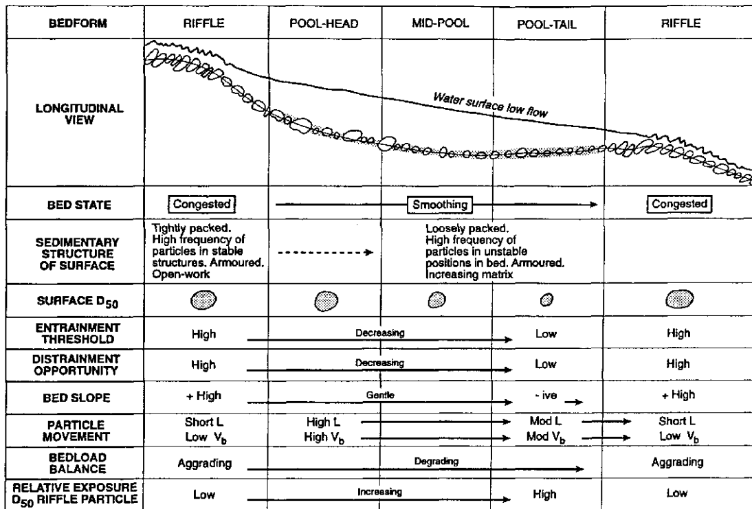
Fig. 3.9: Model of bed material properties and bedload parameters in a riffle-pool sequence. + = very, -ive = negative, L = particle transport distance, V_b = particle transport velocity, Relative exposure of D_{50} particle = within the bed material. (Reprinted from Sear (1996), by permission of John Wiley and Sons, Ltd.).
