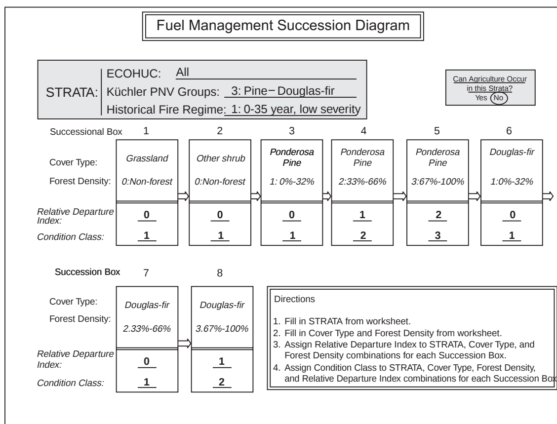
Figure 4 —Succession diagram example. Fields filled out in italics indicate information provided by summary reports (appendix C). Fields filled out in bold indicate information filled in by regional experts.
