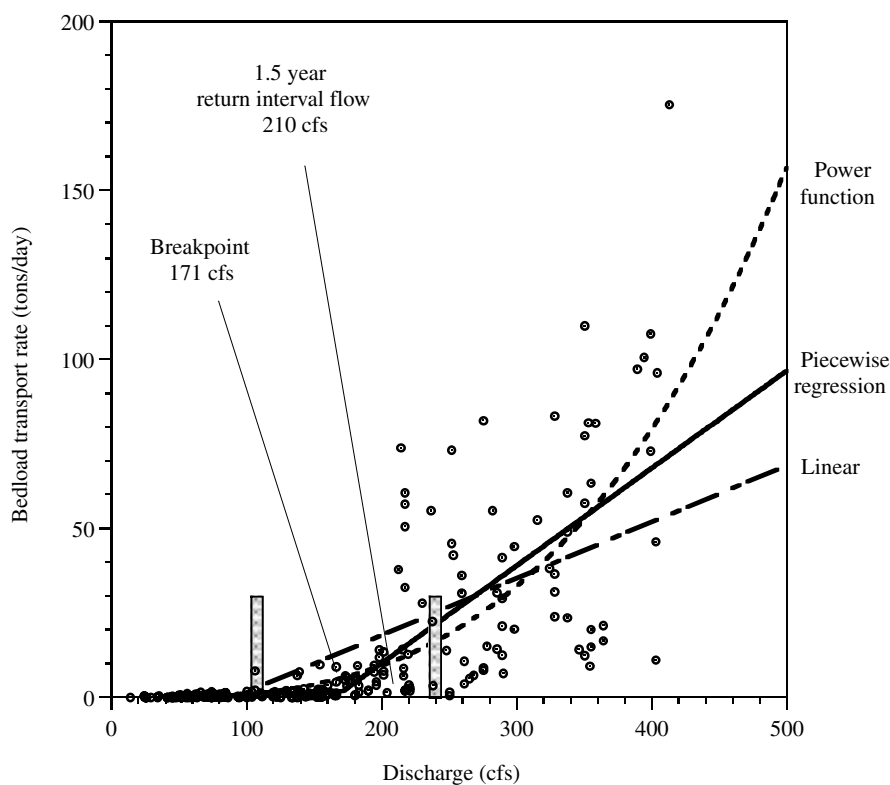
Figure 7 —Arithmetic plot of total bedload transport and water discharge for Little Granite Creek (from Ryan and Emmett 2002). The figure illustrates three fits (linear, power, and piecewise linear) to total bedload transport data on arithmetic scale and shows the breakpoint of 171 cfs. Bars represent the 95% confidence limits on the estimate of the breakpoint; bar height is arbitrary.
