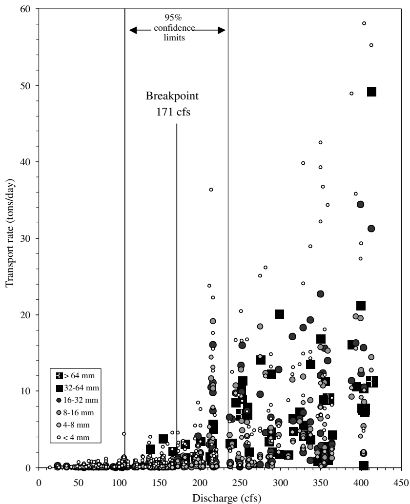
Figure 6 —Arithmetic plot of bedload discharge and water discharge by particle-size classes for Little Granite Creek (from Ryan and Emmett 2002). Lines indicate values of the breakpoint discharge (171 cfs) and the 95% confidence limits on the breakpoint estimate. The discharge at which coarse gravel begins to appear in the samples coincides more or less with the value of the breakpoint. The rate of bedload transport increases dramatically at about 220 cfs -- a value within the confidence limits of the breakpoint estimate from the piecewise regression procedure. Both estimates indicate a substantial increase in the amount of bedload transport at flows approaching bankfull (230 cfs).
