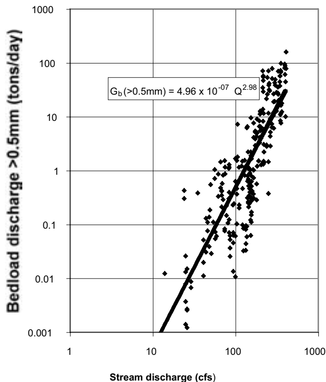
Figure 5 —Logarithmic plot of bedload transport ( G_b ) as a function of water discharge ( Q ) for Little Granite Creek (from Emmett 1999). A logarithmic plot of bedload transport tends to obscure the sudden increase in transport rates associated with the starting point of channel maintenance.
