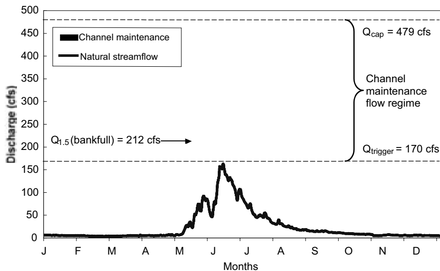
Figure 2c —A typical channel maintenance flow hydrograph applied to a low runoff year (exceeded 80% of years). The discharge data is from Halfmoon Creek, Colorado in 1991. The lower limit ( Q_{\text{trigger}} ) used to initiate the channel maintenance flow regime is 0.8 of the 1.5-year flow and the upper limit ( Q_{\text{cap}} ) is the 25-year flow. No channel-maintaining sediment transport occurs during this dry year because low flows are unable to move coarse sediment. During the low runoff year shown, none of the 16,094 acre-feet of total natural water yield is needed for channel maintenance.
