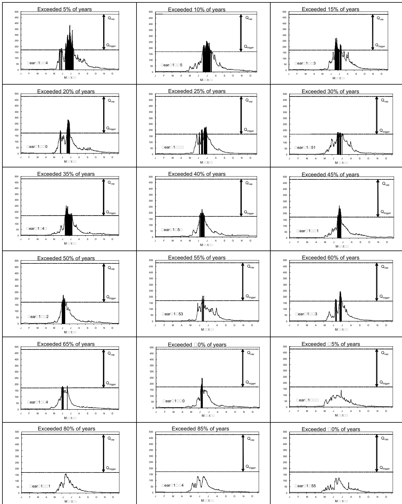
Figure 3— A sequence of channel maintenance flows from wet (exceeded 5% of years) to dry (exceeded 90% of years) years. The volume of water needed for channel maintenance (shown in black in the figures) is highly variable from year to year and the percent of annual water yield used for channel maintenance decreases from wet to dry years in a regular manner. During many low flow years (about one-third of all the years), channel maintenance flows are unnecessary because gravel-moving discharges fail to occur.
