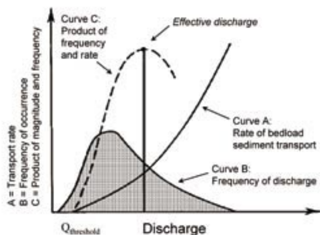
Figure 1 —The magnitude-frequency concept applied to bedload transport and discharge (adapted from Wolman and Miller 1960). The concept suggests that a range of intermediate flows transports more sediment over the long-term than either high or low discharges. Q_{\text{threshold}} refers to a threshold discharge at which bedload transport begins.
