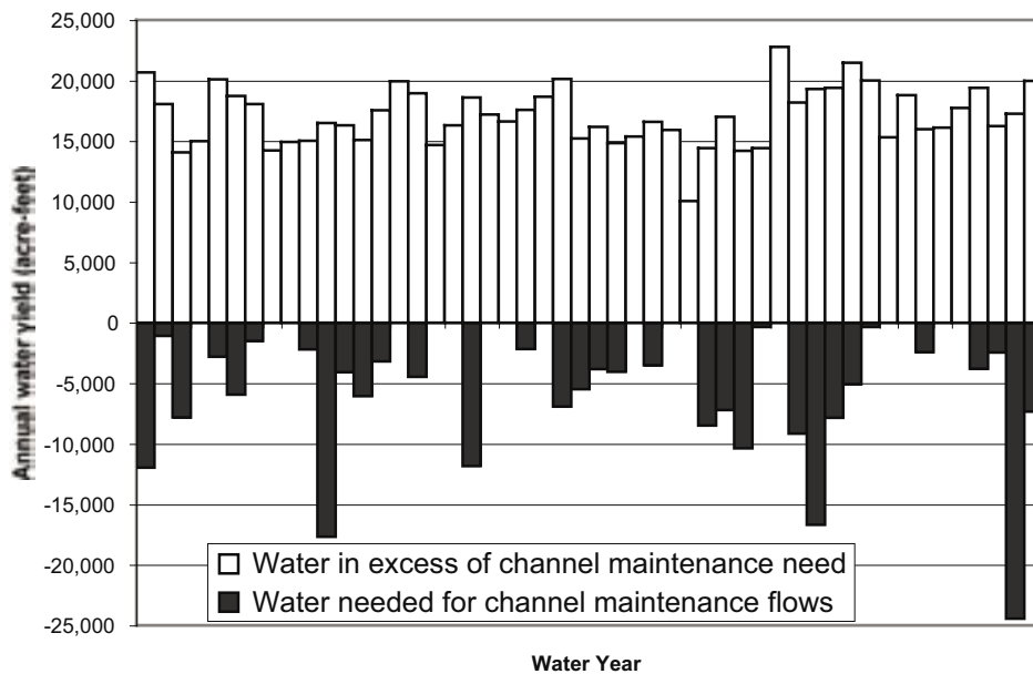
Figure 10 —A display of the long-term partitioning of annual water yield between that needed for channel maintenance and that excess to channel maintenance needs. During some years, no water is needed for channel maintenance while a firm yield of about 15,000 acre-feet of water in excess to channel maintenance needs is annually available except for one drought when water yield is reduced to about 10,000 acre-feet.
