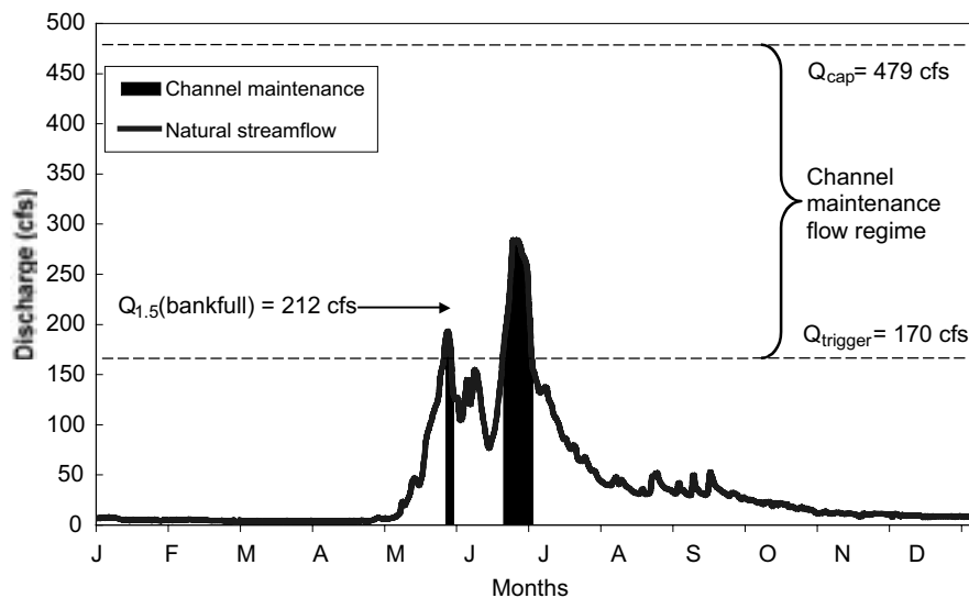
Figure 2b —A typical channel maintenance flow hydrograph applied to a high runoff year (exceeded 20% of years). The discharge data is from Halfmoon Creek, Colorado in 1970. The lower limit ( Q_{\text{trigger}} ) used to initiate the channel maintenance flow regime is 0.8 of the 1.5-year flow and the upper limit ( Q_{\text{cap}} ) is the 25-year flow. For the high runoff year shown, channel maintenance flows require 6,938 acre-feet of water of the 27,070 acre-feet of total natural water yield, or 26% of the annual flow in this year. Most of the channel maintenance work takes place during these high runoff years.
