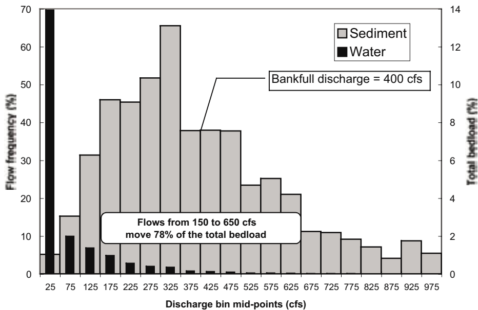
Figure 8 —Example of a sediment magnitude-water frequency histogram. Much (78%) of the total bedload is transported by an intermediate range of flow between 150 and 650 cfs. Extreme high flows and the most frequent low flows tend to move a relatively small percentage of total bedload in the long-term compared to intermediate flows.
