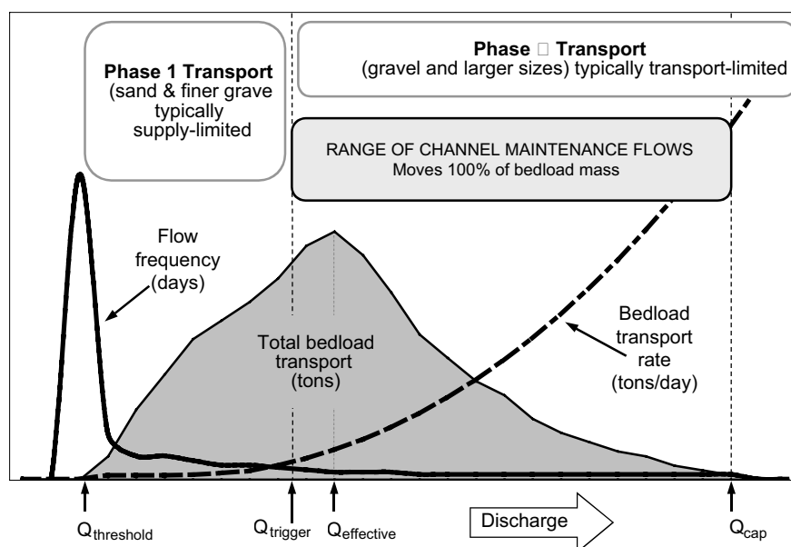
Figure 4 —Schematic of long-term total bedload transport model for gravel-bed rivers based on Wolman and Miller's magnitude-frequency concepts. Bedload movement begins at Q_{\text{threshold}} ; flows between Q_{\text{threshold}} and Q_{\text{trigger}} are Phase 1 transport, Q_{\text{trigger}} is the beginning of Phase 2 transport, flows exceeding Q_{\text{trigger}} are Phase 2 and move the majority of the coarse sizes, and Q_{\text{cap}} is the upper limit of the required channel maintenance flow regime. Flows from Q_{\text{trigger}} to Q_{\text{cap}} constitute the range of flows necessary to maintain the channel.
