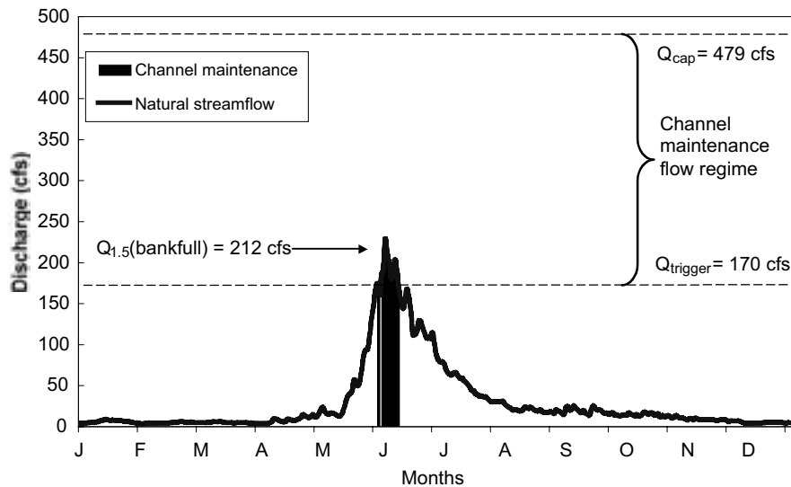
Figure 2a —A typical channel maintenance flow hydrograph applied to an average runoff year (exceeded 50% of years). The discharge data is from Halfmoon Creek, Colorado in 1972. The lower limit ( Q_{\text{trigger}} ) used to initiate the channel maintenance flow regime is 0.8 of the 1.5-year flow and the upper limit ( Q_{\text{cap}} ) is the 25-year flow. For the average year shown, channel maintenance flows require 3,851 acre-feet of water of the 20,023 acre-feet of total natural water yield, or 19% of the annual flow in
