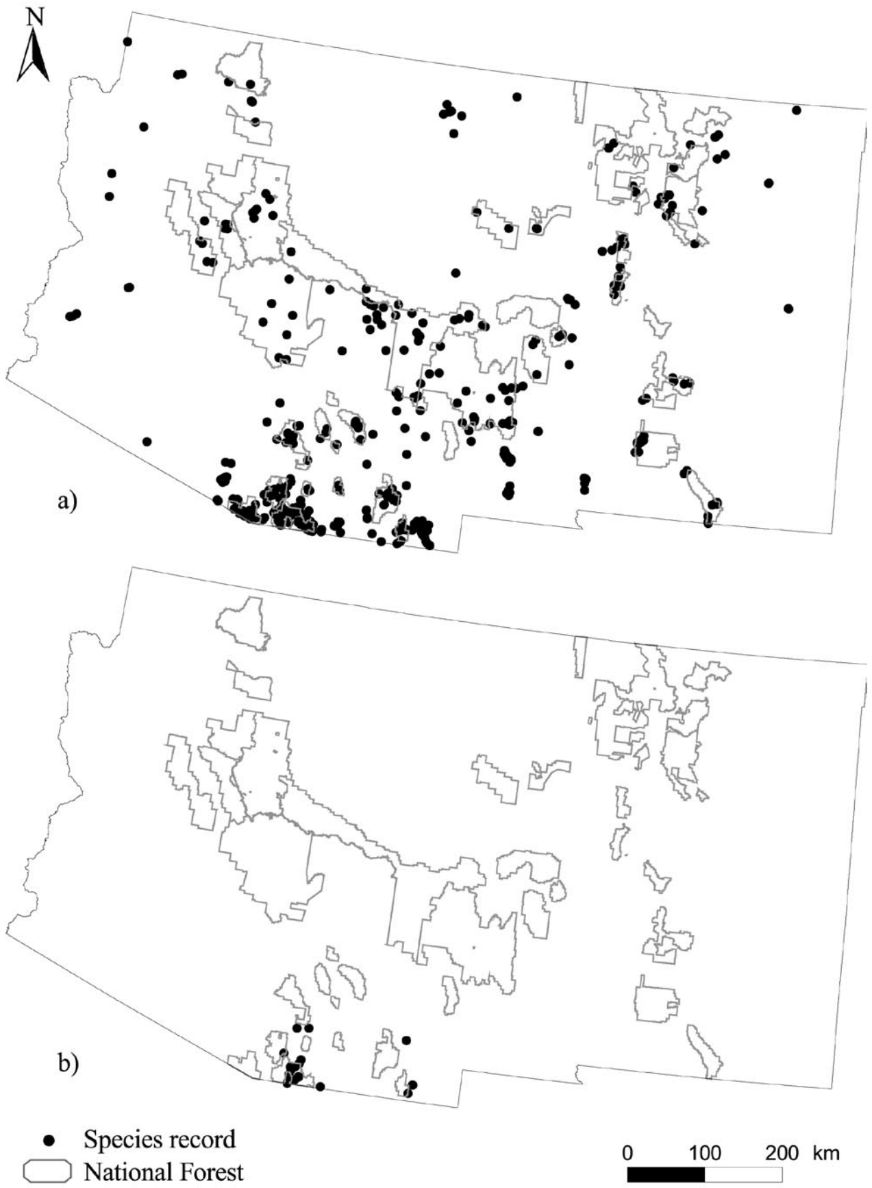
Figure 3 —Point locations for two butterfly species in Arizona and New Mexico: (a) California sister ( Adelpha bredowii ), and (b) sunrise skipper ( Adopaeoides prittwitzi ).
